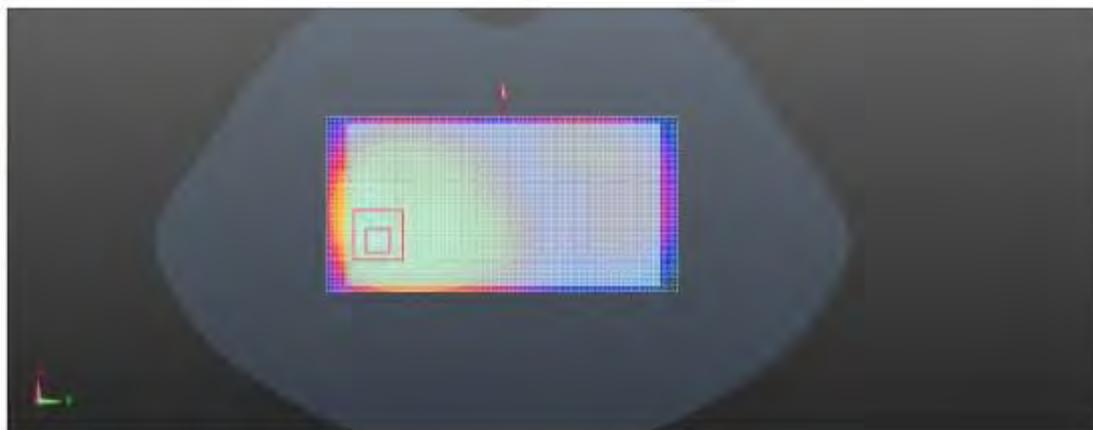
Rear Side (PCS1900 GPRS 4TS Middle Channel)
