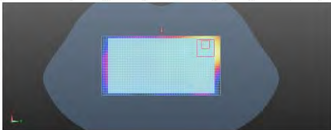
Rear side (WLAN 802.11b Middle Channel)
