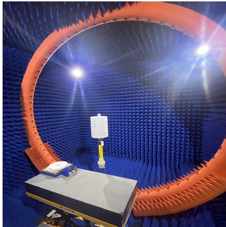
Testing 3D microwave darkroom(6m*6m*6m)
