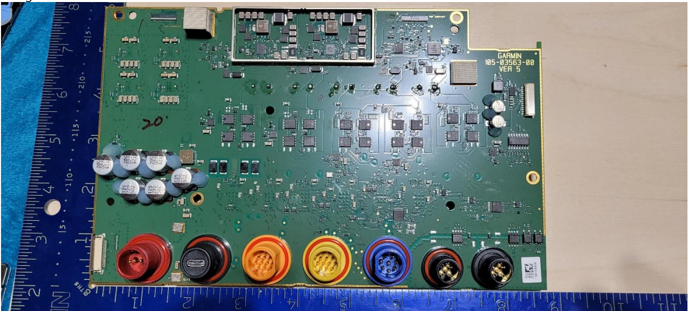
Daughter PCBA
