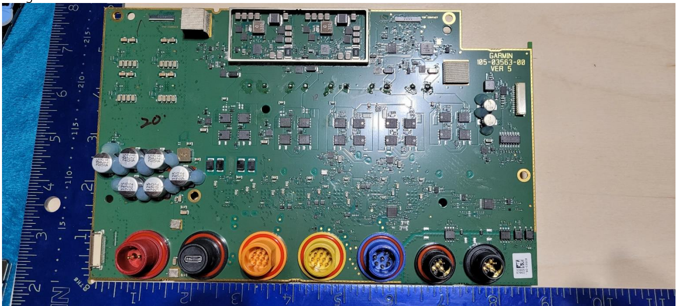
Daughter PCBA
