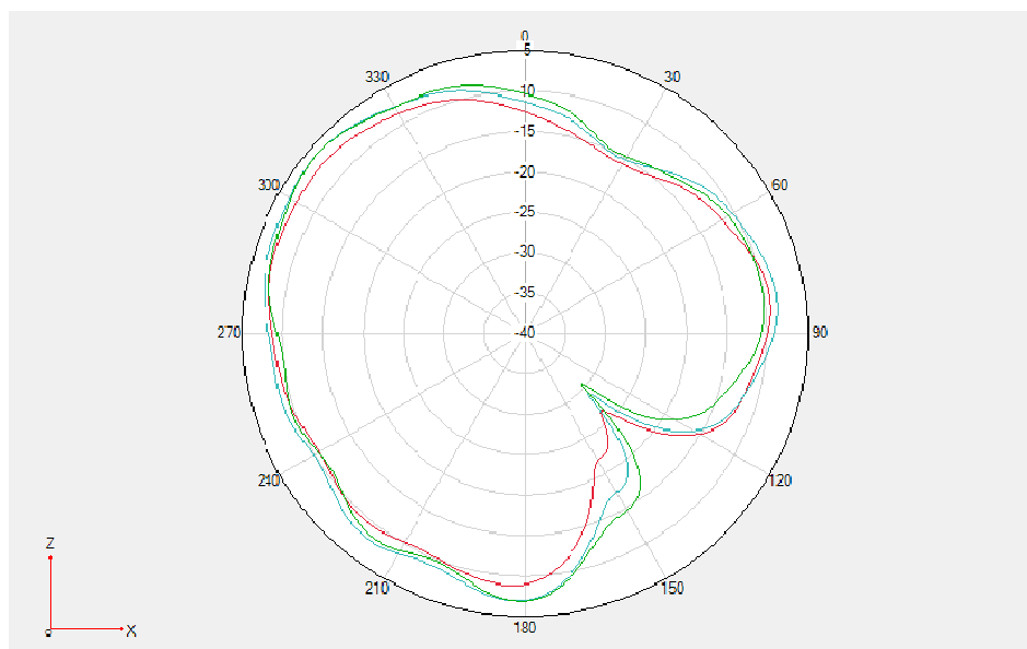
GSM900/WCDMA B8/LTE B8/N8 \Phi=0^\circ
