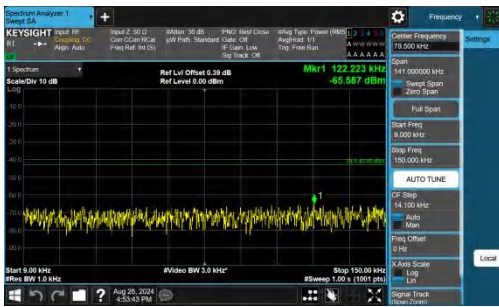
Band25-15MHz-QPSK-26365-1RB#0-0.009~0.15-PASS
