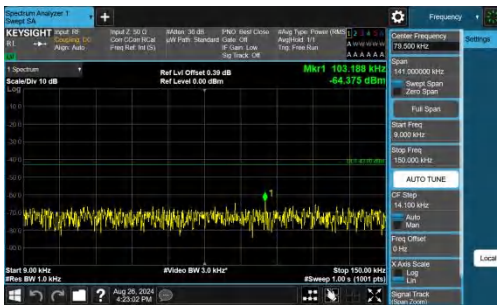
Band25-1.4MHz-QPSK-26683-1RB#0-0.009~0.15-PASS
