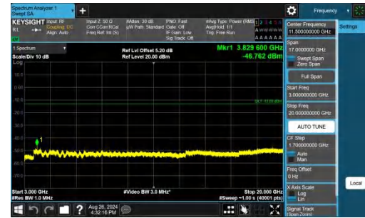
Band25-3MHz-QPSK-26675-1RB#14-3000~20000-PASS
