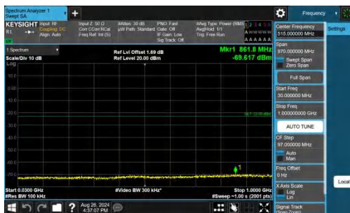
Band25-5MHz-QPSK-26065-1RB#0-30~1000-PASS
