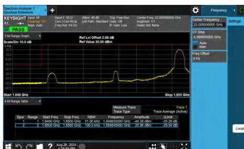
Band25-5MHz-QPSK-26065-1RB#24-PASS
