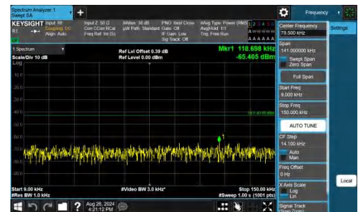
Band25-1.4MHz-QPSK-26047-1RB#5-0.009~0.15-PASS
