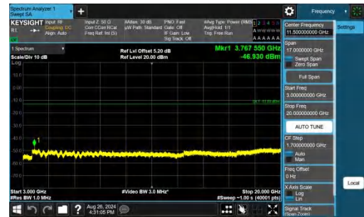
Band25-3MHz-QPSK-26365-1RB#14-3000~20000-PASS
