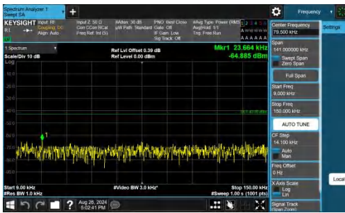
Band25-20MHz-QPSK-26590-1RB#0-0.009~0.15-PASS
