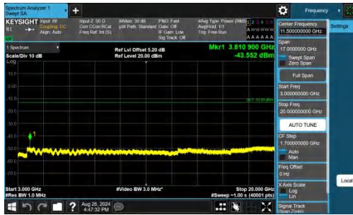
Band25-10MHz-QPSK-26640-1RB#0-3000~20000-PASS
