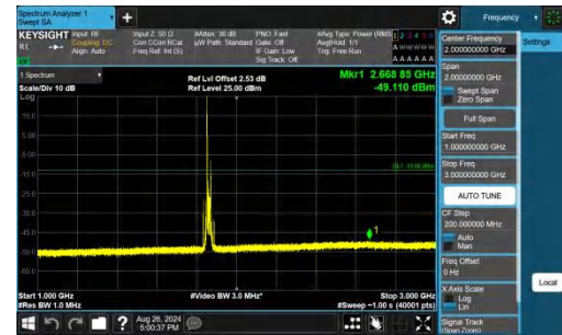
Band25-20MHz-QPSK-26140-1RB#0-1000~3000-PASS
