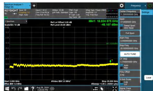
Band25-3MHz-QPSK-26055-1RB#14-3000~20000-PASS
