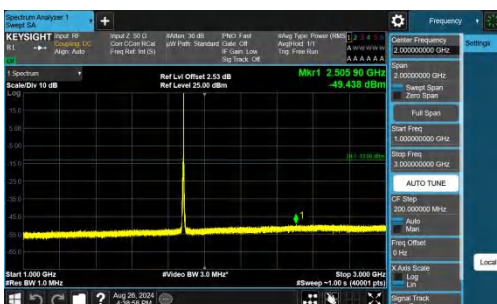
Band25-5MHz-QPSK-26365-1RB#24-1000~3000-PASS
