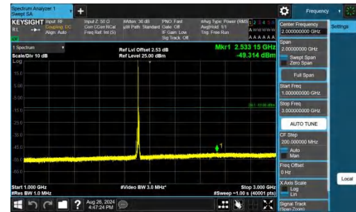
Band25-10MHz-QPSK-26640-1RB#0-1000~3000-PASS
