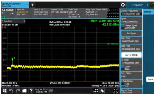
Band25-15MHz-QPSK-26615-1RB#0-3000~20000-PASS
