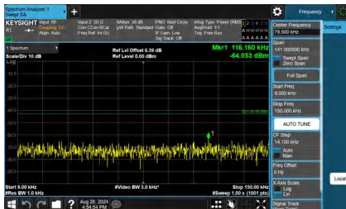
Band25-15MHz-QPSK-26615-1RB#0-0.009~0.15-PASS
