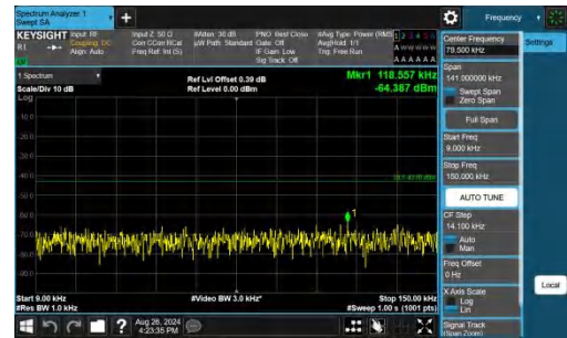
Band25-1.4MHz-QPSK-26683-1RB#5-0.009~0.15-PASS
