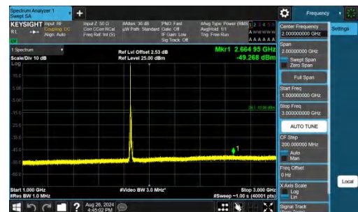
Band25-10MHz-QPSK-26090-1RB#0-1000~3000-PASS
