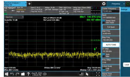
Band25-5MHz-QPSK-26365-1RB#24-0.009~0.15-PASS
