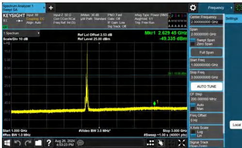
Band25-15MHz-QPSK-26115-1RB#74-1000~3000-PASS
