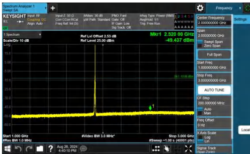
Band25-5MHz-QPSK-26665-1RB#24-1000~3000-PASS
