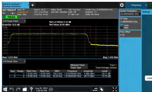
Band25-3MHz-QPSK-26675-15RB#0-PASS
