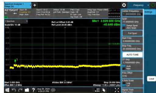
Band25-1.4MHz-QPSK-26683-1RB#5-3000~20000-PASS
