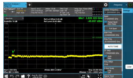
Band25-15MHz-QPSK-26615-1RB#74-3000~20000-PASS
