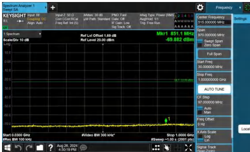
Band25-3MHz-QPSK-26365-1RB#0-30~1000-PASS
