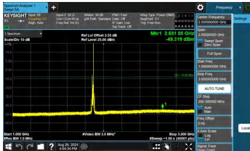
Band25-15MHz-QPSK-26365-1RB#74-1000~3000-PASS
