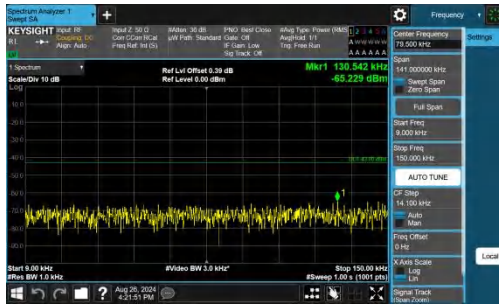
Band25-1.4MHz-QPSK-26365-1RB#0-0.009~0.15-PASS
