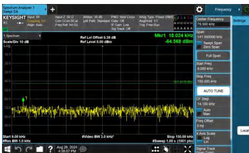
Band25-5MHz-QPSK-26365-1RB#0-0.009~0.15-PASS
