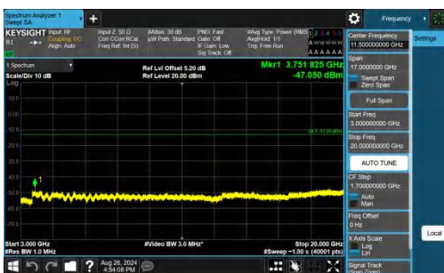
Band25-15MHz-QPSK-26365-1RB#0-3000~20000-PASS
