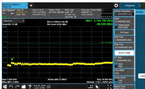
Band25-1.4MHz-QPSK-26365-1RB#0-3000~20000-PASS
