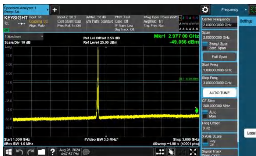
Band25-10MHz-QPSK-26640-1RB#49-1000~3000-PASS
