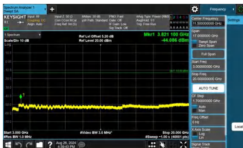
Band25-5MHz-QPSK-26665-1RB#0-3000~20000-PASS
