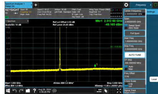
Band25-5MHz-QPSK-26365-1RB#0-1000~3000-PASS
