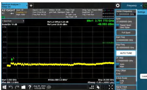
Band25-20MHz-QPSK-26590-1RB#0-3000~20000-PASS
