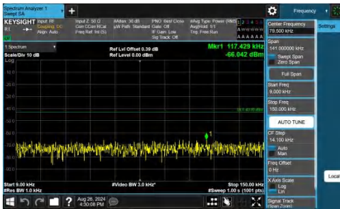
Band25-3MHz-QPSK-26365-1RB#0-0.009~0.15-PASS
