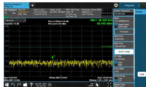
Band25-3MHz-QPSK-26675-1RB#14-0.009~0.15-PASS
