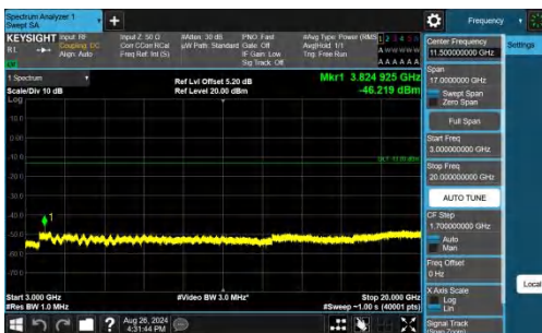
Band25-3MHz-QPSK-26675-1RB#0-3000~20000-PASS
