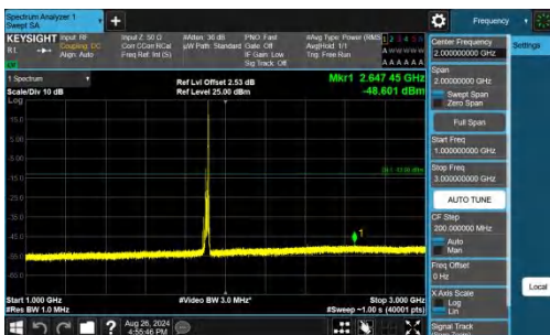
Band25-15MHz-QPSK-26615-1RB#74-1000~3000-PASS
