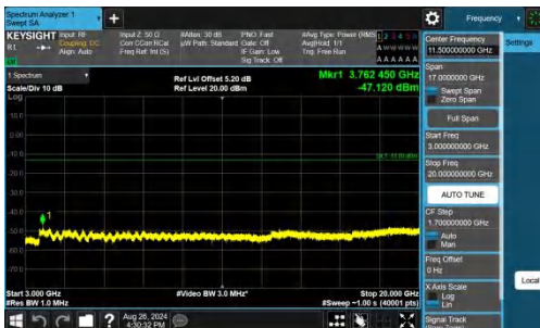
Band25-3MHz-QPSK-26365-1RB#0-3000~20000-PASS
