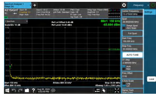
Band25-15MHz-QPSK-26365-1RB#0-0.15~30-PASS
