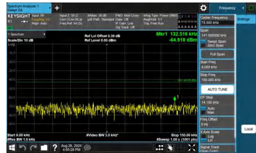
Band25-15MHz-QPSK-26615-1RB#74-0.009~0.15-PASS
