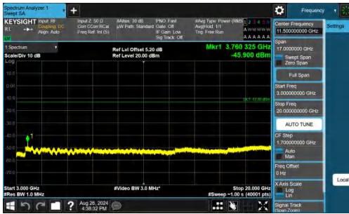
Band25-5MHz-QPSK-26365-1RB#0-3000~20000-PASS
