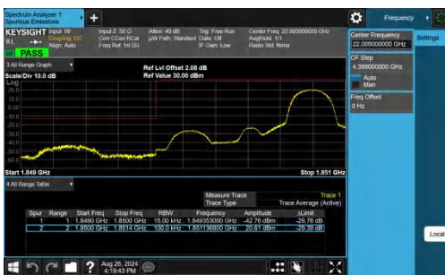
Band25-1.4MHz-QPSK-26047-1RB#5-PASS
