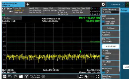
Band25-5MHz-QPSK-26065-1RB#0-0.009~0.15-PASS
