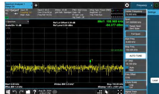
Band25-3MHz-QPSK-26365-1RB#14-0.009~0.15-PASS
