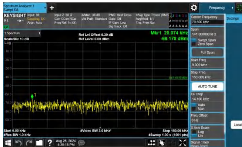
Band25-5MHz-QPSK-26665-1RB#0-0.009~0.15-PASS
