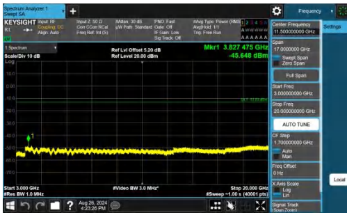
Band25-1.4MHz-QPSK-26683-1RB#0-3000~20000-PASS
