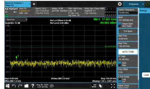
Band25-5MHz-QPSK-26065-1RB#24-0.009~0.15-PASS
