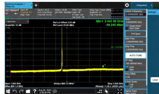
Band25-5MHz-QPSK-26665-1RB#0-1000~3000-PASS
