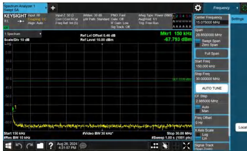
Band25-3MHz-QPSK-26675-1RB#14-0.15~30-PASS
