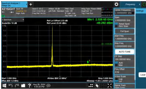
Band25-10MHz-QPSK-26090-1RB#49-1000~3000-PASS
