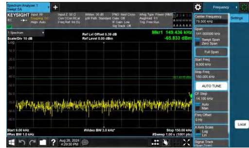
Band25-3MHz-QPSK-26055-1RB#14-0.009~0.15-PASS
