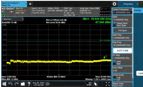
Band25-5MHz-QPSK-26065-1RB#0-3000~20000-PASS
