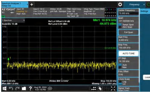
Band25-3MHz-QPSK-26675-1RB#0-0.009~0.15-PASS
