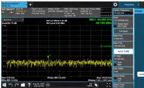
Band25-15MHz-QPSK-26115-1RB#0-0.009~0.15-PASS
