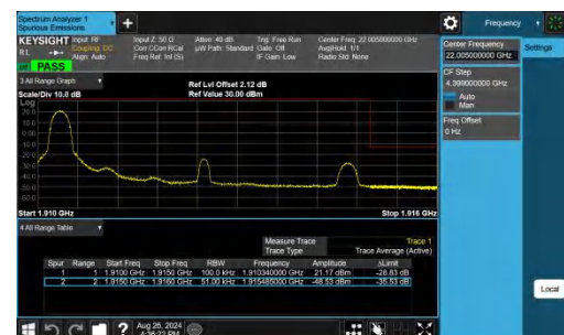
Band25-5MHz-QPSK-26665-1RB#0-PASS
