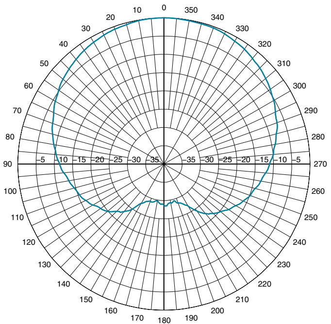
WISP4959018MBV - 90° Azimuth Cut
