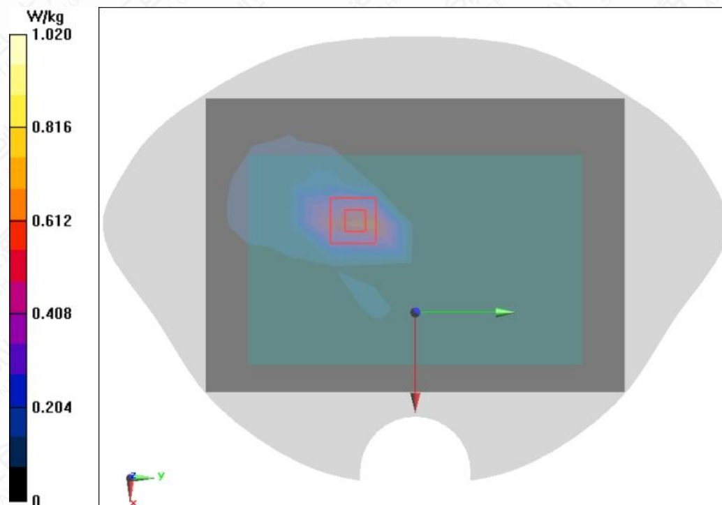
Figure A.1-2 Wi-Fi 5G 802.11ac20 Left Side-2 Mode Low 0mm
