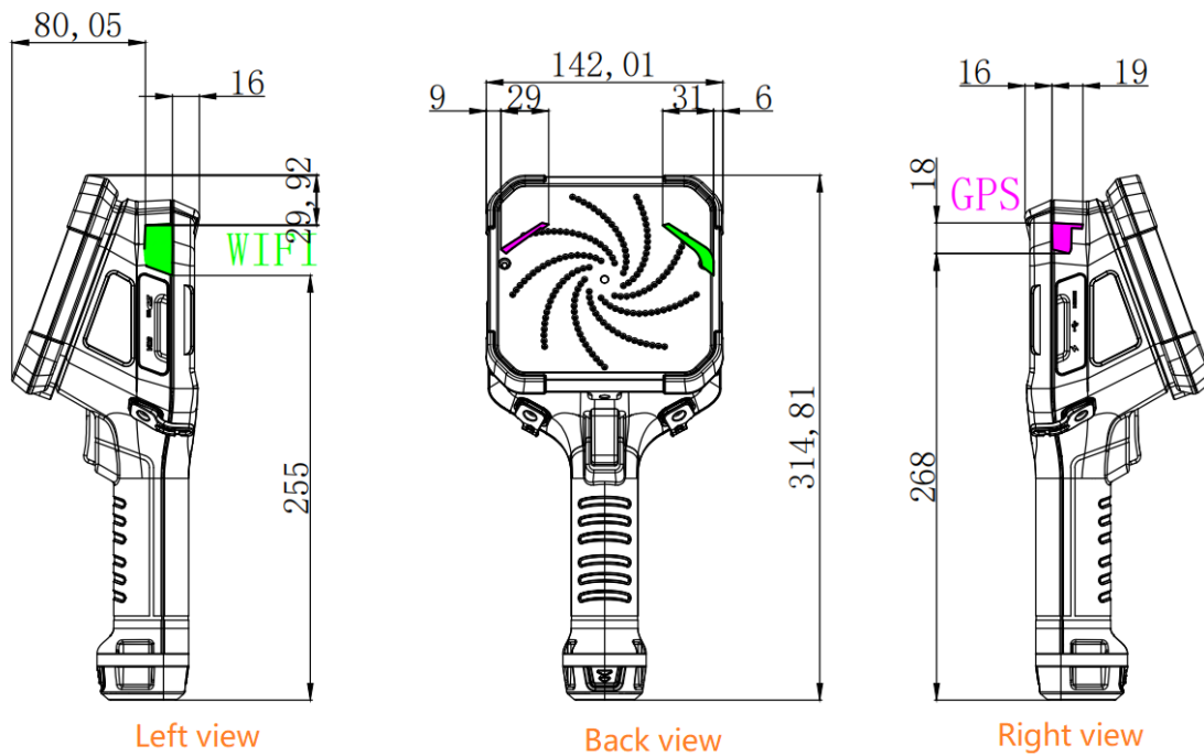
Figure 12.2-1 Antenna Locations
