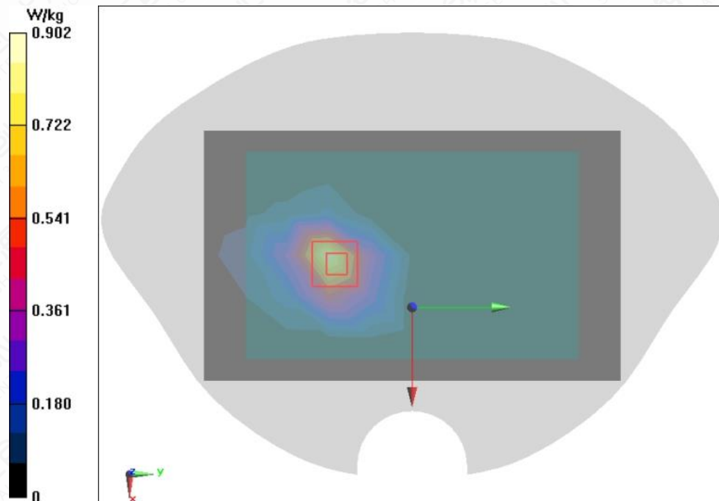
Figure A.1-5 Wi-Fi 5G 802.11n20 Top Side Mode Middle 0mm
