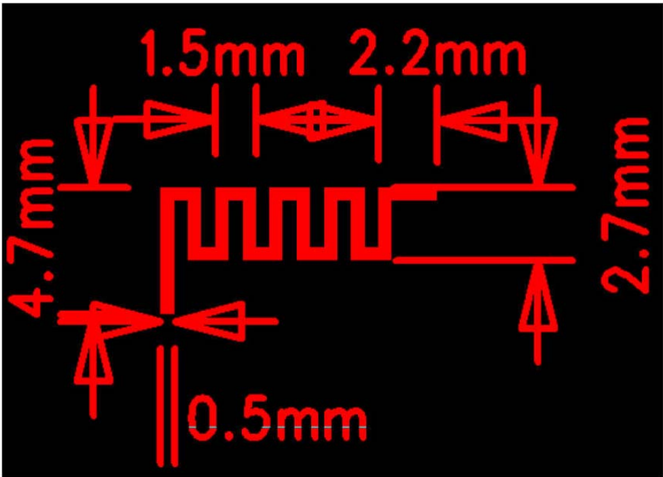
Antenna Photo & Length (mm)
