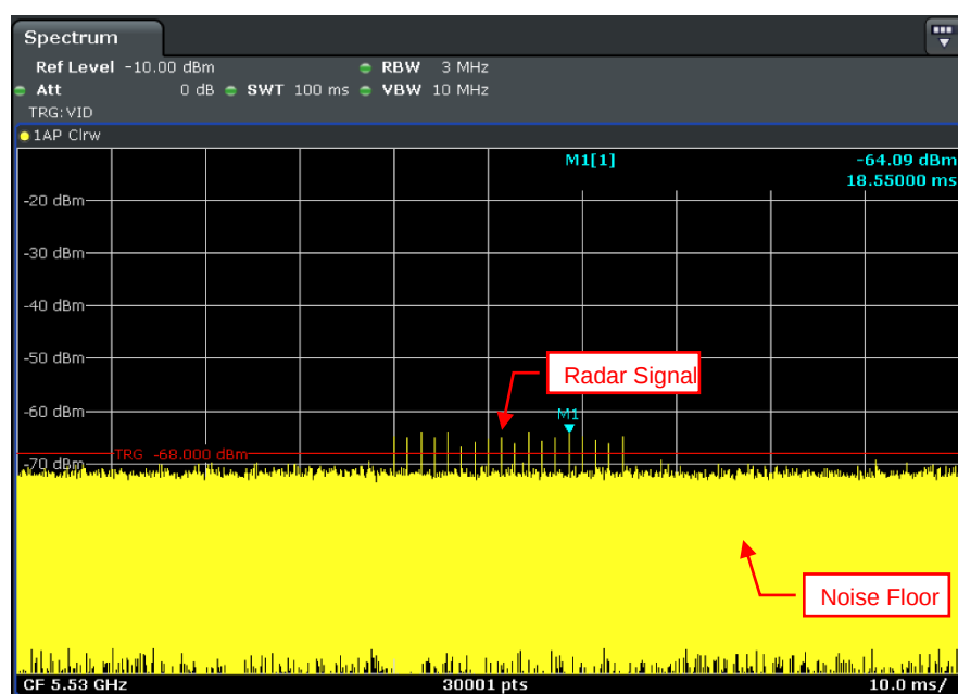
Radar Signal 0
