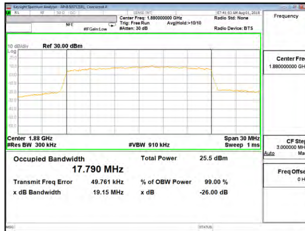
LTE B2 20MHz 64QAM Mid Channel RB100-0
