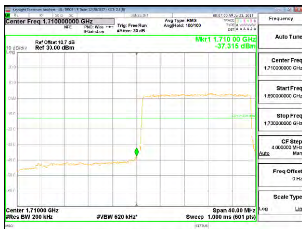
LTE B4 20MHz 16QAM Low Channel RB100-0
