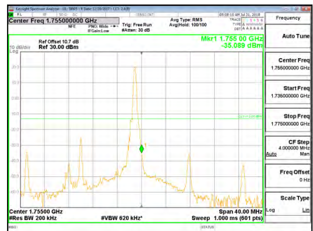
LTE B4 20MHz 16QAM High Channel RB1-0
