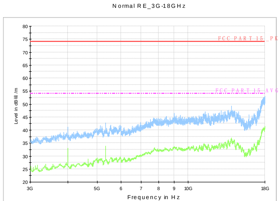
Fig.A.6.2.6 Radiated Spurious Emission (802.11b, Ch6, 3 GHz-18 GHz)
