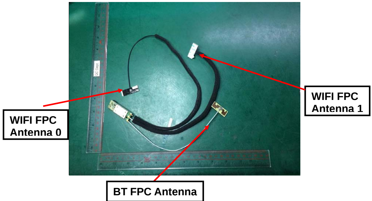
Photo 2 Appearance of FPC Antenna
