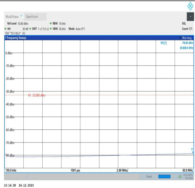
2-2-15MHz-15MHz-QPSK-QPSK-18825-18975-1RB#0-1RB#7 4-0.15~30MHz-PASS
