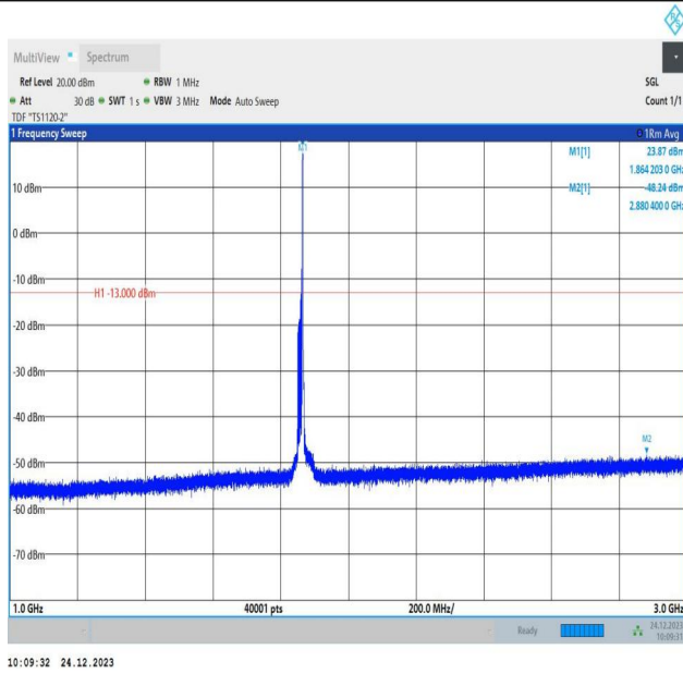
2-2-15MHz-15MHz-QPSK-QPSK-18675-18825-1RB#74-0RB# 0-1000~3000MHz-PASS
