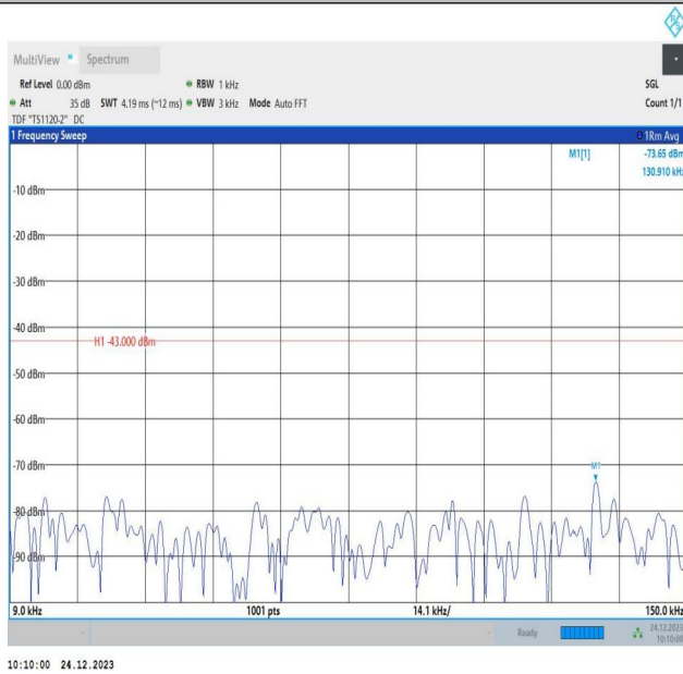
2-2-15MHz-15MHz-QPSK-QPSK-18675-18825-1RB#0-1RB#7 4-0.009~0.15MHz-PASS
