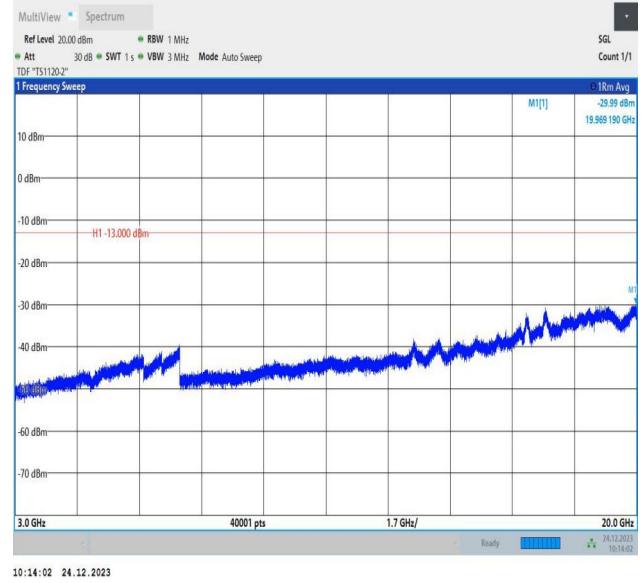
2-2-15MHz-15MHz-QPSK-QPSK-18825-18975-1RB#74-0RB# 0-3000~20000MHz-PASS
