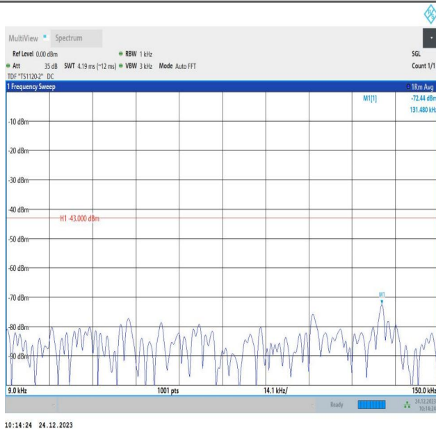
2-2-15MHz-15MHz-QPSK-QPSK-18825-18975-1RB#0-1RB#7 4-0.009~0.15MHz-PASS
