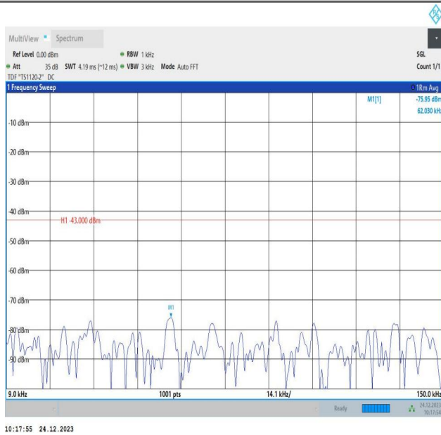
2-2-15MHz-15MHz-QPSK-QPSK-18975-19125-1RB#0-1RB#7 4-0.009~0.15MHz-PASS
