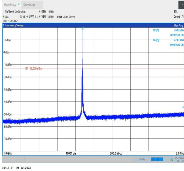
2-2-15MHz-15MHz-QPSK-QPSK-18825-18975-1RB#74-0RB# 0-1000~3000MHz-PASS
