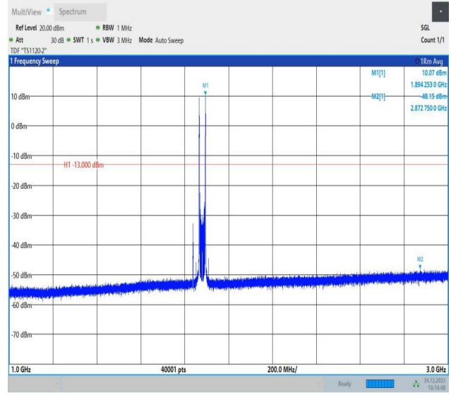
2-2-15MHz-15MHz-QPSK-QPSK-18825-18975-1RB#0-1RB#7 4-1000~3000MHz-PASS
