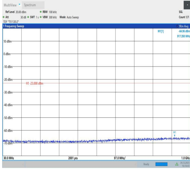
2-2-15MHz-15MHz-QPSK-QPSK-18825-18975-1RB#0-1RB#7 4-30~1000MHz-PASS
