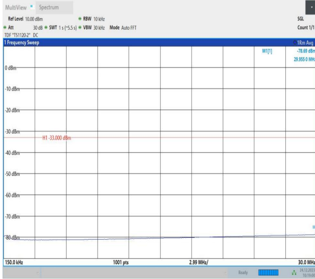
2-2-15MHz-15MHz-QPSK-QPSK-18975-19125-75RB#0-75RB #0-0.15~30MHz-PASS
