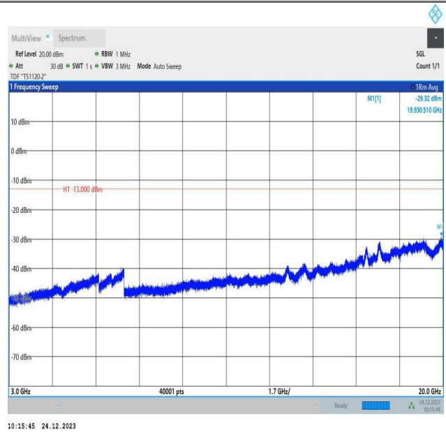
2-2-15MHz-15MHz-QPSK-QPSK-18825-18975-75RB#0-75RB #0-3000~20000MHz-PASS
