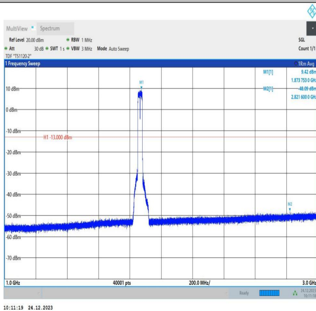
2-2-15MHz-15MHz-QPSK-QPSK-18675-18825-75RB#0-75RB #0-1000~3000MHz-PASS
