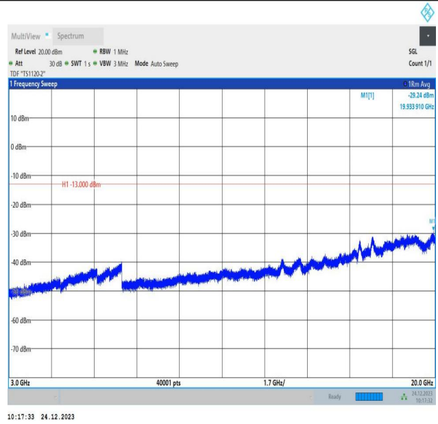
2-2-15MHz-15MHz-QPSK-QPSK-18975-19125-1RB#74-0RB# 0-3000~20000MHz-PASS
