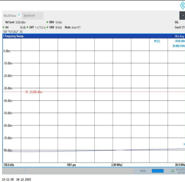
2-2-15MHz-15MHz-QPSK-QPSK-18675-18825-75RB#0-75RB #0-0.15~30MHz-PASS
