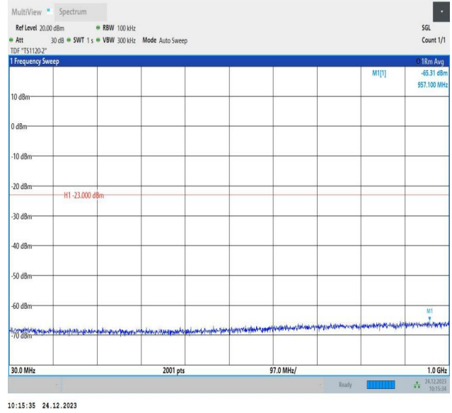
2-2-15MHz-15MHz-QPSK-QPSK-18825-18975-75RB#0-75RB #0-30~1000MHz-PASS
