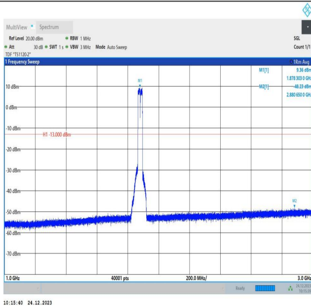
2-2-15MHz-15MHz-QPSK-QPSK-18825-18975-75RB#0-75RB #0-1000~3000MHz-PASS
