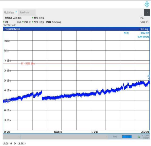
2-2-15MHz-15MHz-QPSK-QPSK-18675-18825-1RB#74-0RB# 0-3000~20000MHz-PASS
