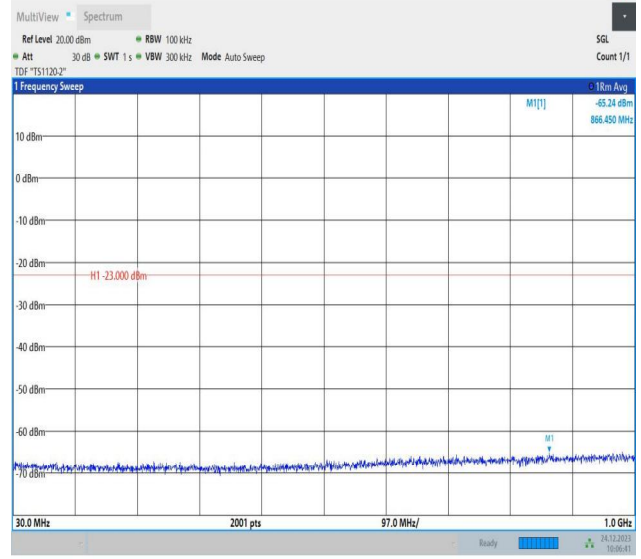
2-2-15MHz-10MHz-QPSK-QPSK-19027-19147-75RB#0-50RB #0-30~1000MHz-PASS
