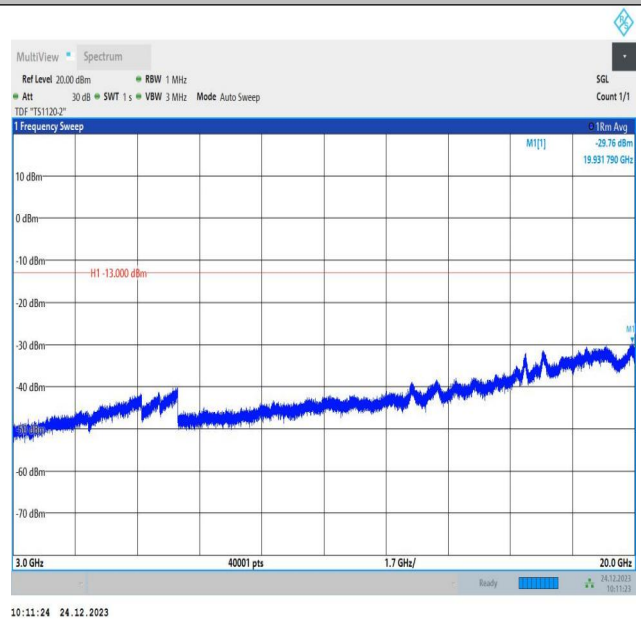
2-2-15MHz-15MHz-QPSK-QPSK-18675-18825-75RB#0-75RB #0-3000~20000MHz-PASS
