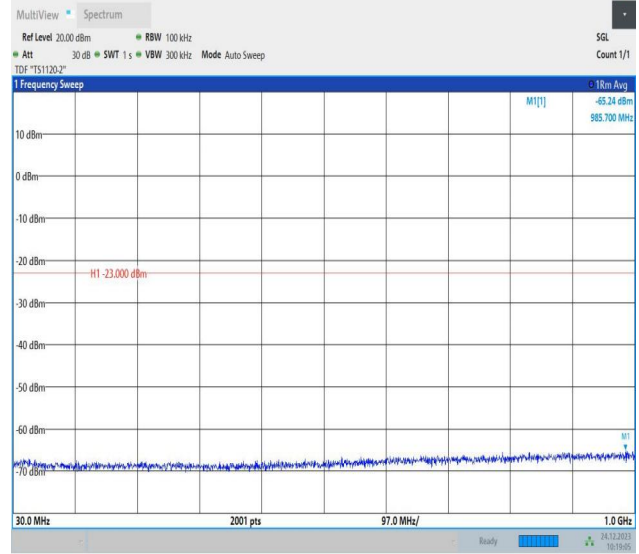
2-2-15MHz-15MHz-QPSK-QPSK-18975-19125-75RB#0-75RB #0-30~1000MHz-PASS
