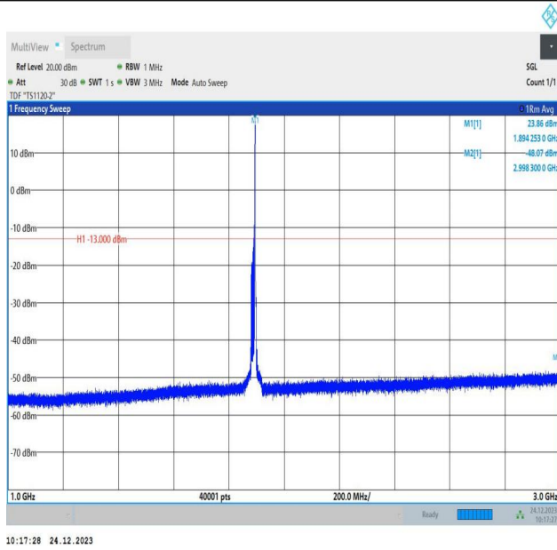
2-2-15MHz-15MHz-QPSK-QPSK-18975-19125-1RB#74-0RB# 0-1000~3000MHz-PASS
