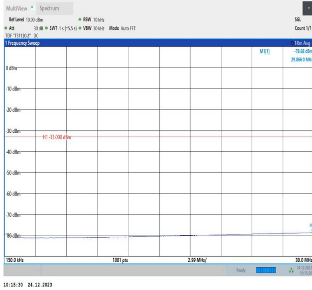
2-2-15MHz-15MHz-QPSK-QPSK-18825-18975-75RB#0-75RB #0-0.15~30MHz-PASS
