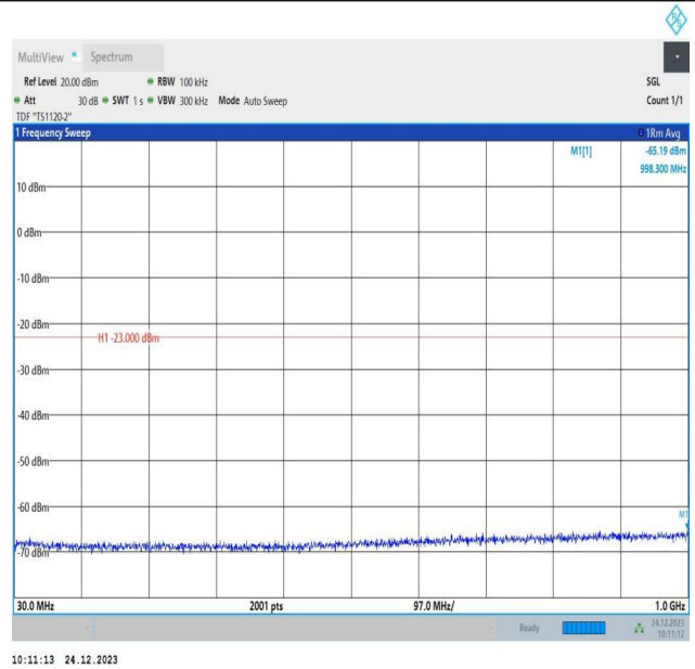
2-2-15MHz-15MHz-QPSK-QPSK-18675-18825-75RB#0-75RB #0-30~1000MHz-PASS
