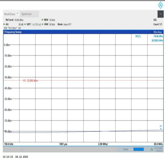
2-2-15MHz-15MHz-QPSK-QPSK-18675-18825-1RB#0-1RB#7 4-0.15~30MHz-PASS
