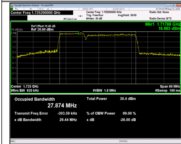
66-66-10MHz-20MHz-64QAM-64QAM-132027-132171-50RB #0-100RB#0-PASS
