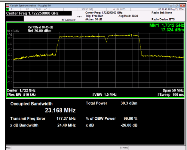
66-66-15MHz-10MHz-64QAM-64QAM-132047-132167-75RB RB#0-50RB#0-PASS
