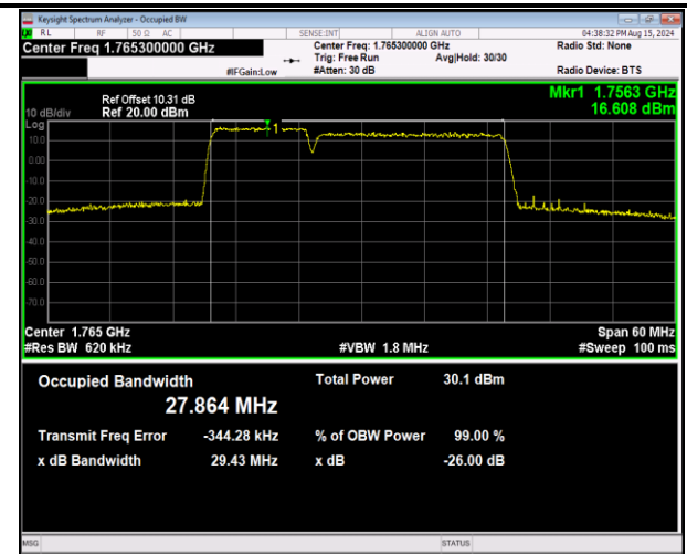
66-66-10MHz-20MHz-16QAM-16QAM-132428-132572-50RB #0-100RB#0-PASS
