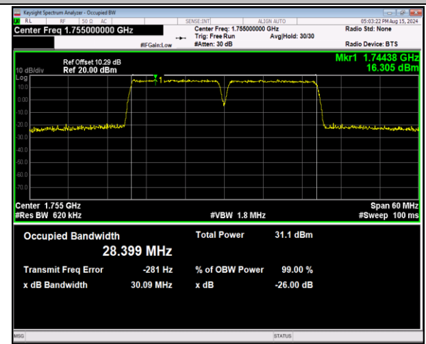
66-66-15MHz-15MHz-QPSK-QPSK-132347-132497-75RB #0-75RB#0-PASS
