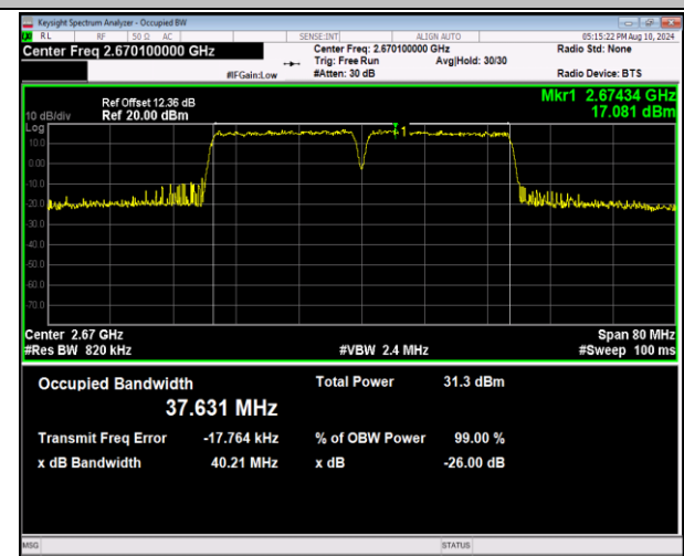
41-41-20MHz-20MHz-QPSK-QPSK-41292-41490-100RB#0-100RB#0-PASS
