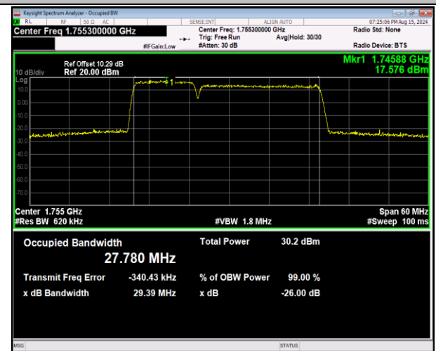
66-66-10MHz-20MHz-64QAM-64QAM-132328-132472-50RB #0-100RB#0-PASS
