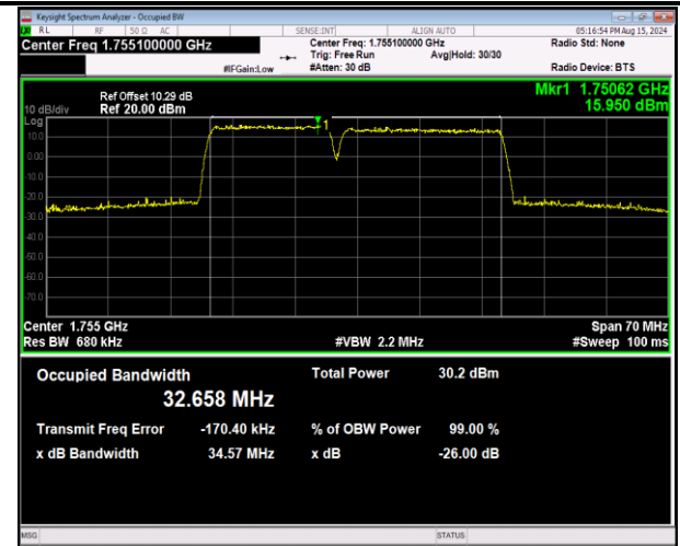
66-66-15MHz-20MHz-16QAM-16QAM-132325-132496-75RB #0-100RB#0-PASS
