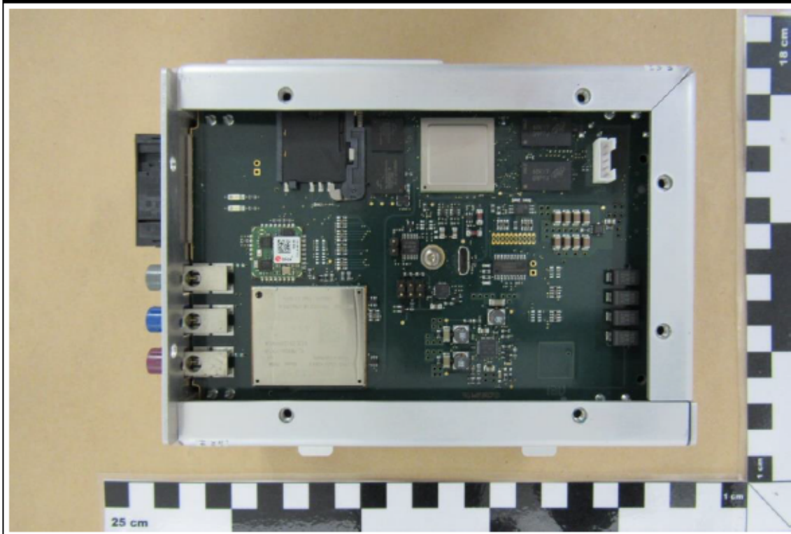
VIEW (A)
