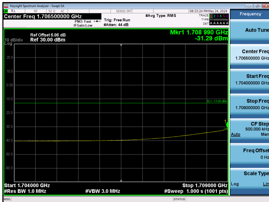
LTE Band 66 / 3MHz / 16QAM - RB Size/Offset (8/4)
