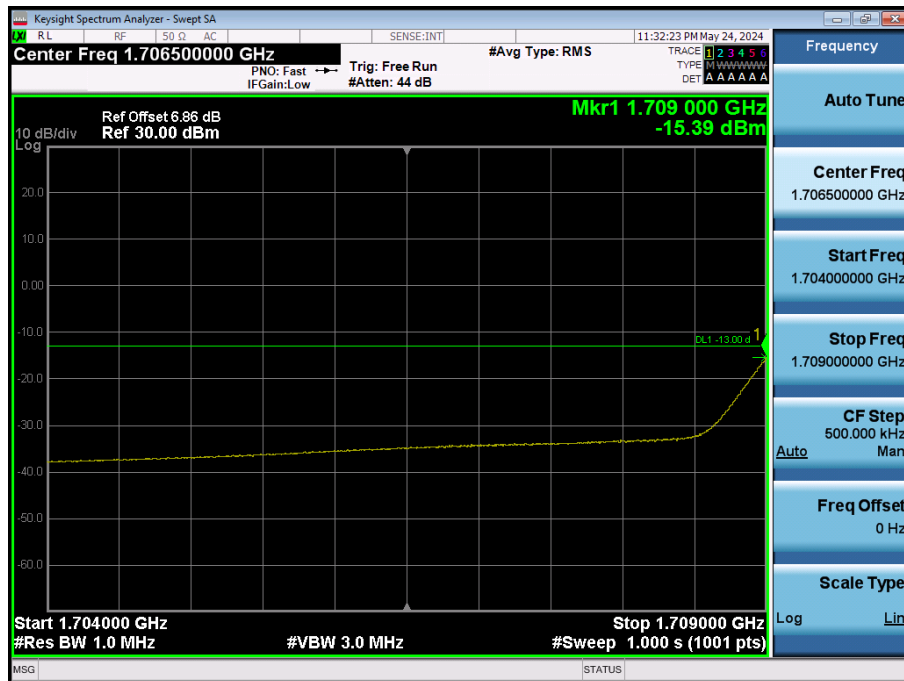
LTE Band 66 / 5MHz / 64QAM - RB Size/Offset (25/0)
