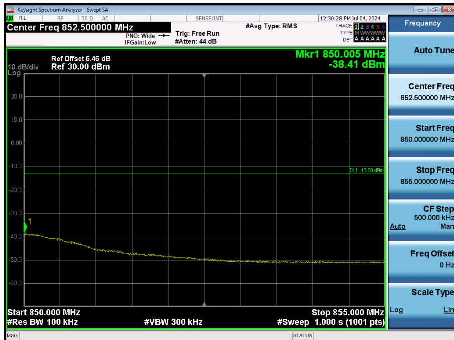
LTE Band 5 / 5MHz / 256QAM - RB Size/Offset (12/13)
