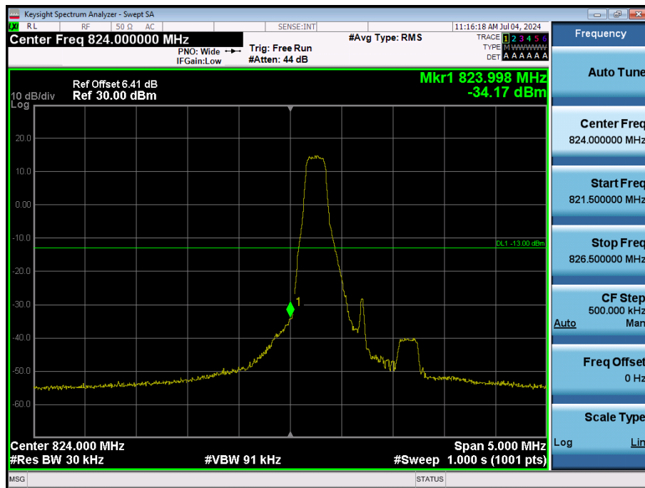
LTE Band 5 / 1.4MHz / 64QAM - RB Size/Offset (1/0)
