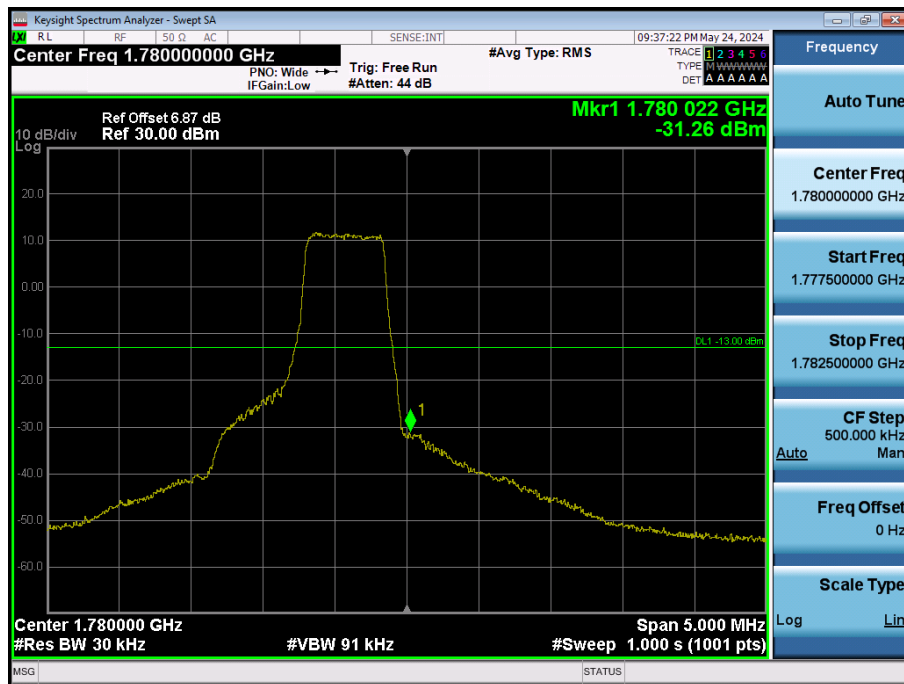
LTE Band 66 / 1.4MHz / 16QAM - RB Size/Offset (3/3)
