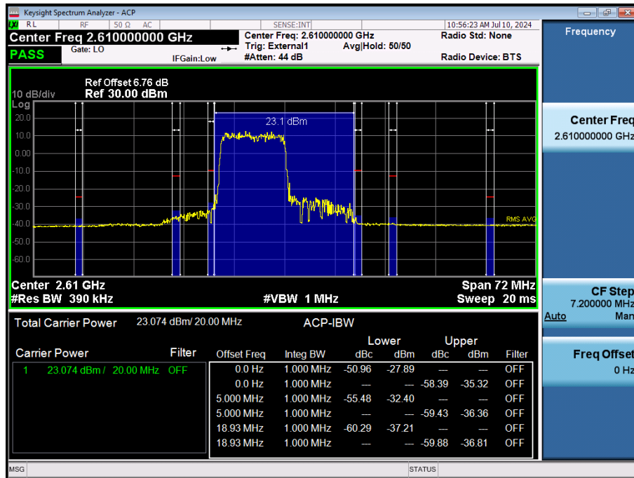
LTE Band 38 / 20Hz / QPSK - RB Size/Offset (50/0)
