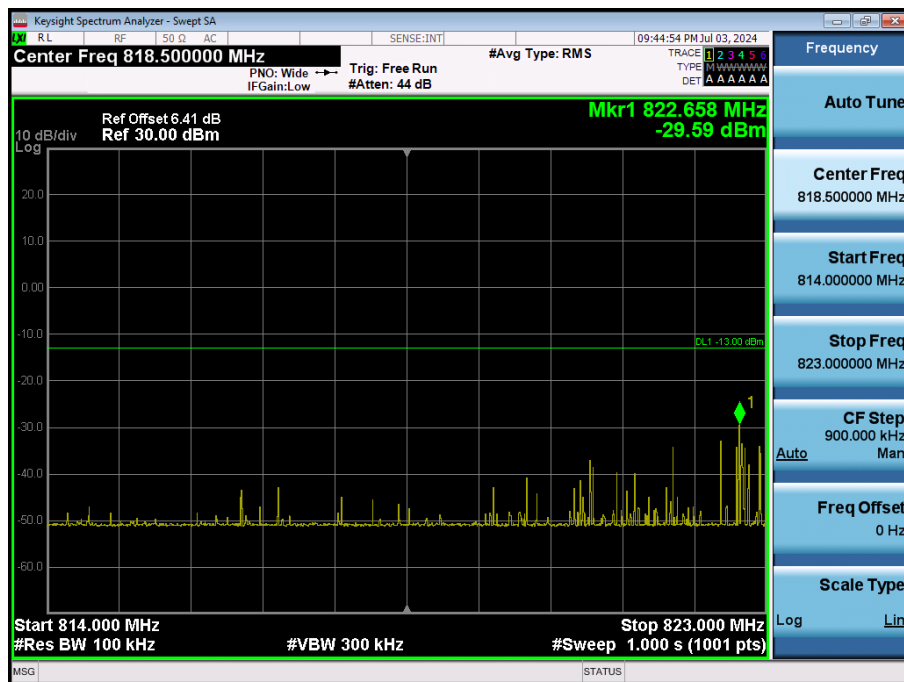
LTE Band 5 / 10MHz / QPSK - RB Size/Offset (1/25)
