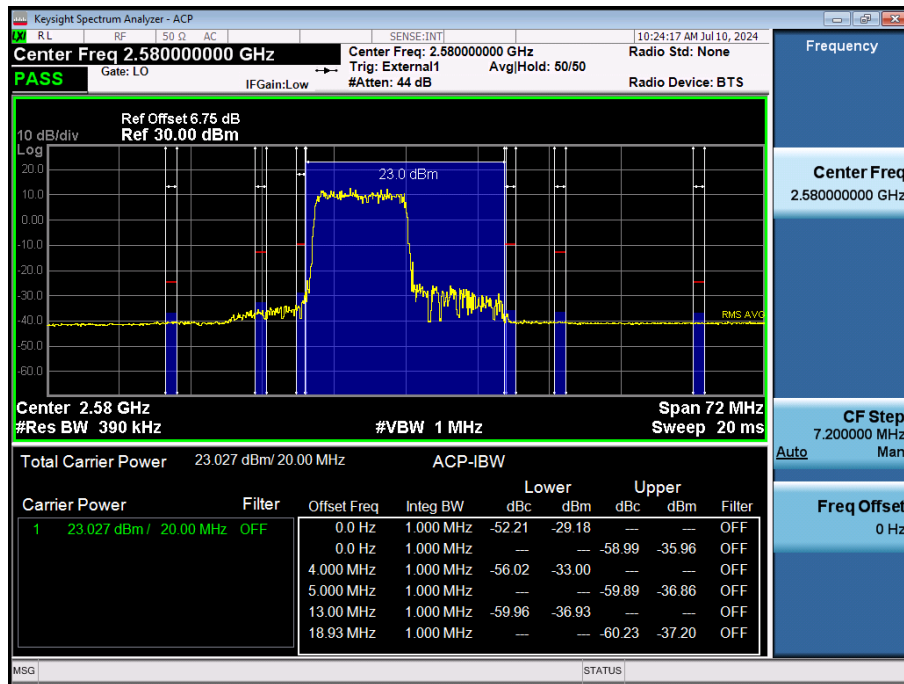
LTE Band 38 / 20MHz / QPSK - RB Size/Offset (50/0)
