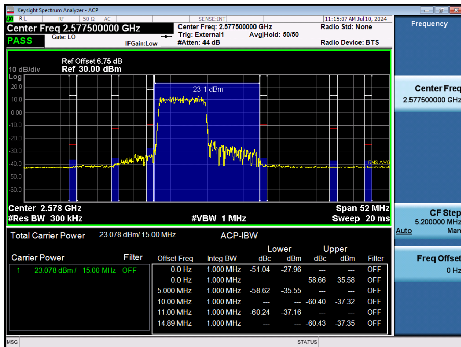
LTE Band 38 / 15MHz / QPSK - RB Size/Offset (36/0)
