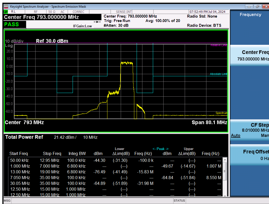
LTE Band 14 / 10MHz / QPSK - RB Size/Offset (25/25)
