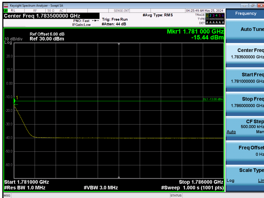
LTE Band 66 / 1.4MHz / 256QAM - RB Size/Offset (1/2)
