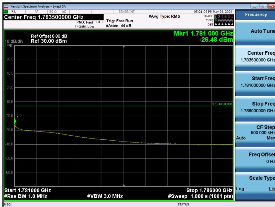
LTE Band 66 / 3MHz / QPSK - RB Size/Offset (8/4)
