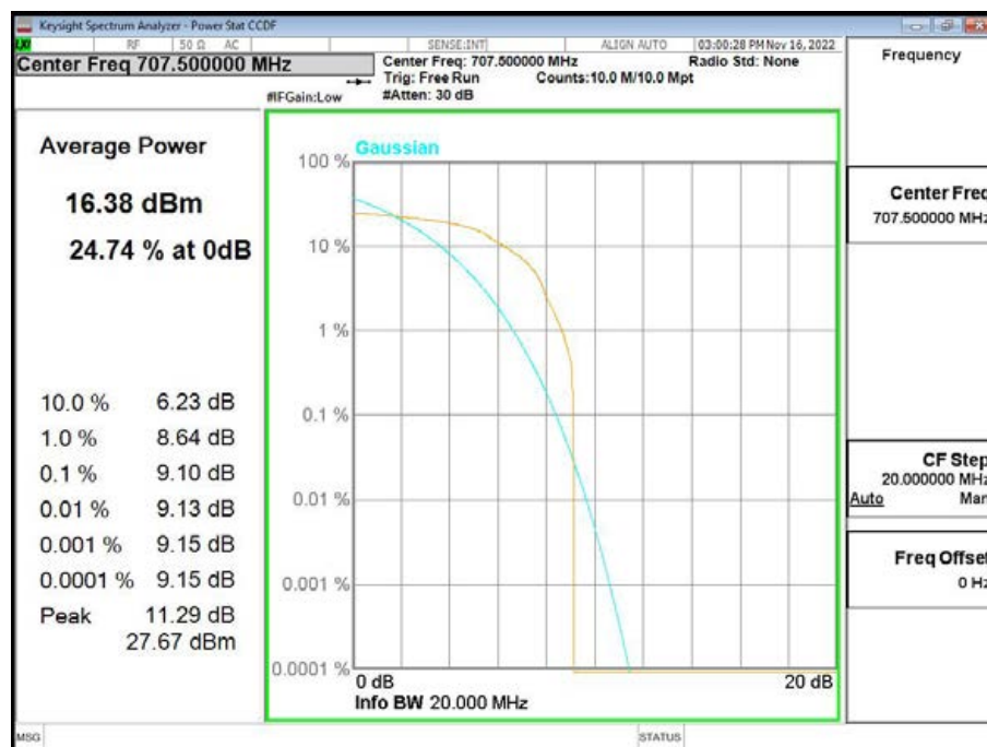
Band12-CH23095-707.5MHz-5MHz Bandwidth-16QAM
