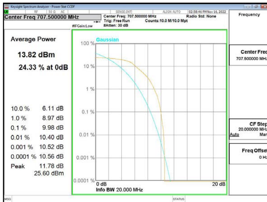
Band12-CH23095-707.5MHz-3MHz Bandwidth-QPSK
