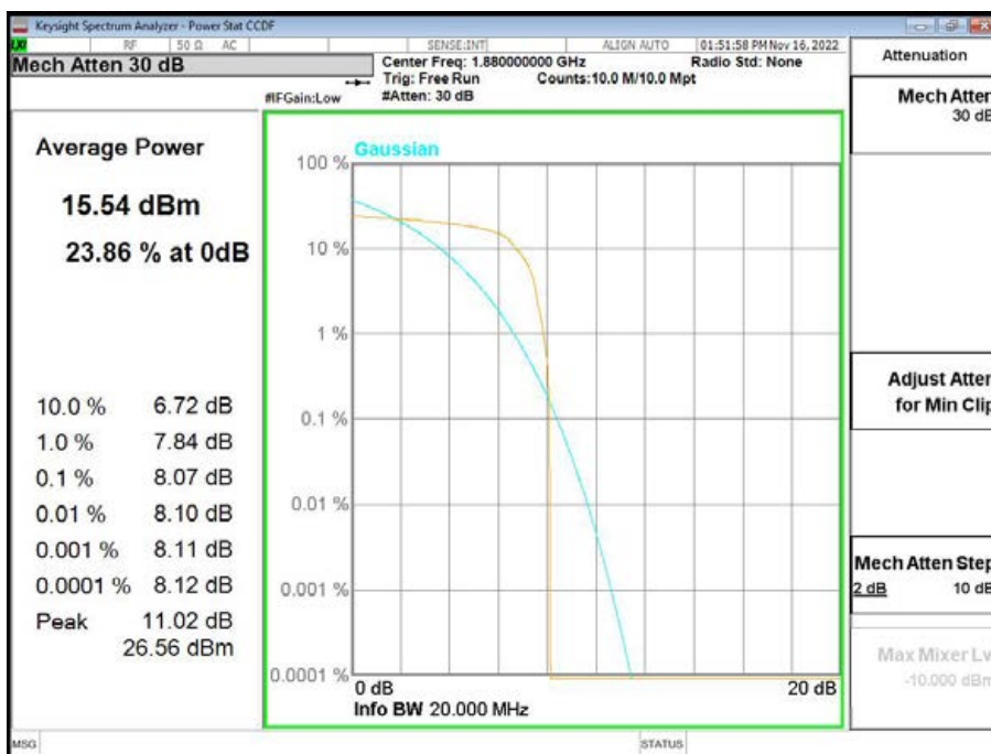
Band2-CH18900-1880MHz-15MHz Bandwidth-16QAM
