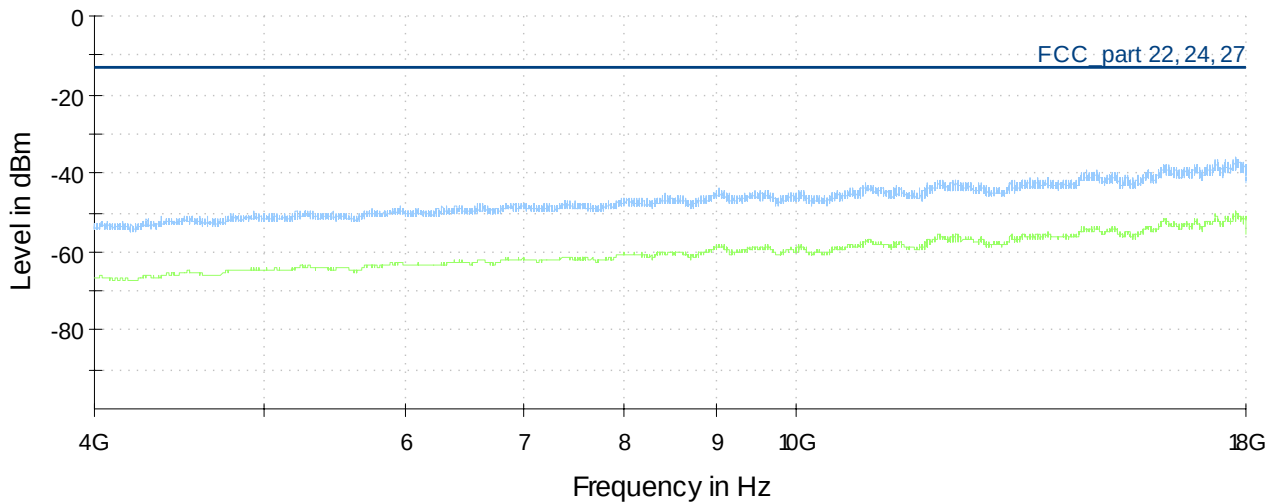
Results 4 to 18 GHz
