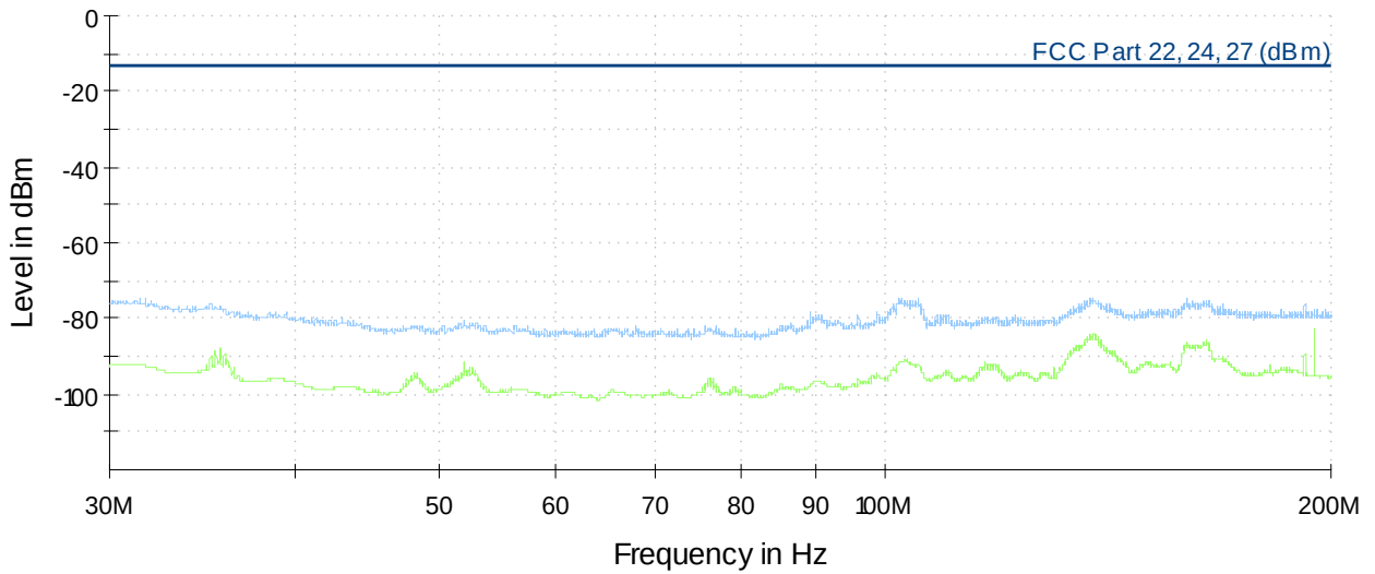
Results 30 MHz to 200 MHz
