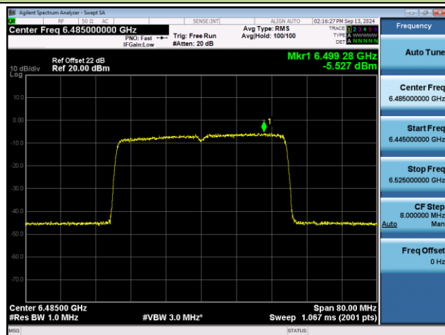
Channel 107 (6485MHz)
