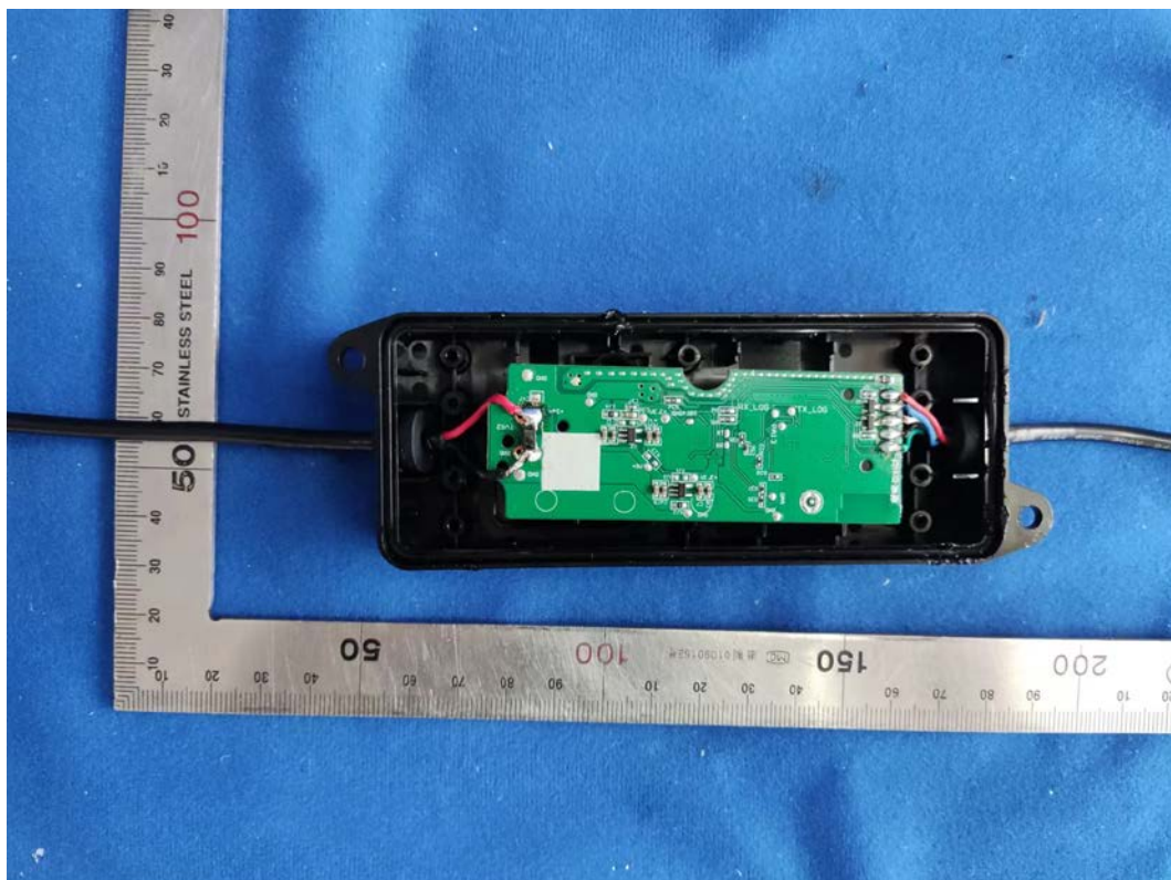
FIGURE 6 CYNC DIRECT CONNECTED OUTDOOR PREMIUM LIGHT STRIP (16FT.) (M/N: CLEDSTR36SCDODP) MAIN BORAD FRONT
