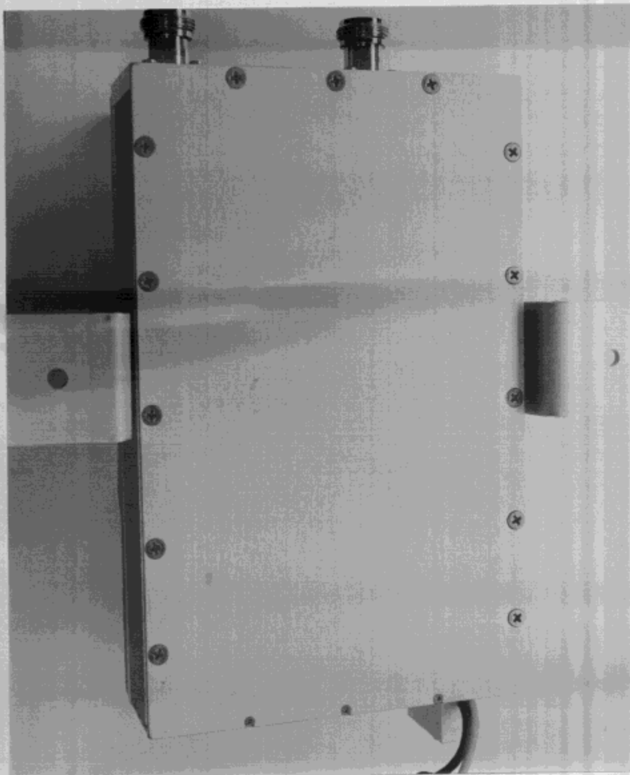
6.5 Photo: EUT Bottom View
