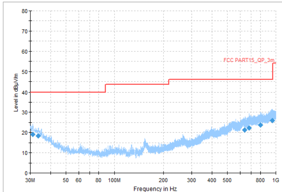
Fig. 49 Radiated Spurious Emission (All Channels, 30MHz ~ 1GHz)
