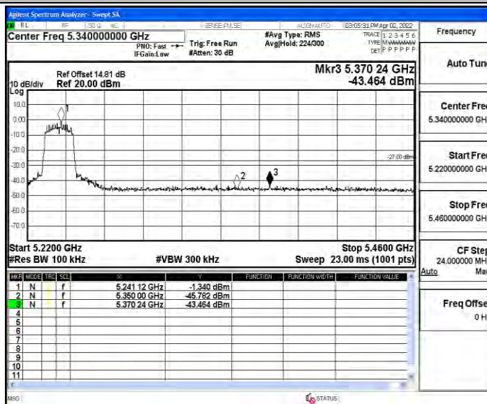
11AC20MIMO_Ant2_High_5240
