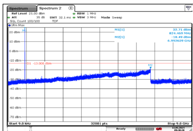
GSM 850 VOICE Low Channel
