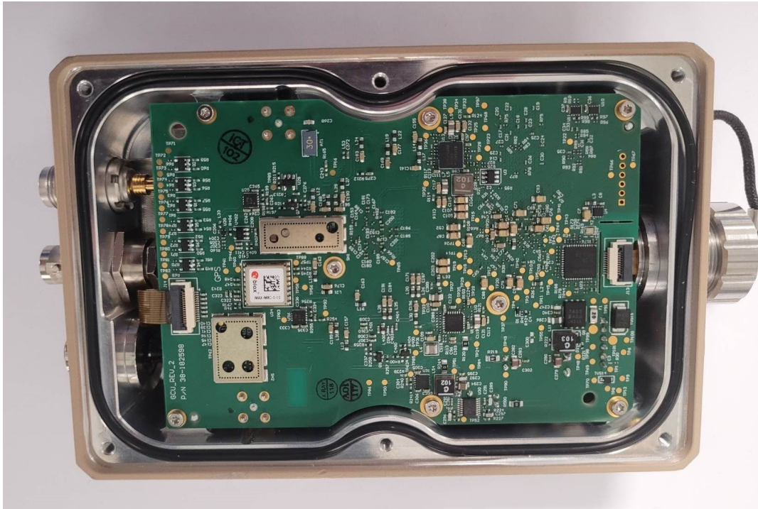
408060A Yahsat T-TAC GCU without Lid.
