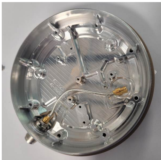
Yahsat T-TAC Vehicular Antenna Step 1 – Mounting of TNC Connector
