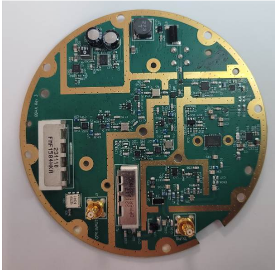
Yahsat T-TAC Vehicular Antenna PCBA TopView
