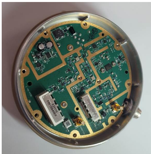
Yahsat T-TAC Vehicular Antenna Step 2 – Mounting of PCBA
