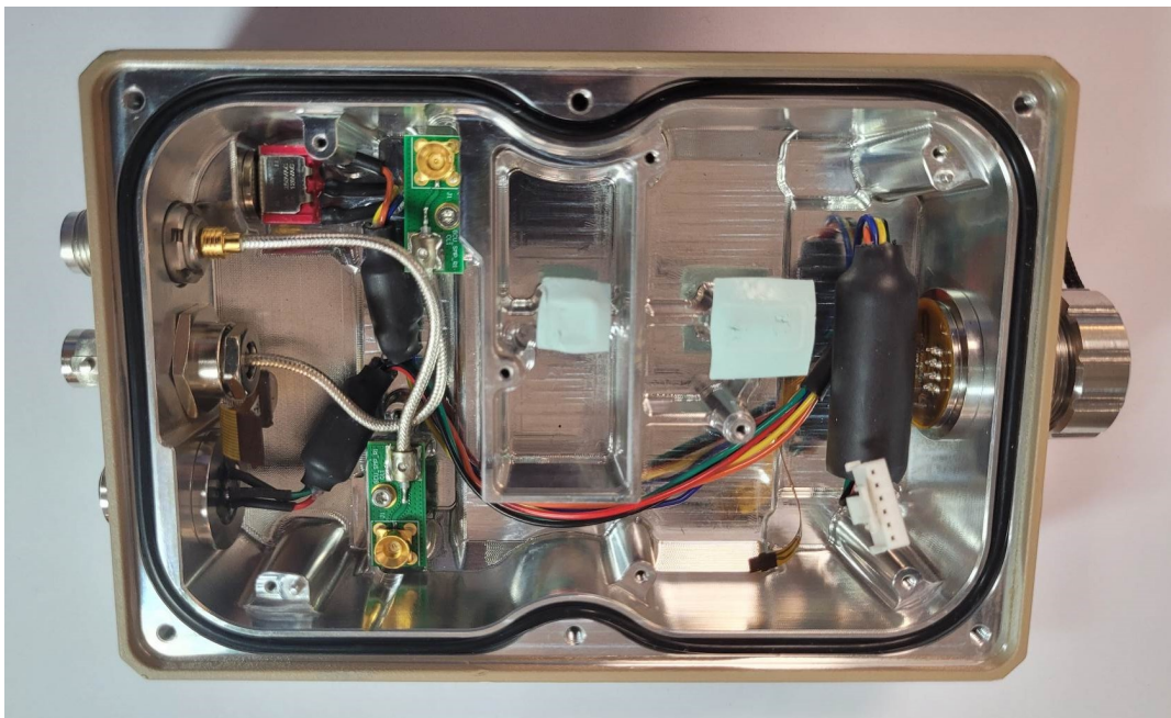
408060A Yahsat T-TAC GCU without PCBA and Lid.
