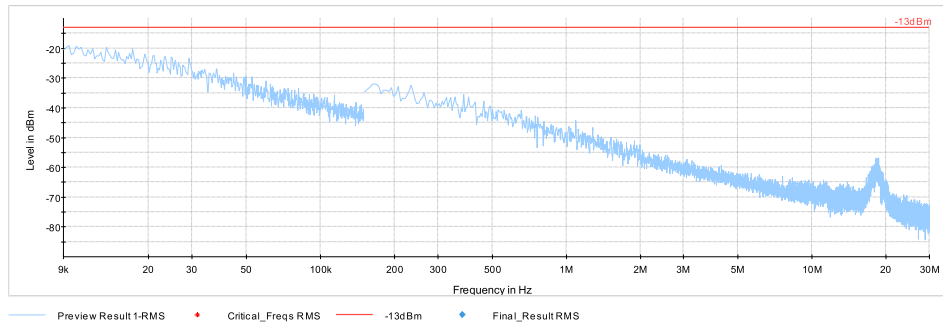
Plot # 36 Radiated Emissions: 9 kHz-30 MHz
