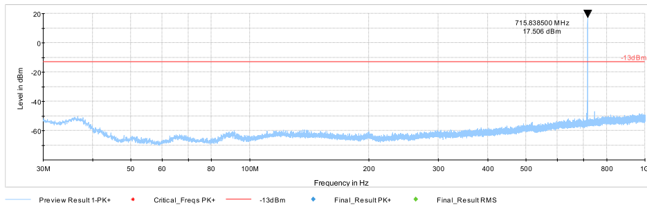
Plot #40 Radiated Emissions: 30 MHz – 1GHz
