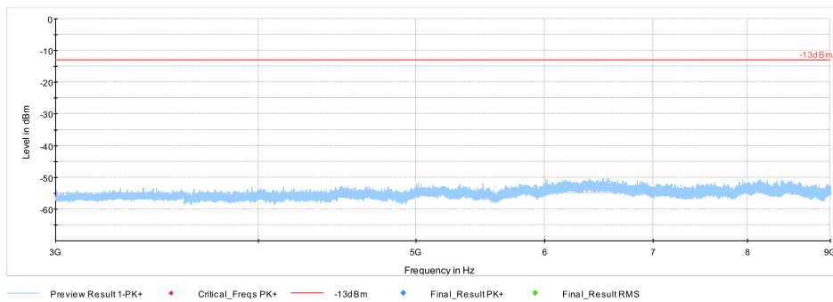
Plot #39 Radiated Emissions: 3-9 GHz
