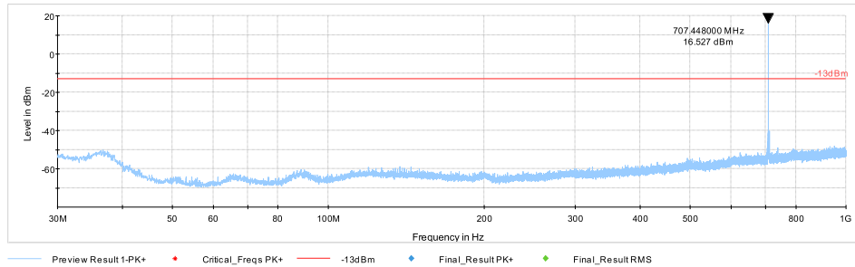
Plot #37 Radiated Emissions: 30 MHz – 1GHz
