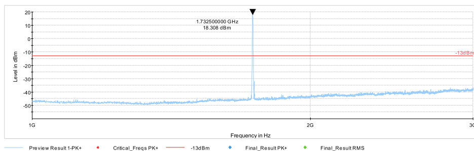
Plot #17 Radiated Emissions: 1-3 GHz
