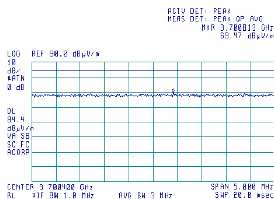
Plot 8.4.23 Radiated emission measurements at the second harmonic of mid carrier frequency
