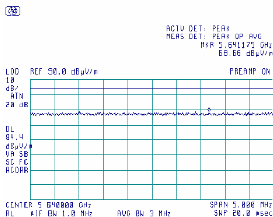
Plot 8.4.27 Radiated emission measurements at the third harmonic of high carrier frequency
