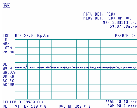
Plot 7.4.28 Radiated emission measurements at the fifth harmonic of low carrier frequency
