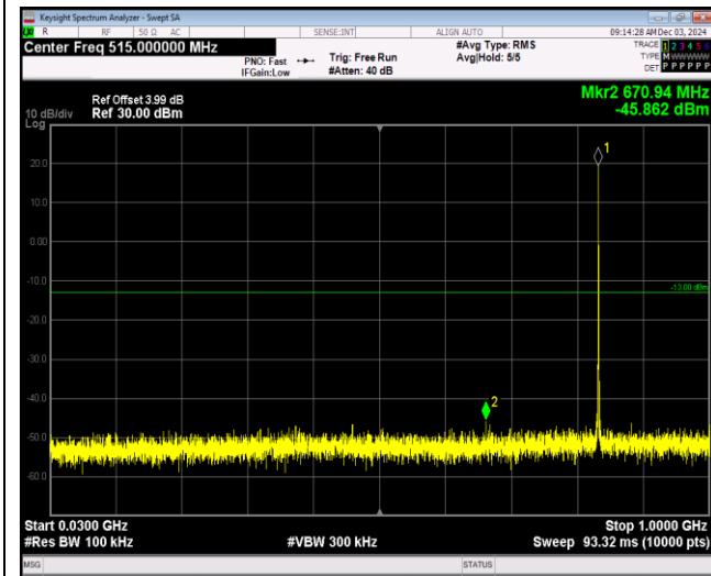
Band5-1.4MHz-64QAM-20643-1RB#0-Range1:30~1000MHz
