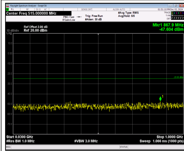
Band7-20MHz-QPSK-21100-1RB#0-Range1:30~100 OMHz
