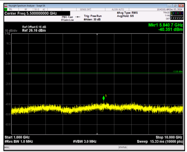
Band12-1.4MHz-64QAM-23095-1RB#0-Range2:1000~10000MHz
