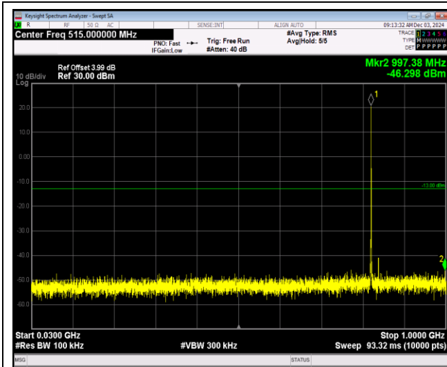
Band5-1.4MHz-64QAM-20525-1RB#0-Range1:30~1000MHz
