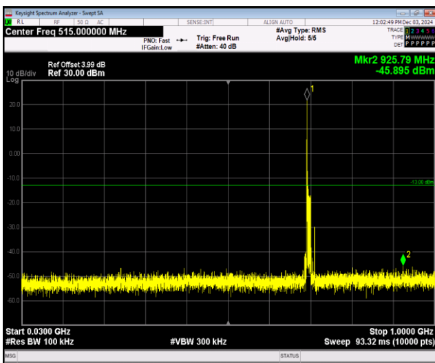
Band12-10MHz-QPSK-23095-1RB#0-Range1:30~1000MHz
