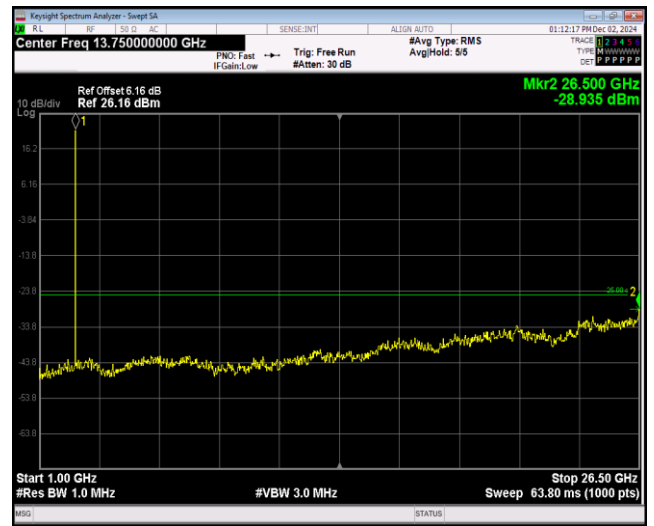
Band7-5MHz-16QAM-21425-1RB#0-Range2:1000~2 6500MHz
