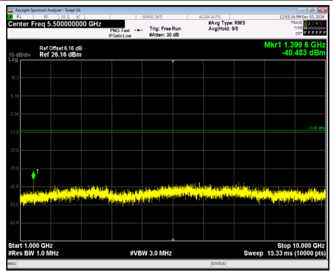
Band12-10MHz-16QAM-23060-1RB#0-Range2:1000~10000MHz
