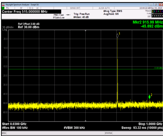
Band12-10MHz-QPSK-23060-1RB#0-Range1:30~1000MHz
