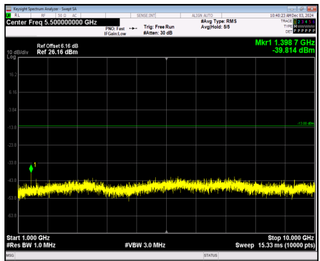
Band12-1.4MHz-16QAM-23095-1RB#0-Range2:1000~10000MHz
