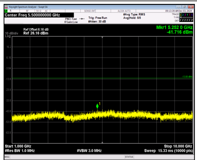
Band5-1.4MHz-64QAM-20525-1RB#0-Range2:1000~10000MHz
