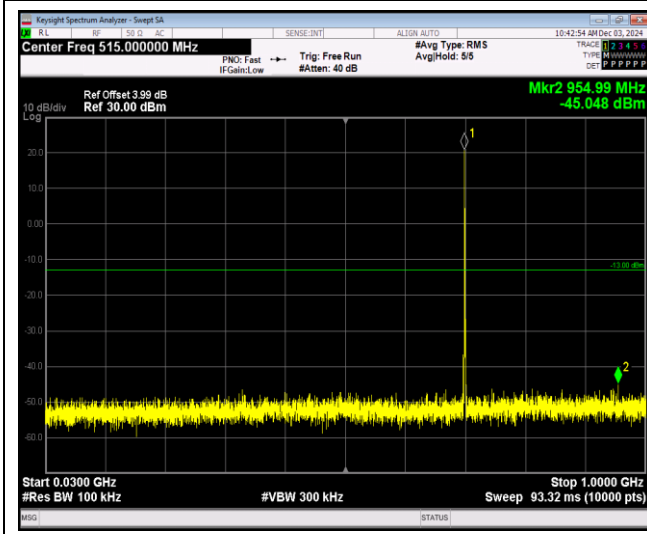
Band12-1.4MHz-64QAM-23095-1RB#0-Range1:30~1000MHz
