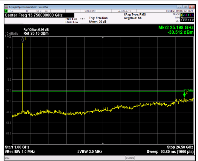
Band7-5MHz-16QAM-21100-1RB#0-Range2:1000~2 6500MHz
