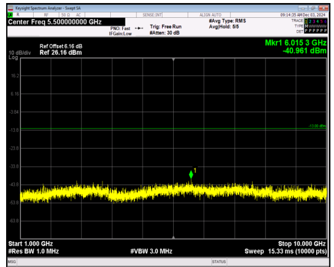
Band5-1.4MHz-64QAM-20643-1RB#0-Range2:1000~10000MHz
