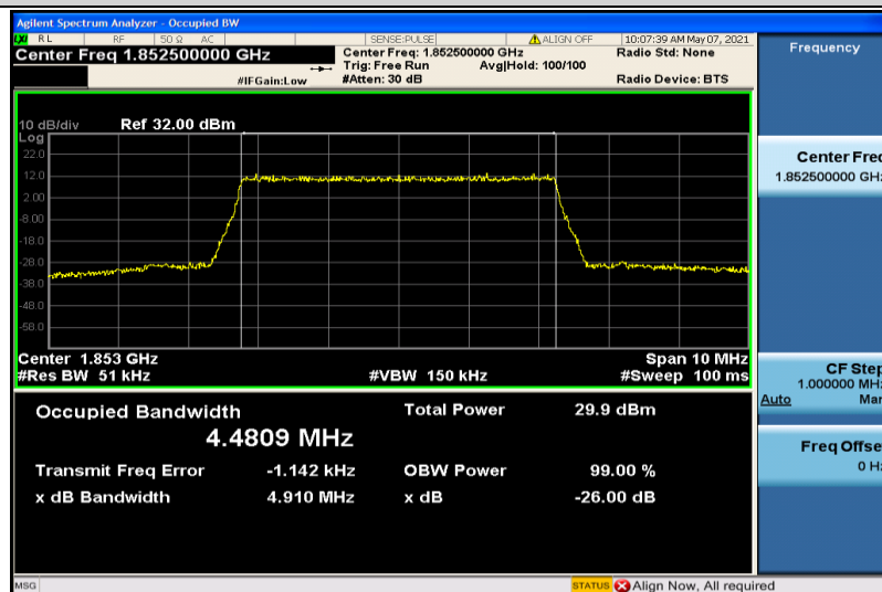
Band25-5MHz-16QAM-26065-25RB#0-4.4809
