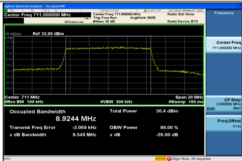
Band12-10MHz-16QAM-23130-50RB#0-8.9244
