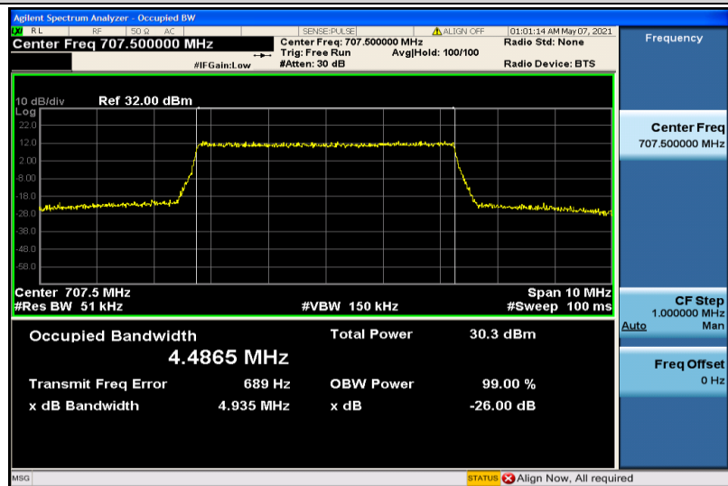
Band12-5MHz-16QAM-23095-25RB#0-4.4865
