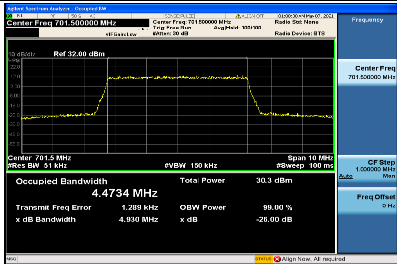
Band12-5MHz-16QAM-23035-25RB#0-4.4734
