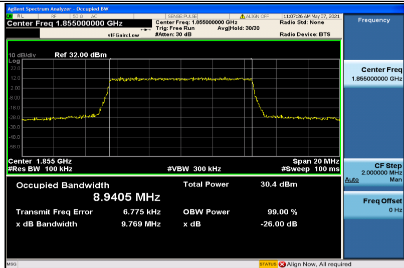
Band25-10MHz-QPSK-26090-50RB#0-8.9405
