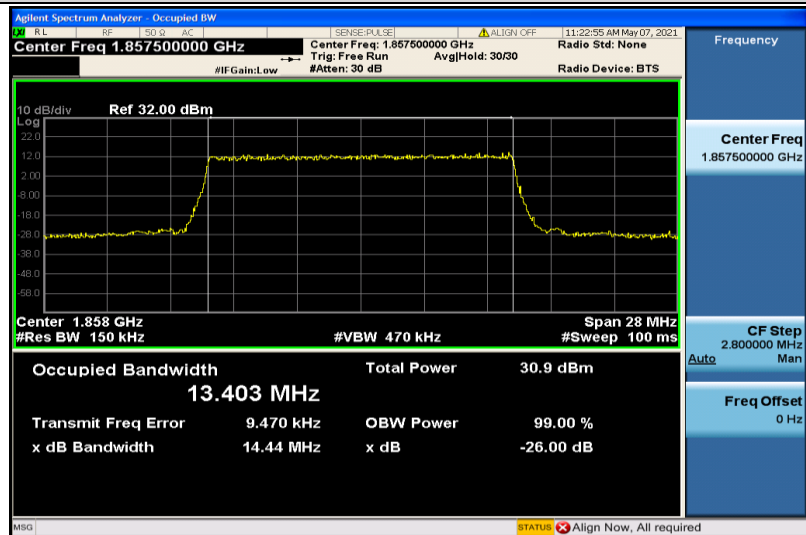
Band25-15MHz-QPSK-26115-75RB#0-13.403
