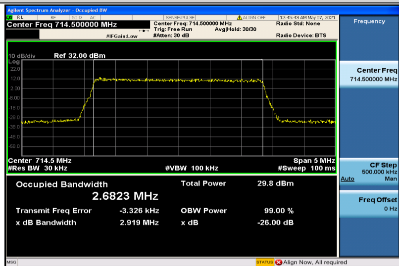
Band12-3MHz-16QAM-23165-15RB#0-2.6823
