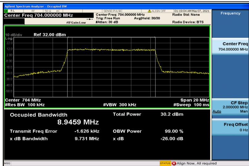
Band12-10MHz-16QAM-23060-50RB#0-8.9459
