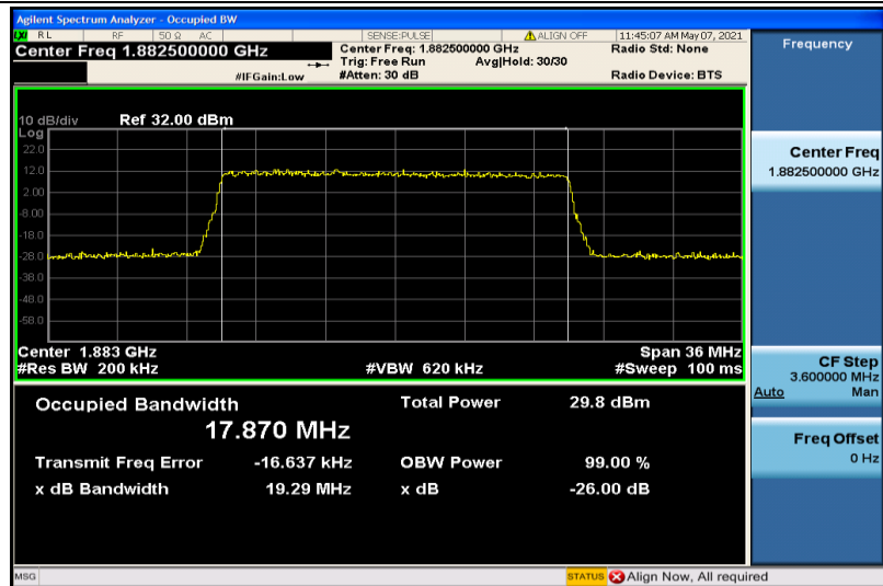
Band25-20MHz-16QAM-26365-100RB#0-17.870
