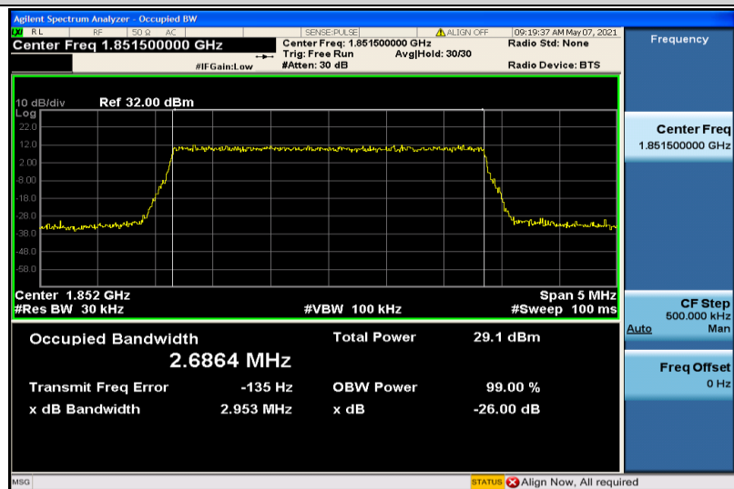
Band25-3MHz-16QAM-26055-15RB#0-2.6864
