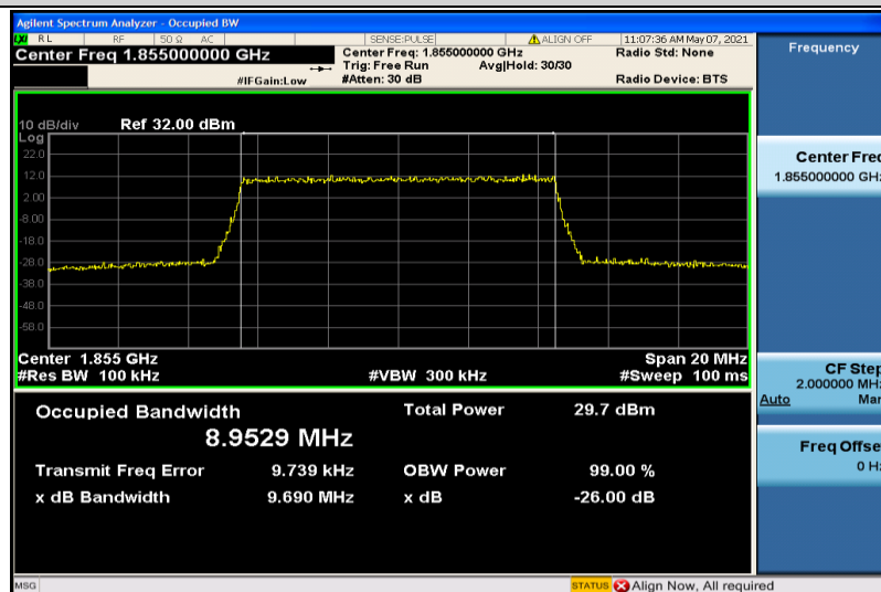
Band25-10MHz-16QAM-26090-50RB#0-8.9529
