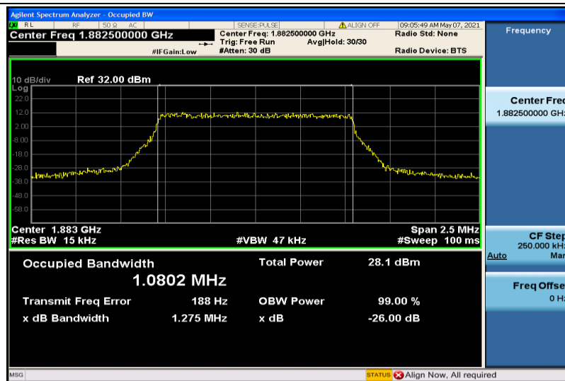
Band25-1.4MHz-16QAM-26365-6RB#0-1.0802
