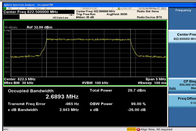
Band26-3MHz-QPSK-26775-15RB#0-2.6893
