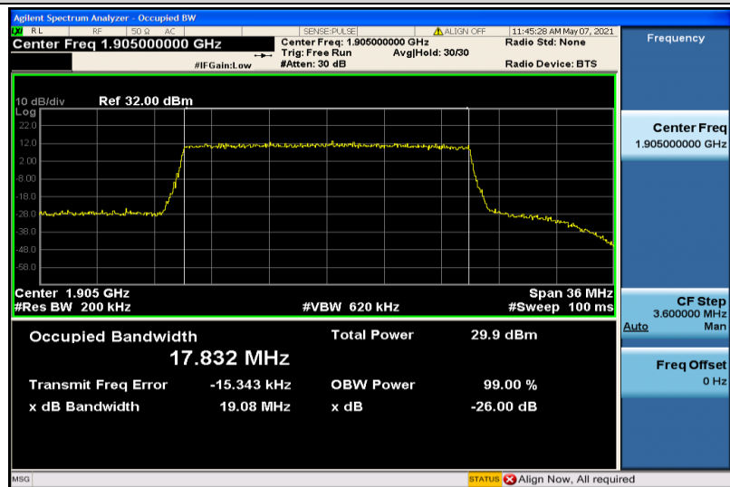
Band25-20MHz-16QAM-26590-100RB#0-17.832
