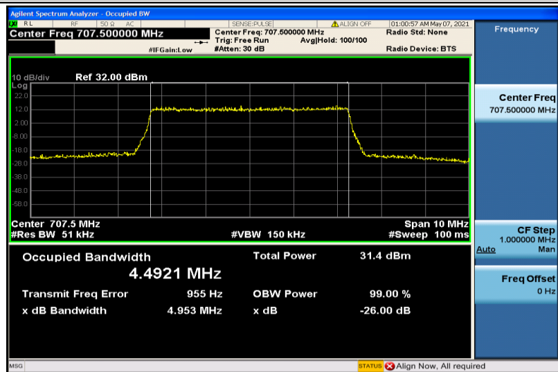
Band12-5MHz-QPSK-23095-25RB#0-4.4921
