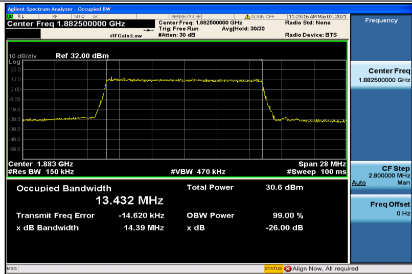
Band25-15MHz-QPSK-26365-75RB#0-13.432
