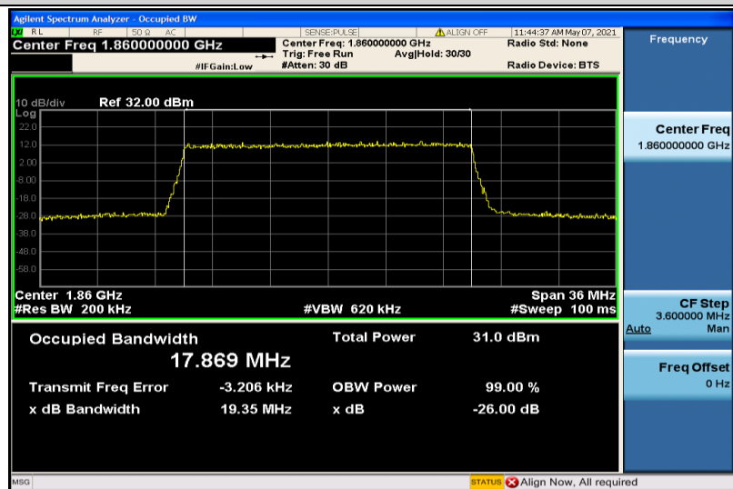
Band25-20MHz-QPSK-26140-100RB#0-17.869
