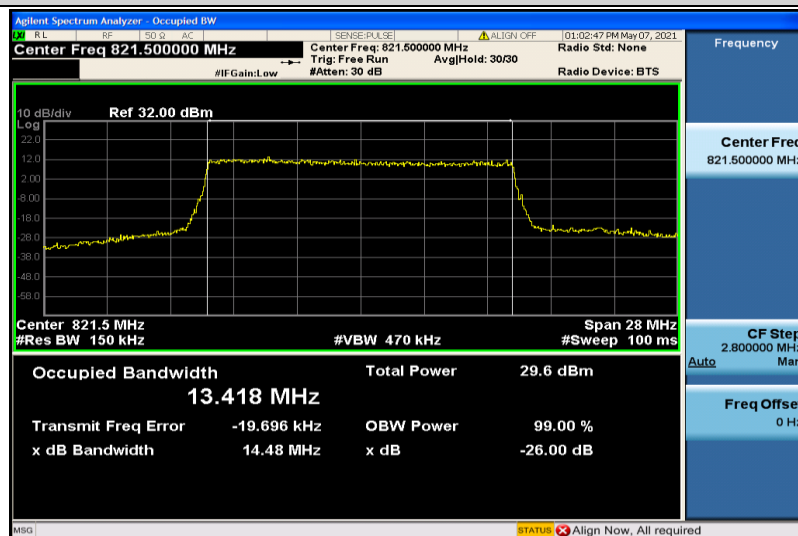
Band26-15MHz-16QAM-26765-75RB#0-13.418
