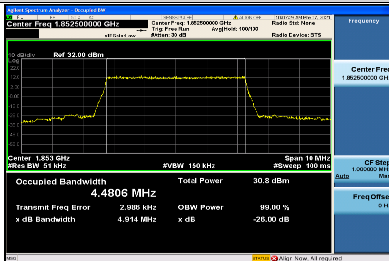
Band25-5MHz-QPSK-26065-25RB#0-4.4806
