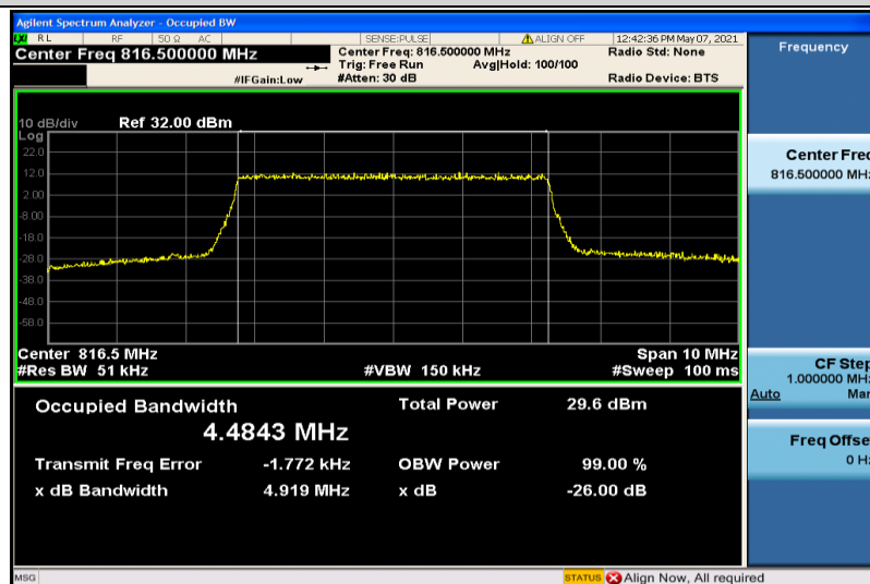
Band26-5MHz-16QAM-26715-25RB#0-4.4843
