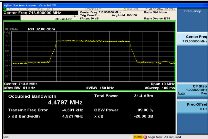
Band12-5MHz-QPSK-23155-25RB#0-4.4797
