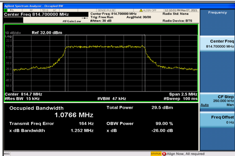
Band26-1.4MHz-QPSK-26697-6RB#0-1.0766
