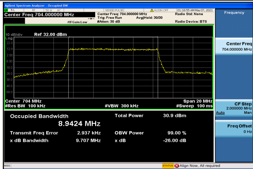
Band12-10MHz-QPSK-23060-50RB#0-8.9424
