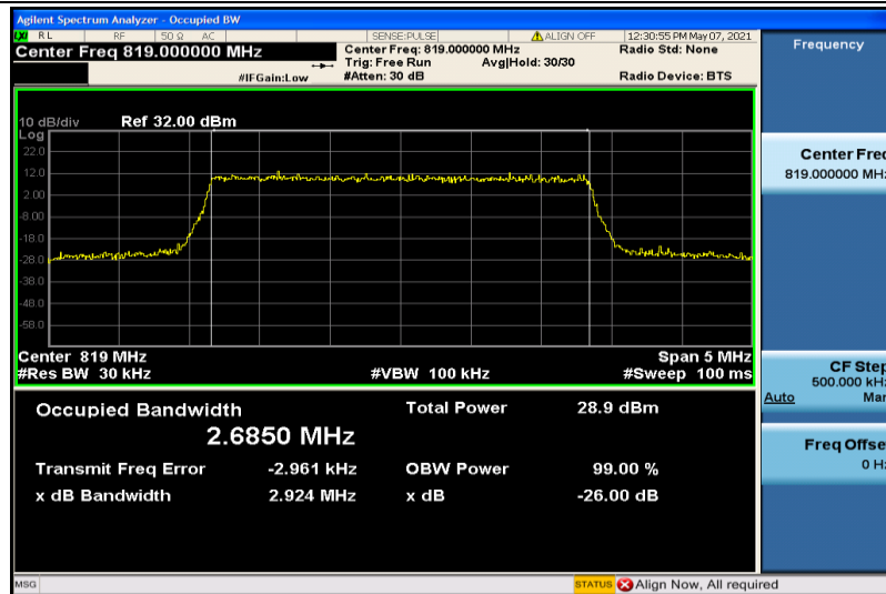
Band26-3MHz-16QAM-26740-15RB#0-2.6850
