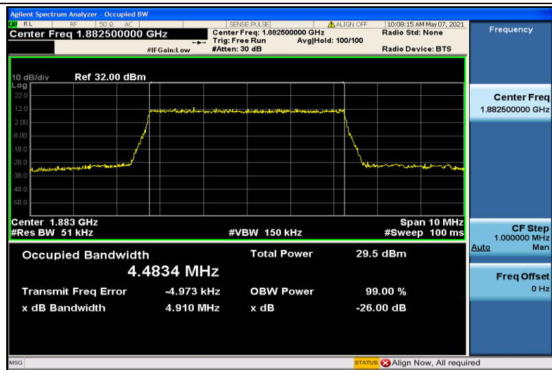
Band25-5MHz-16QAM-26365-25RB#0-4.4834
