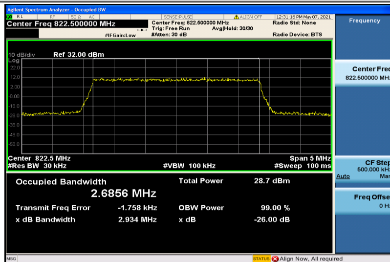
Band26-3MHz-16QAM-26775-15RB#0-2.6856
