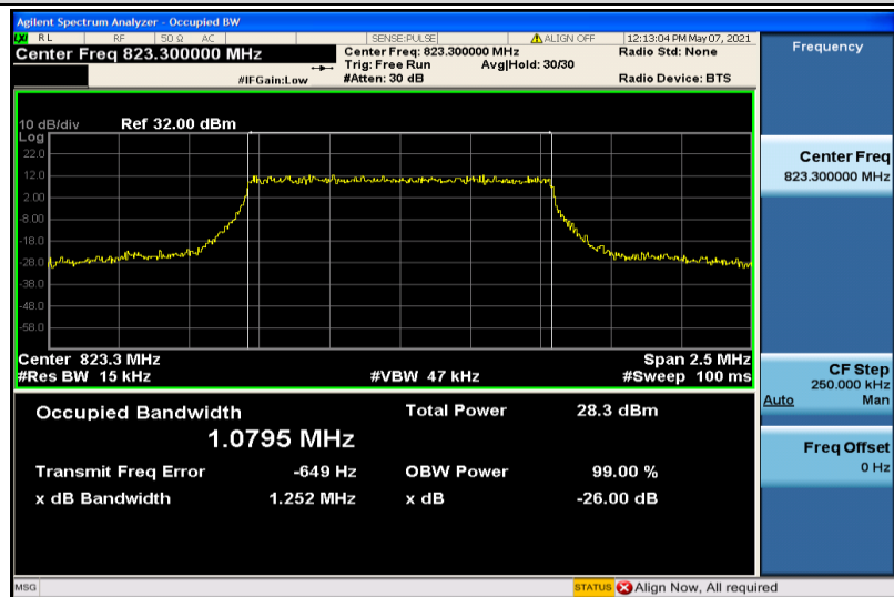
Band26-1.4MHz-16QAM-26783-6RB#0-1.0795
