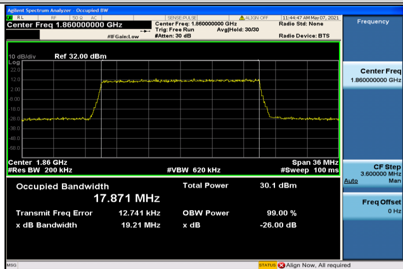
Band25-20MHz-16QAM-26140-100RB#0-17.871
