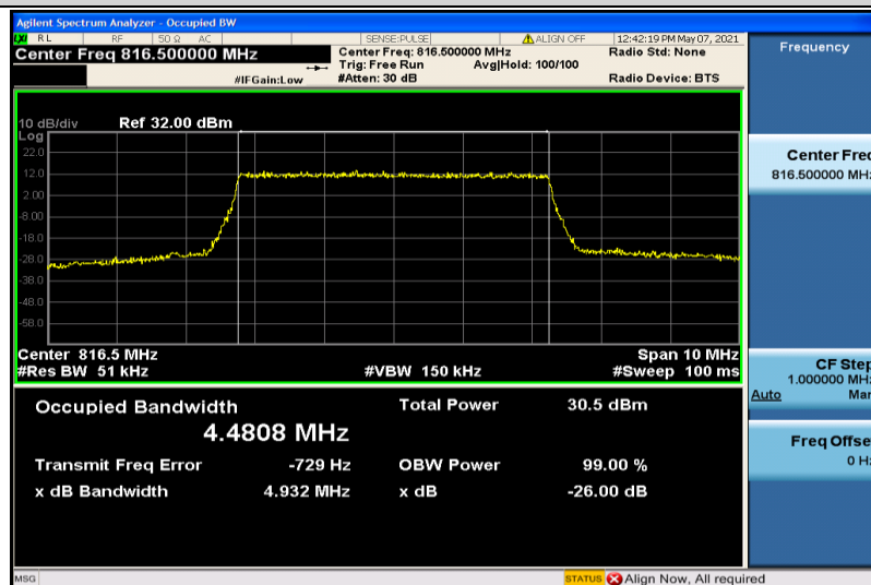
Band26-5MHz-QPSK-26715-25RB#0-4.4808
