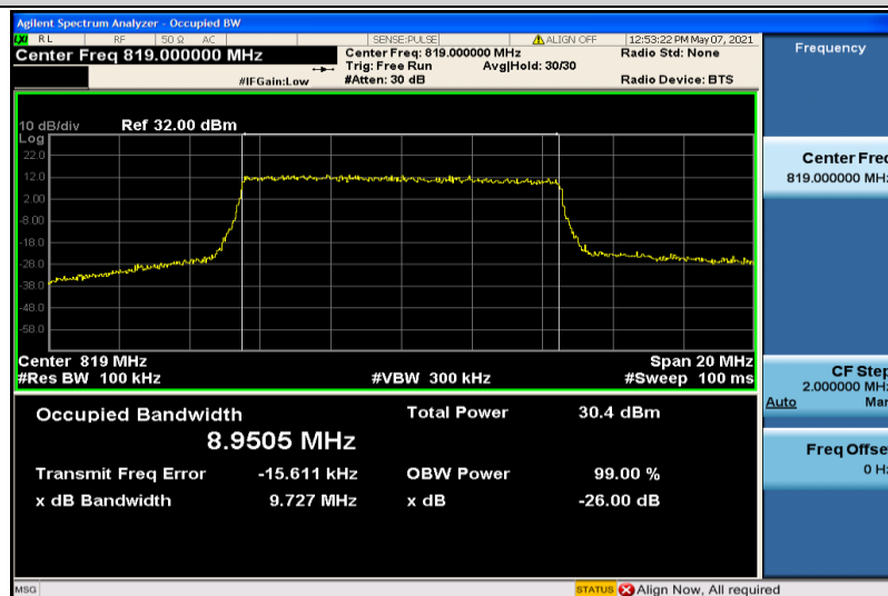
Band26-10MHz-QPSK-26740-50RB#0-8.9505
