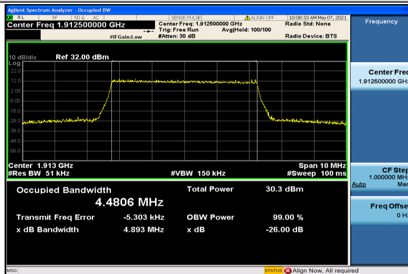
Band25-5MHz-QPSK-26665-25RB#0-4.4806
