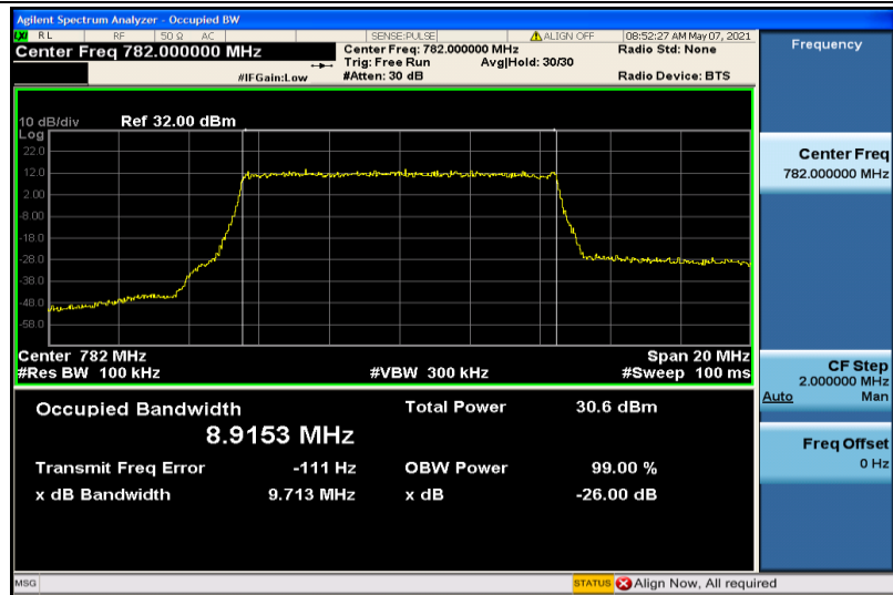
Band13-10MHz-QPSK-23230-50RB#0-8.9153
