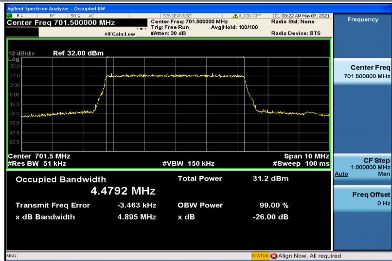
Band12-5MHz-QPSK-23035-25RB#0-4.4792
