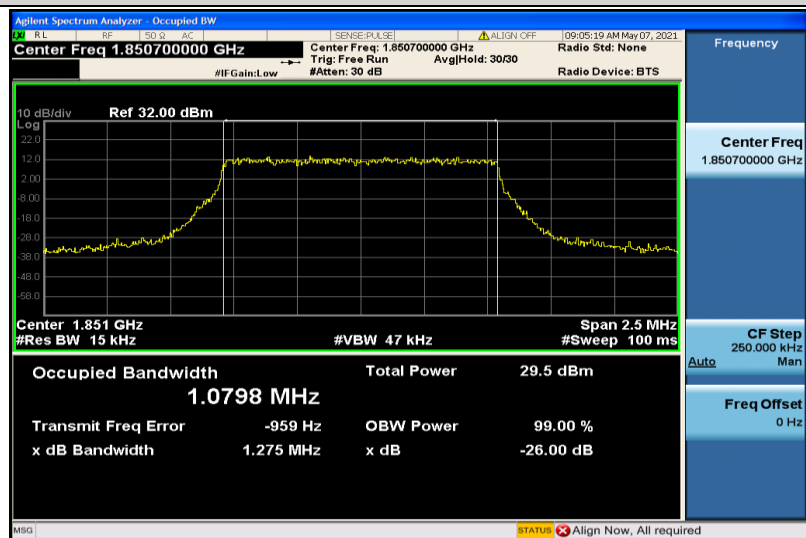
Band25-1.4MHz-QPSK-26047-6RB#0-1.0798
