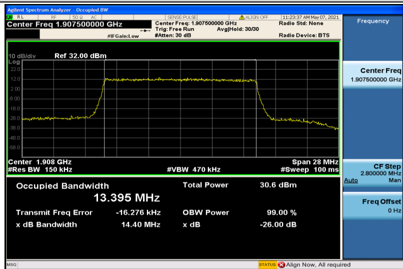
Band25-15MHz-QPSK-26615-75RB#0-13.395
