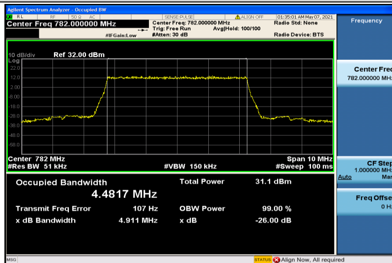
Band13-5MHz-QPSK-23230-25RB#0-4.4817
