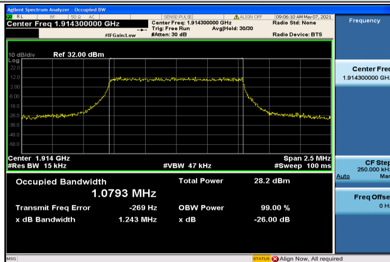
Band25-1.4MHz-16QAM-26683-6RB#0-1.0793
