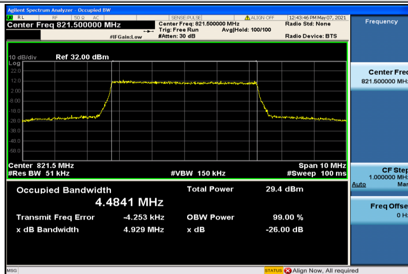
Band26-5MHz-16QAM-26765-25RB#0-4.4841
