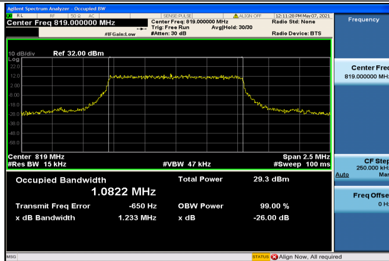
Band26-1.4MHz-QPSK-26740-6RB#0-1.0822
