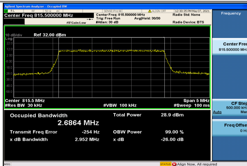
Band26-3MHz-16QAM-26705-15RB#0-2.6864
