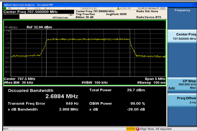
Band12-3MHz-16QAM-23095-15RB#0-2.6884
