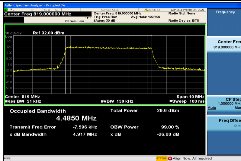
Band26-5MHz-16QAM-26740-25RB#0-4.4850
