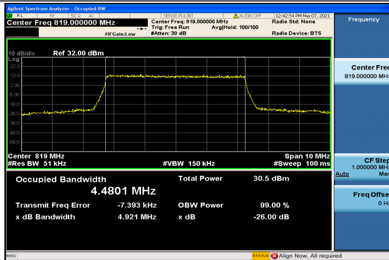
Band26-5MHz-QPSK-26740-25RB#0-4.4801
