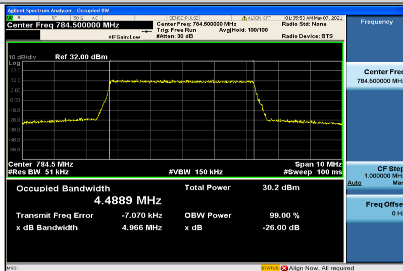
Band13-5MHz-16QAM-23255-25RB#0-4.4889
