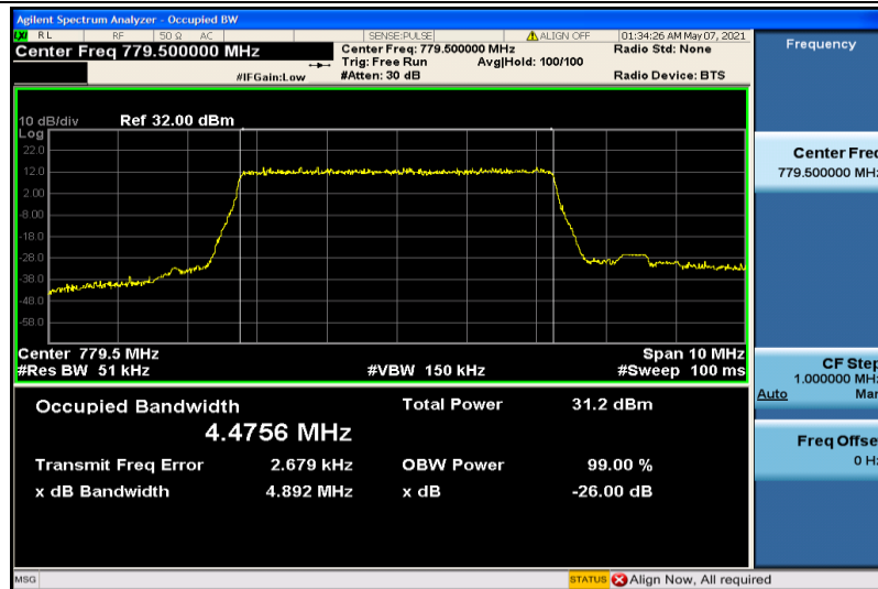
Band13-5MHz-QPSK-23205-25RB#0-4.4756
