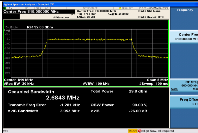
Band26-3MHz-QPSK-26740-15RB#0-2.6843
