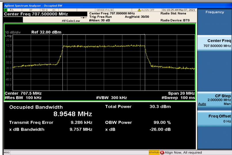
Band12-10MHz-16QAM-23095-50RB#0-8.9548
