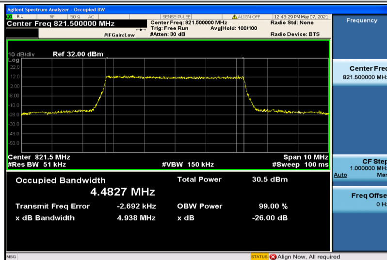
Band26-5MHz-QPSK-26765-25RB#0-4.4827
