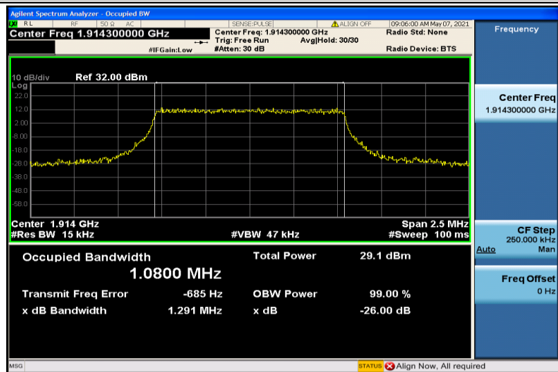
Band25-1.4MHz-QPSK-26683-6RB#0-1.0800
