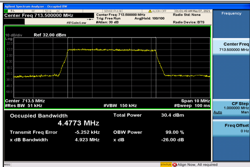
Band12-5MHz-16QAM-23155-25RB#0-4.4773
