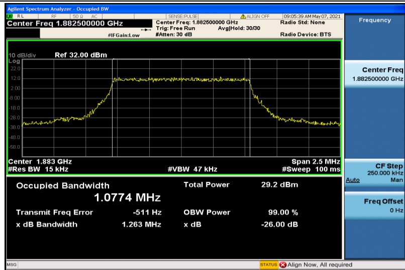
Band25-1.4MHz-QPSK-26365-6RB#0-1.0774
