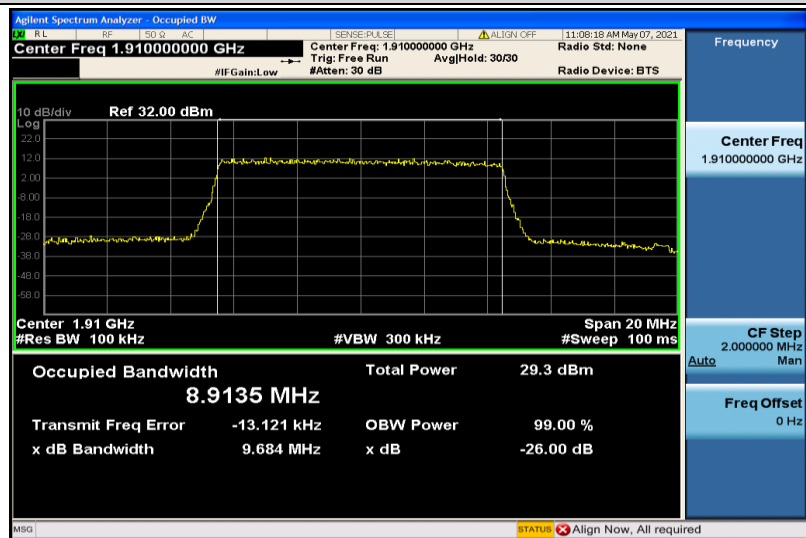
Band25-10MHz-16QAM-26640-50RB#0-8.9135
