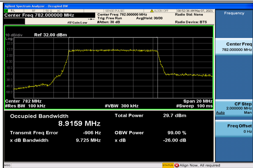
Band13-10MHz-16QAM-23230-50RB#0-8.9159
