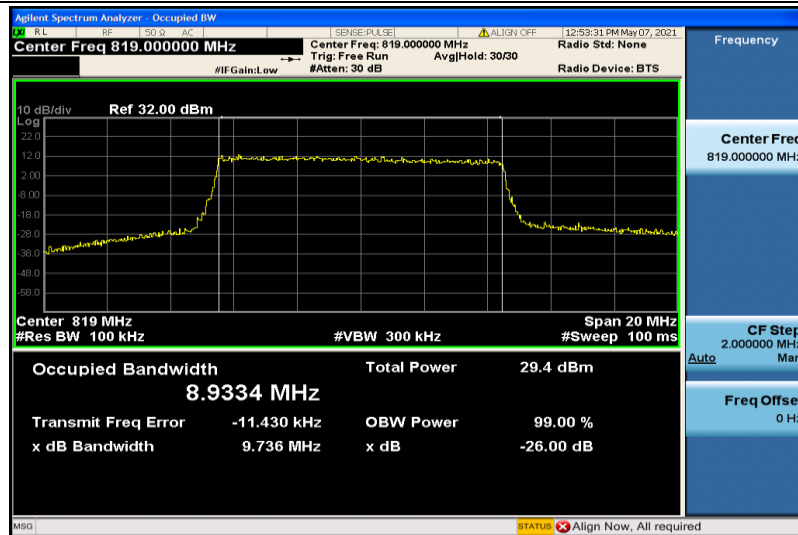
Band26-10MHz-16QAM-26740-50RB#0-8.9334
