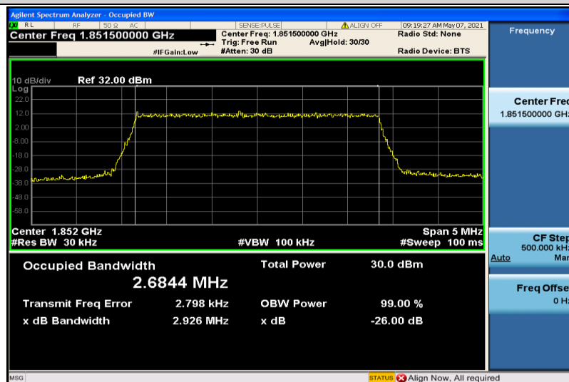
Band25-3MHz-QPSK-26055-15RB#0-2.6844
