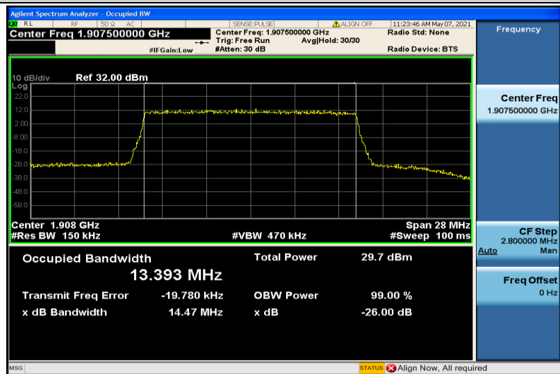
Band25-15MHz-16QAM-26615-75RB#0-13.393
