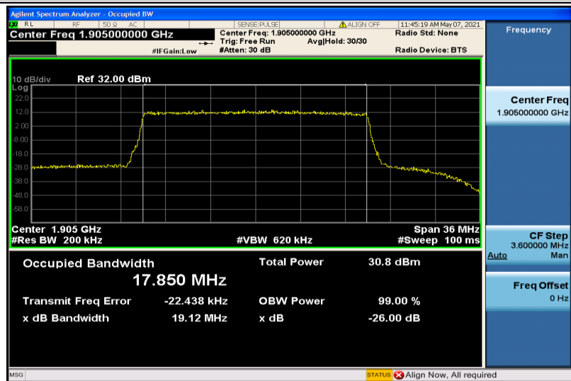
Band25-20MHz-QPSK-26590-100RB#0-17.850
