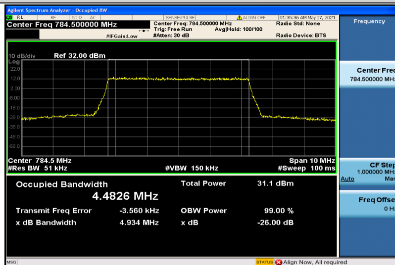
Band13-5MHz-QPSK-23255-25RB#0-4.4826
