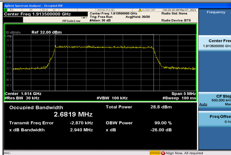
Band25-3MHz-16QAM-26675-15RB#0-2.6819
