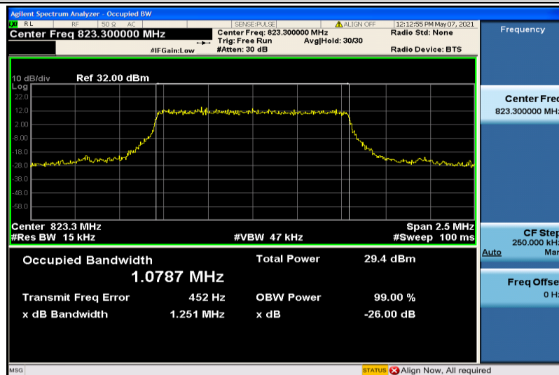
Band26-1.4MHz-QPSK-26783-6RB#0-1.0787
