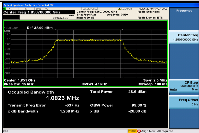
Band25-1.4MHz-16QAM-26047-6RB#0-1.0823
