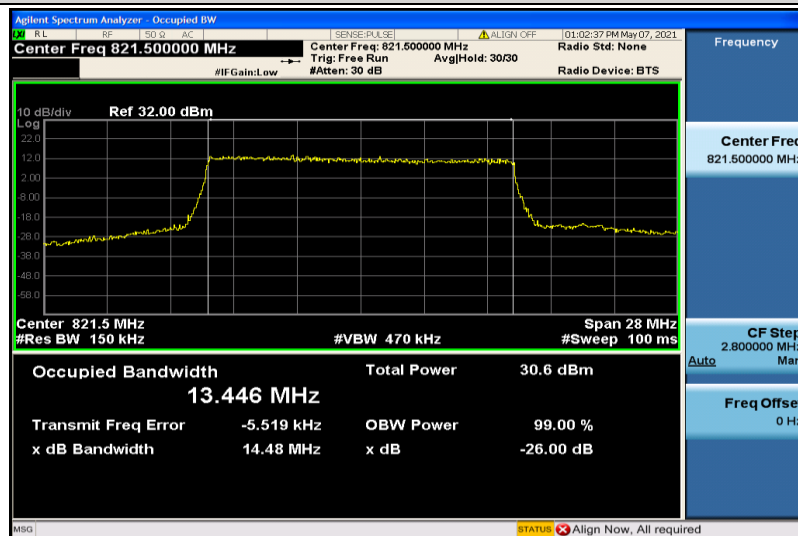
Band26-15MHz-QPSK-26765-75RB#0-13.446
