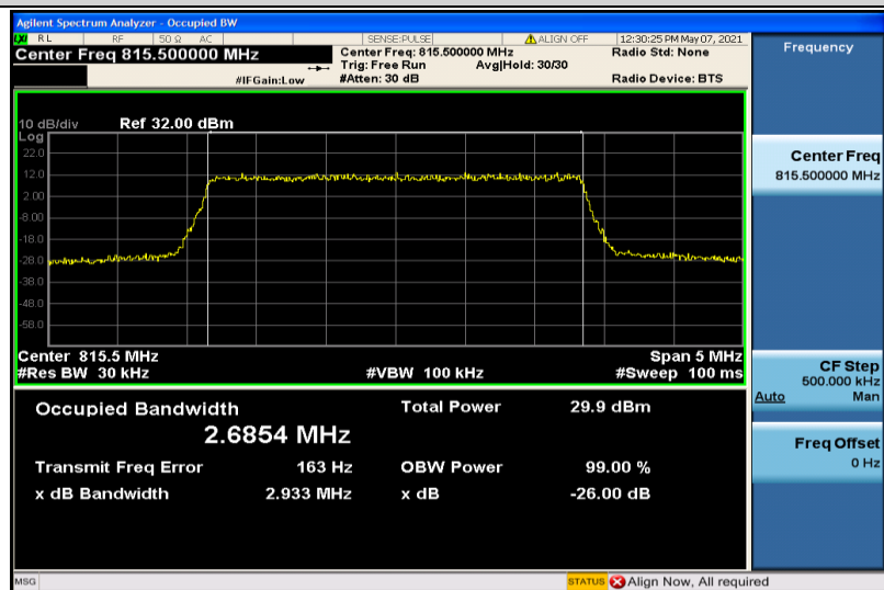
Band26-3MHz-QPSK-26705-15RB#0-2.6854
