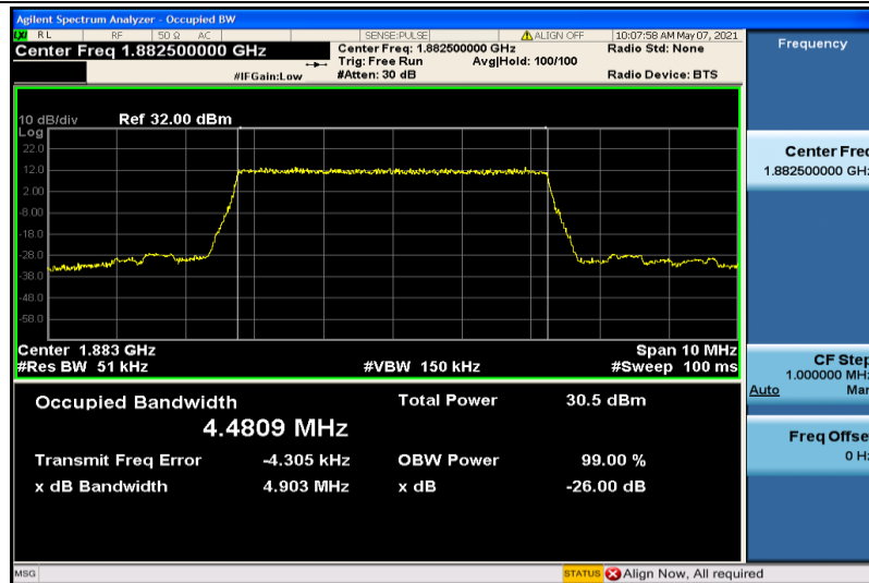
Band25-5MHz-QPSK-26365-25RB#0-4.4809
