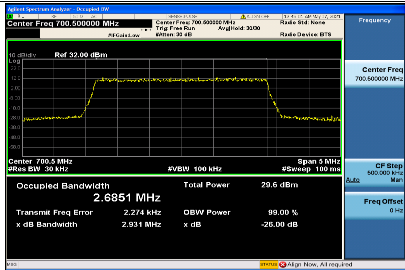
Band12-3MHz-16QAM-23025-15RB#0-2.6851
