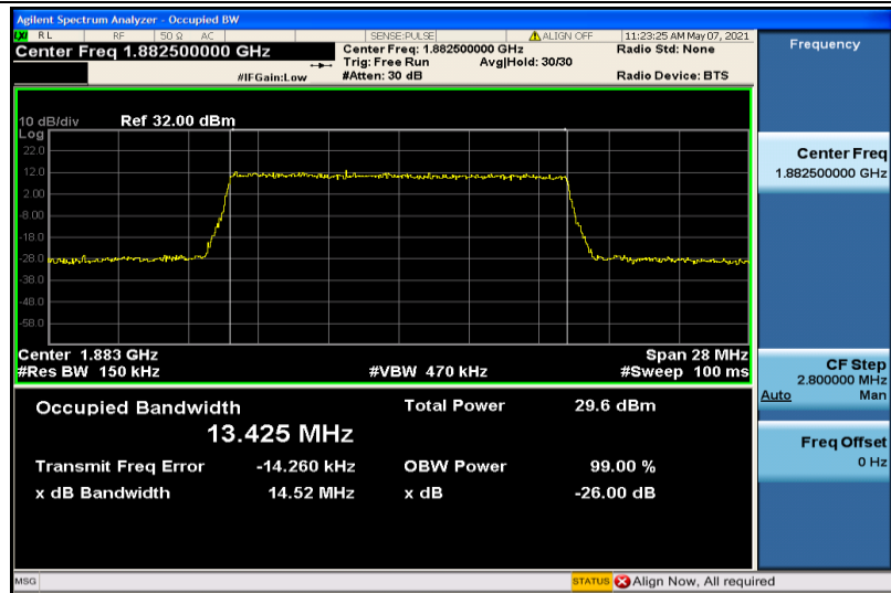
Band25-15MHz-16QAM-26365-75RB#0-13.425
