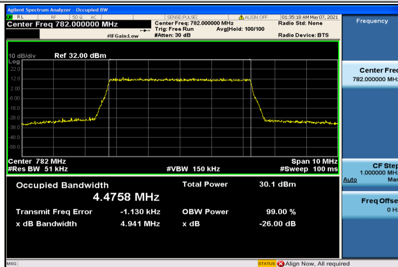
Band13-5MHz-16QAM-23230-25RB#0-4.4758
