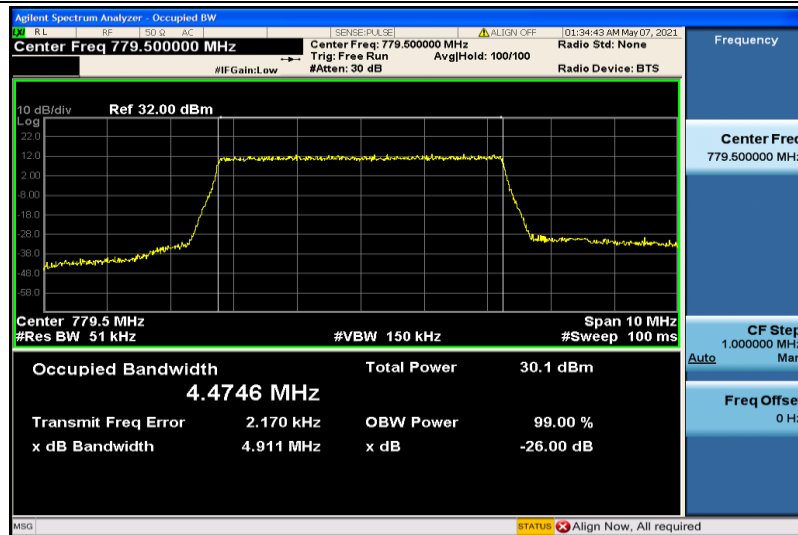
Band13-5MHz-16QAM-23205-25RB#0-4.4746
