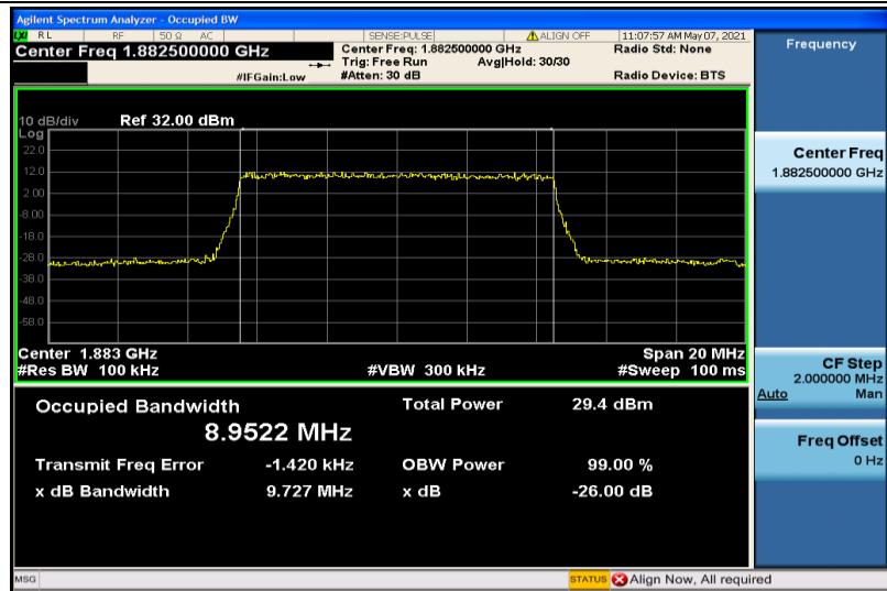
Band25-10MHz-16QAM-26365-50RB#0-8.9522
