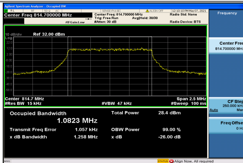
Band26-1.4MHz-16QAM-26697-6RB#0-1.0823
