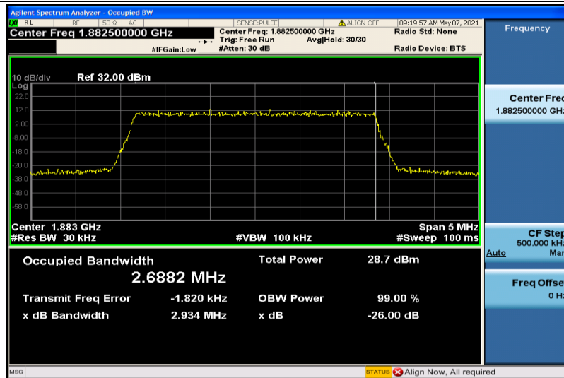
Band25-3MHz-16QAM-26365-15RB#0-2.6882
