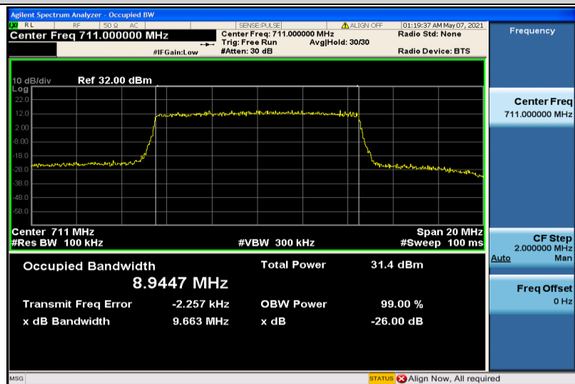
Band12-10MHz-QPSK-23130-50RB#0-8.9447
