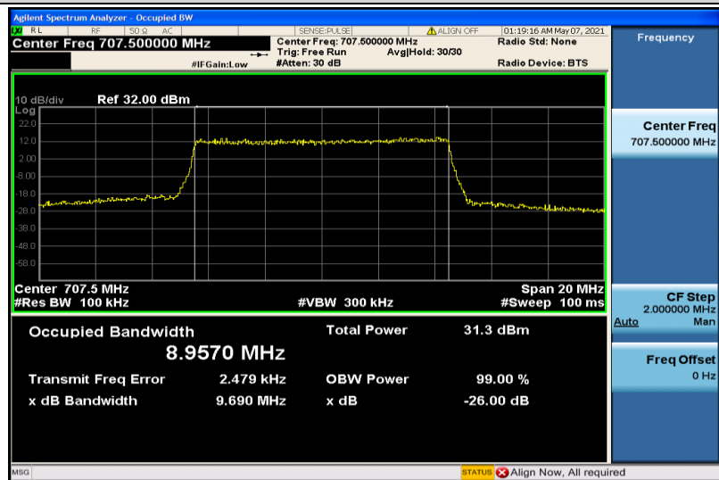
Band12-10MHz-QPSK-23095-50RB#0-8.9570
