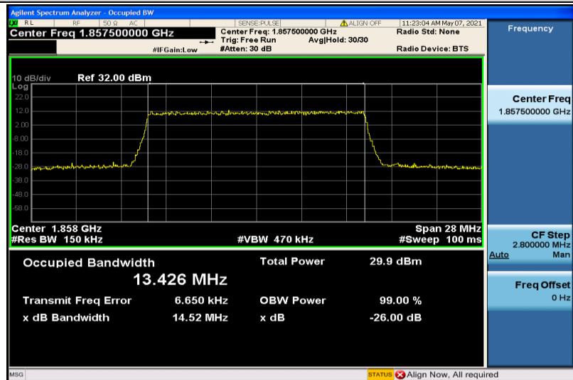
Band25-15MHz-16QAM-26115-75RB#0-13.426
