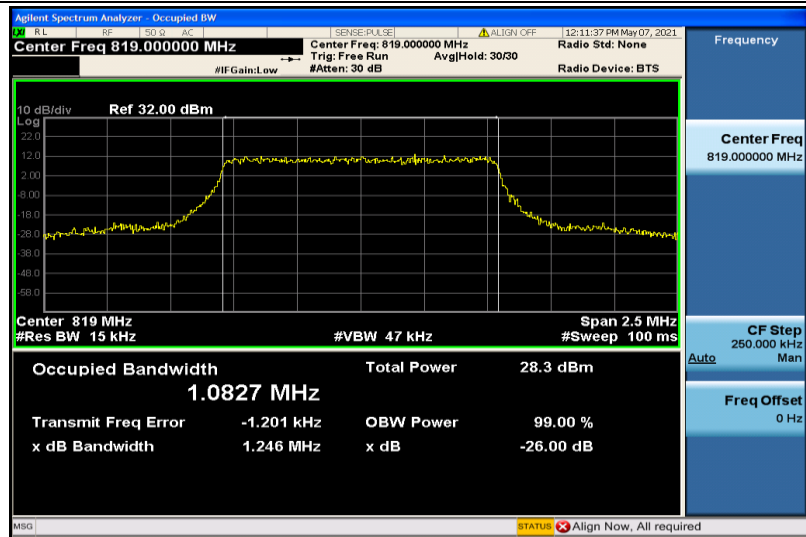
Band26-1.4MHz-16QAM-26740-6RB#0-1.0827
