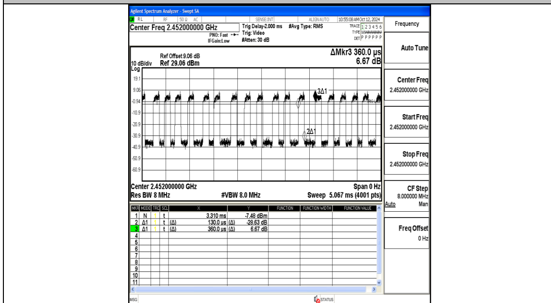
NTNV-11N40MIMO-Ant1-2452
