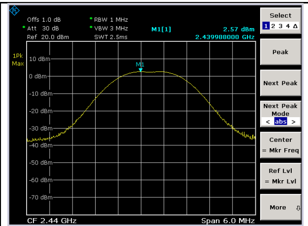
BLE-Power-Mid-1Mbps
