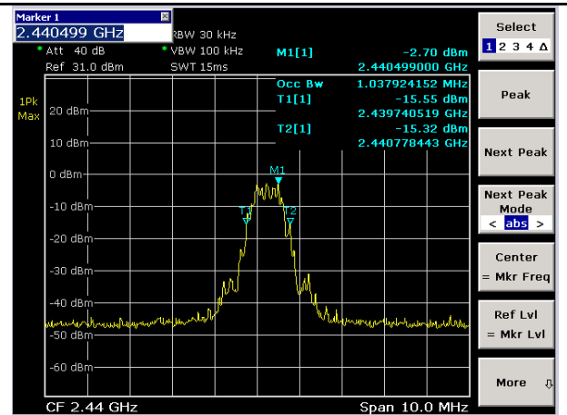
BLE-OBW-Mid-1Mbps
