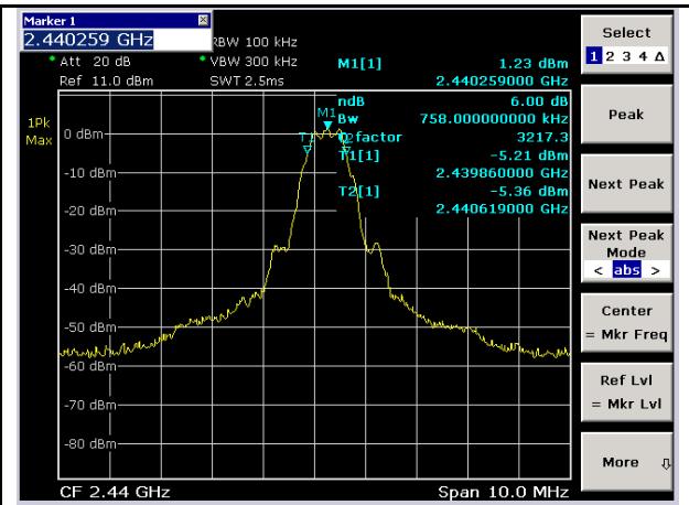
BLE-DTS BW-Mid-1Mbps
