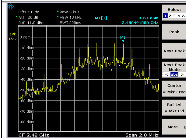
BLE-PSD-High-1Mbps
