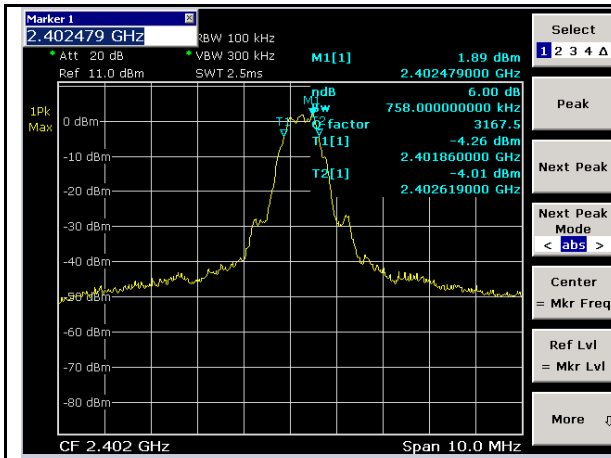
BLE-DTS BW-Low-1Mbps
