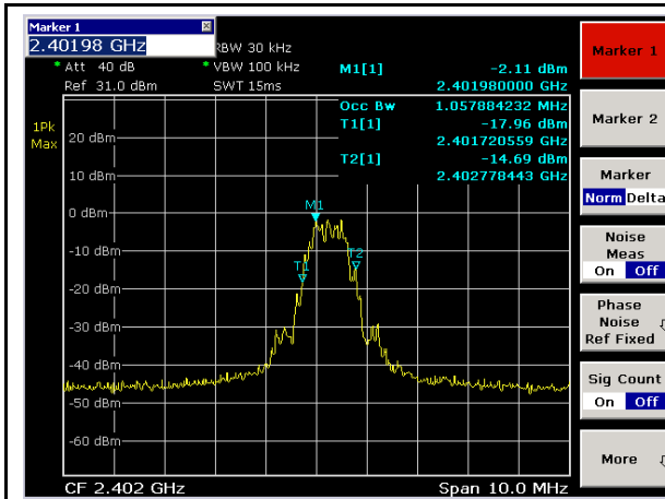
BLE-OBW-Low-1Mbps
