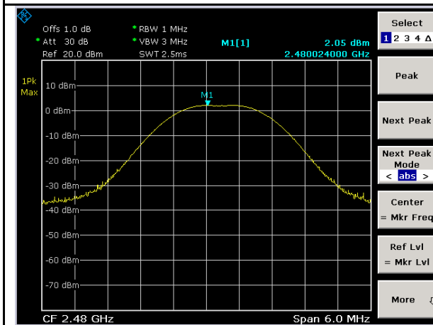
BLE-Power-High-1Mbps
