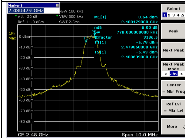
BLE-DTS BW-High-1Mbps
