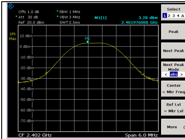
BLE-Power-Low-1Mbps
