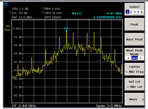
BLE-PSD-Mid-1Mbps
