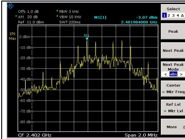
BLE-PSD-Low-1Mbps
