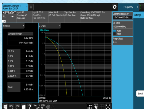
Band4-15MHz-QPSK-20325-1RB#0-PASS
