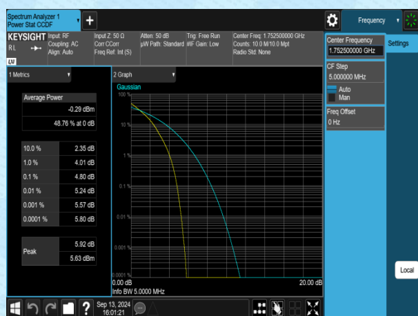
Band4-5MHz-QPSK-20375-1RB#0-PASS
