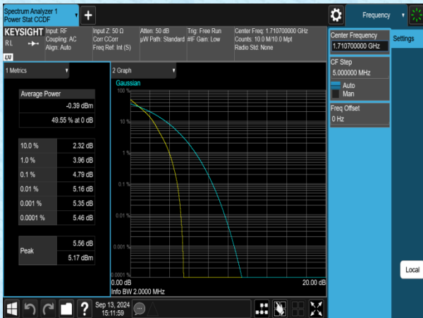
Band4-1.4MHz-QPSK-19957-1RB#0-PASS
