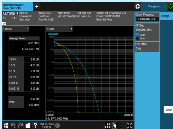
Band4-3MHz-QPSK-20175-1RB#0-PASS
