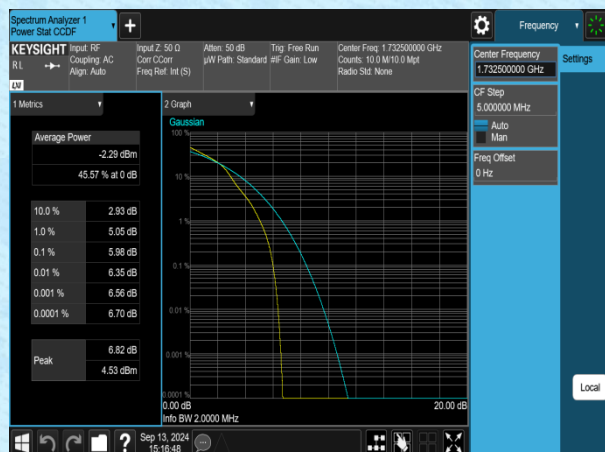
Band4-1.4MHz-16QAM-20175-1RB#0-PASS
