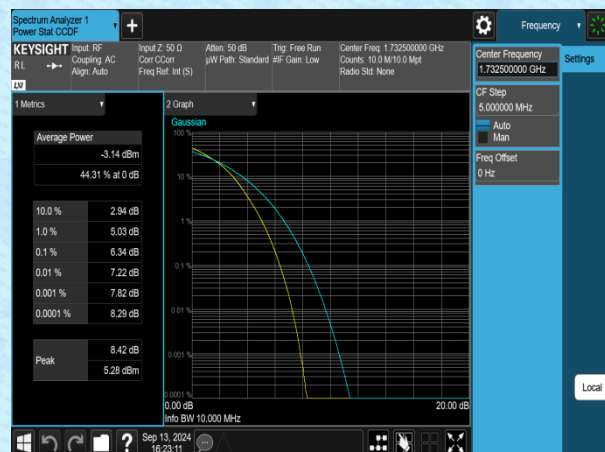
Band4-10MHz-16QAM-20175-50RB#0-PASS
