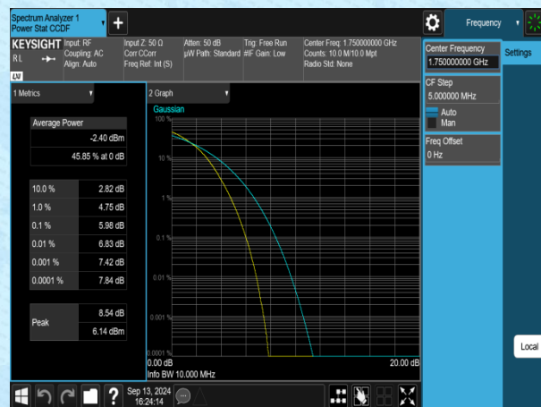
Band4-10MHz-16QAM-20350-50RB#0-PASS
