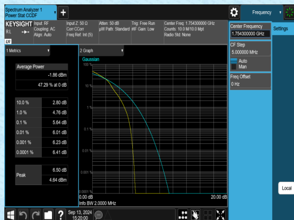
Band4-1.4MHz-16QAM-20393-1RB#0-PASS
