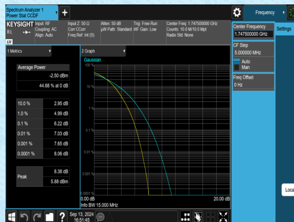
Band4-15MHz-16QAM-20325-75RB#0-PASS
