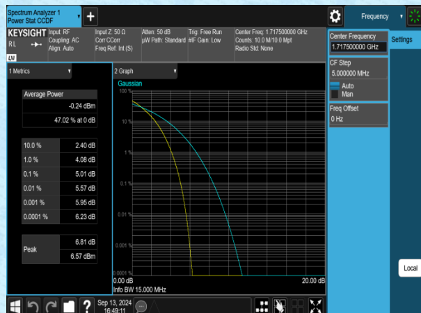
Band4-15MHz-QPSK-20025-1RB#0-PASS
