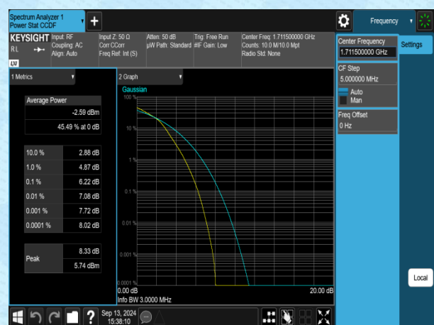
Band4-3MHz-16QAM-19965-15RB#0-PASS
