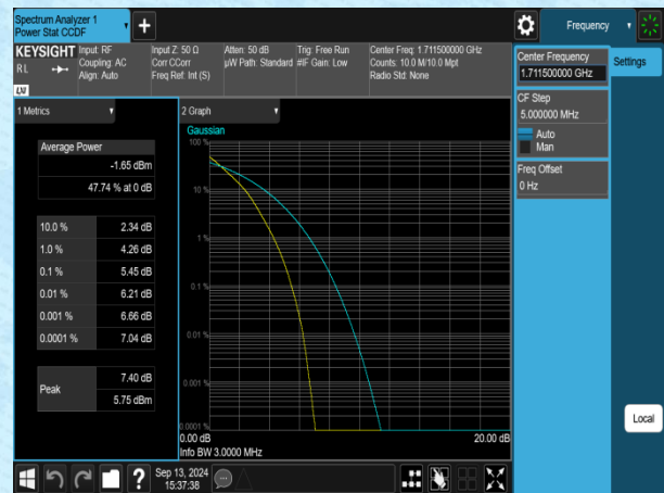
Band4-3MHz-QPSK-19965-15RB#0-PASS
