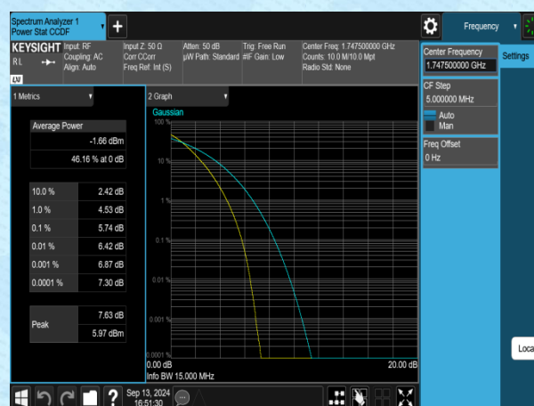
Band4-15MHz-QPSK-20325-75RB#0-PASS
