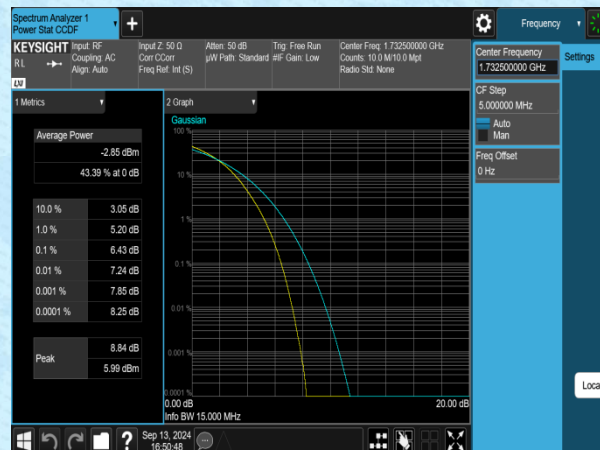
Band4-15MHz-16QAM-20175-75RB#0-PASS
