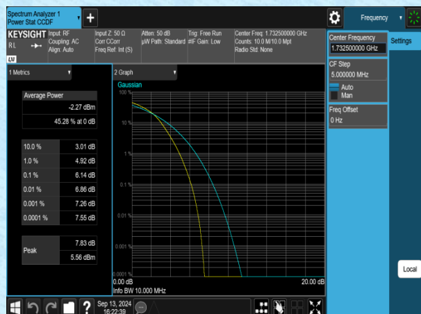
Band4-10MHz-16QAM-20175-1RB#0-PASS
