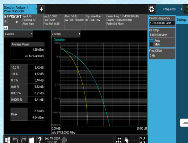
Band4-1.4MHz-QPSK-20393-6RB#0-PASS
