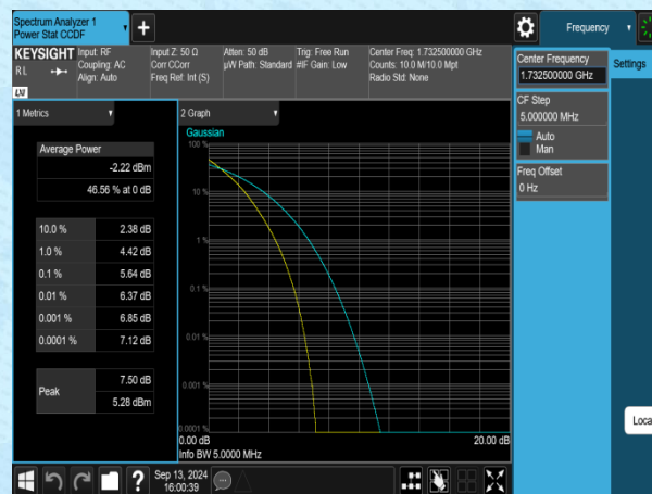
Band4-5MHz-QPSK-20175-25RB#0-PASS
