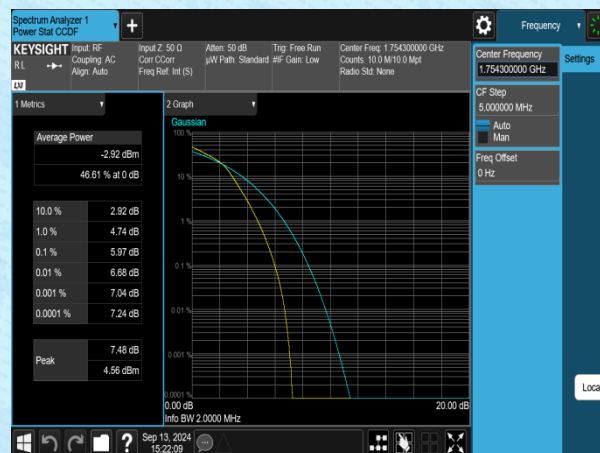
Band4-1.4MHz-16QAM-20393-6RB#0-PASS
