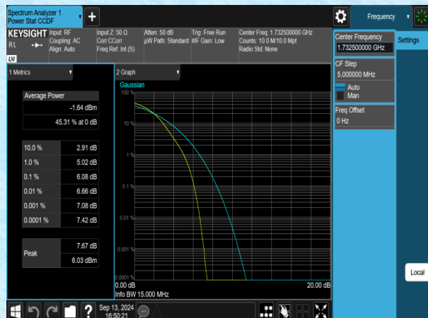
Band4-15MHz-16QAM-20175-1RB#0-PASS
