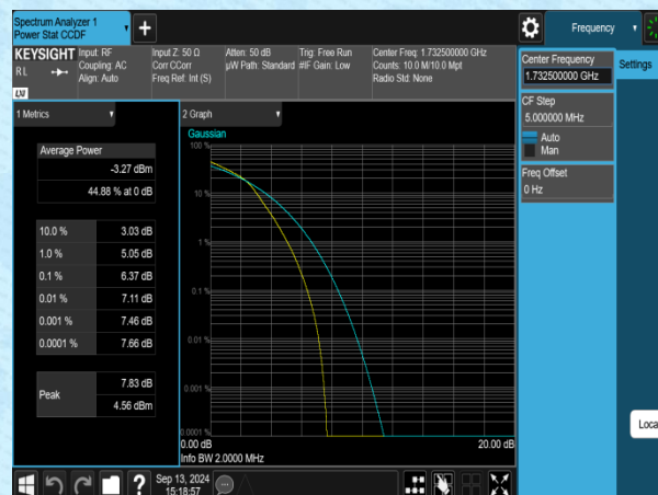
Band4-1.4MHz-16QAM-20175-6RB#0-PASS
