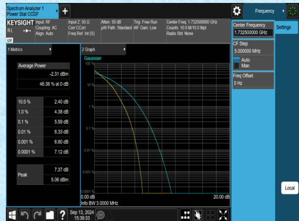
Band4-3MHz-QPSK-20175-15RB#0-PASS
