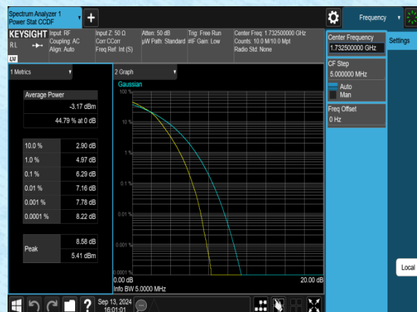
Band4-5MHz-16QAM-20175-25RB#0-PASS
