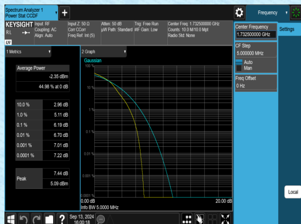
Band4-5MHz-16QAM-20175-1RB#0-PASS
