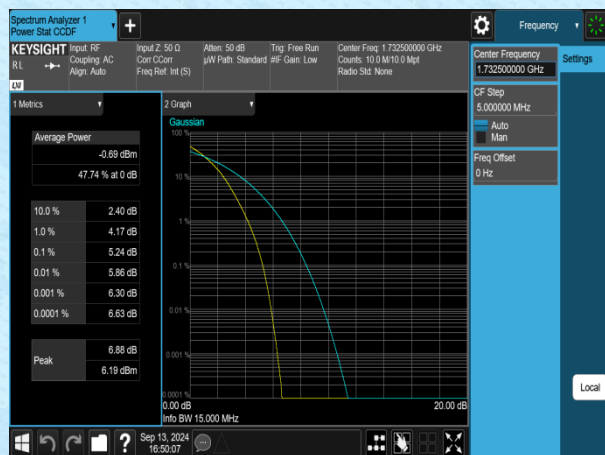
Band4-15MHz-QPSK-20175-1RB#0-PASS
