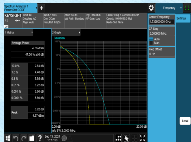
Band4-1.4MHz-QPSK-20175-6RB#0-PASS
