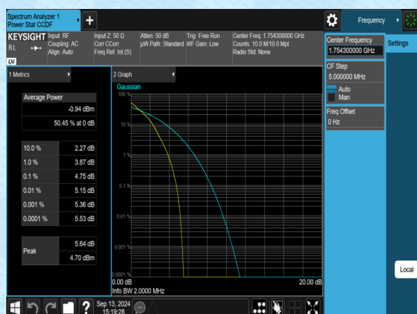
Band4-1.4MHz-QPSK-20393-1RB#0-PASS
