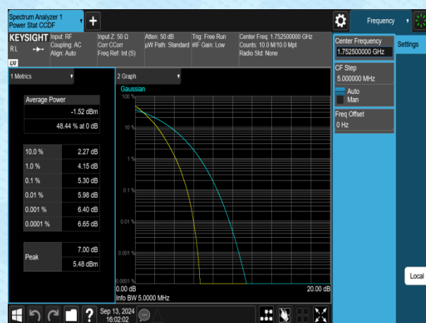
Band4-5MHz-QPSK-20375-25RB#0-PASS
