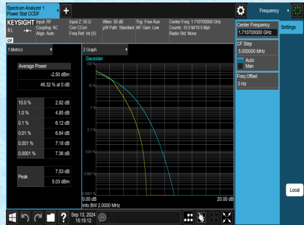
Band4-1.4MHz-16QAM-19957-6RB#0-PASS
