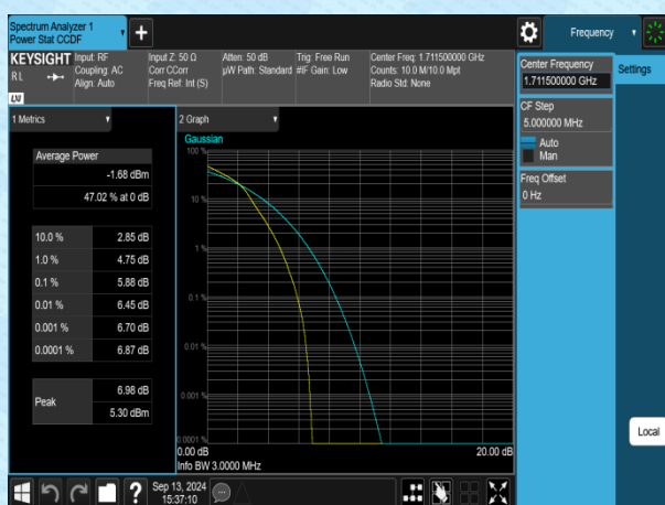
Band4-3MHz-16QAM-19965-1RB#0-PASS
