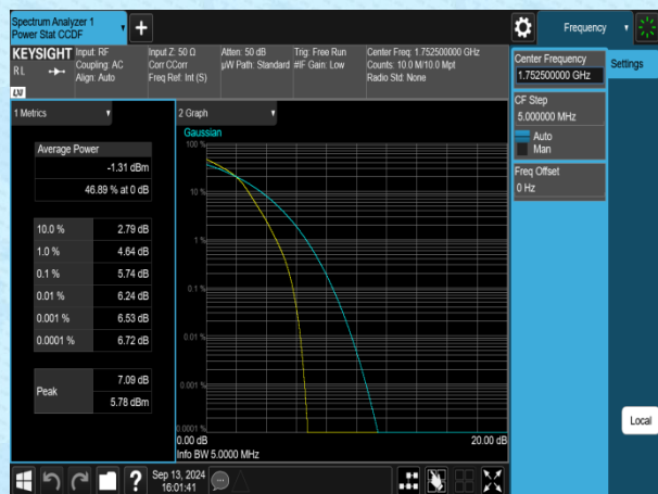
Band4-5MHz-16QAM-20375-1RB#0-PASS
