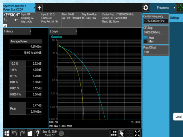
Band4-5MHz-QPSK-20175-1RB#0-PASS
