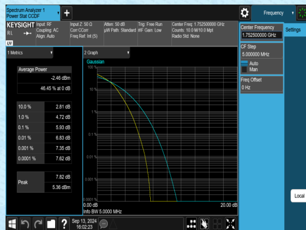
Band4-5MHz-16QAM-20375-25RB#0-PASS
