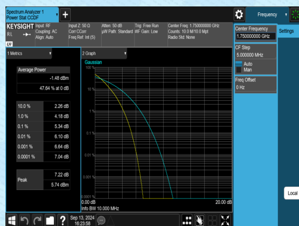
Band4-10MHz-QPSK-20350-50RB#0-PASS
