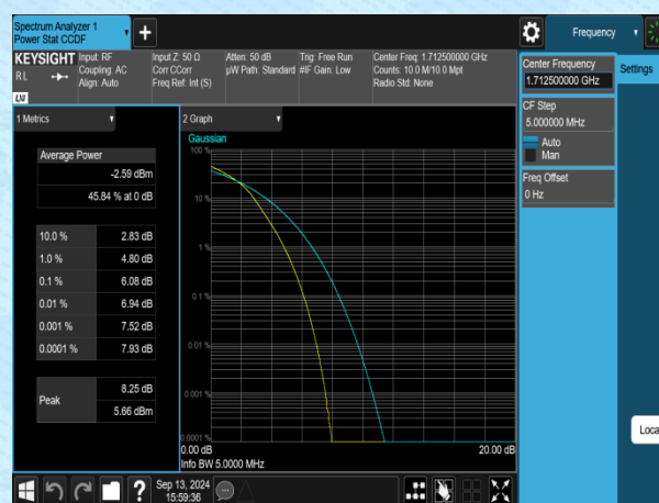
Band4-5MHz-16QAM-19975-25RB#0-PASS
