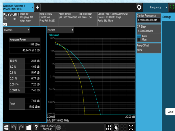
Band4-10MHz-16QAM-20350-1RB#0-PASS
