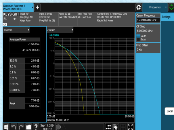
Band4-15MHz-16QAM-20325-1RB#0-PASS
