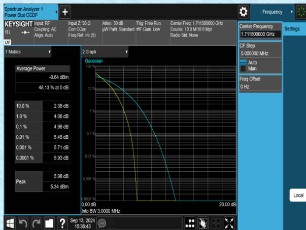
Band4-3MHz-QPSK-19965-1RB#0-PASS
