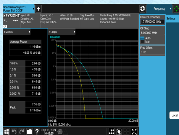
Band4-15MHz-16QAM-20025-1RB#0-PASS
