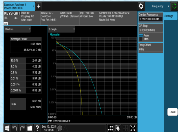
Band4-1.4MHz-QPSK-19957-6RB#0-PASS
