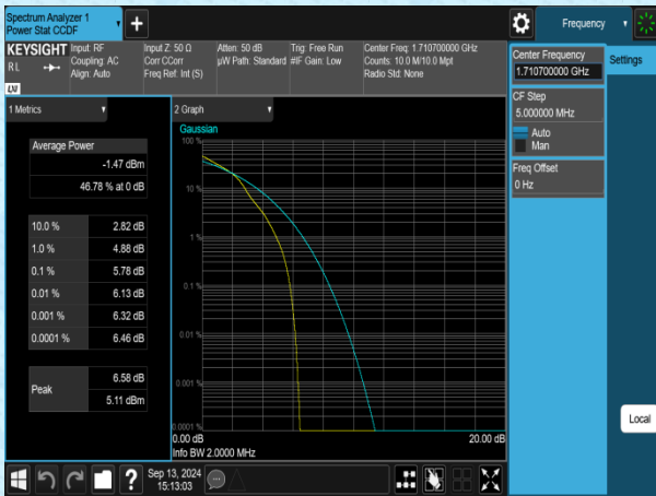
Band4-1.4MHz-16QAM-19957-1RB#0-PASS
