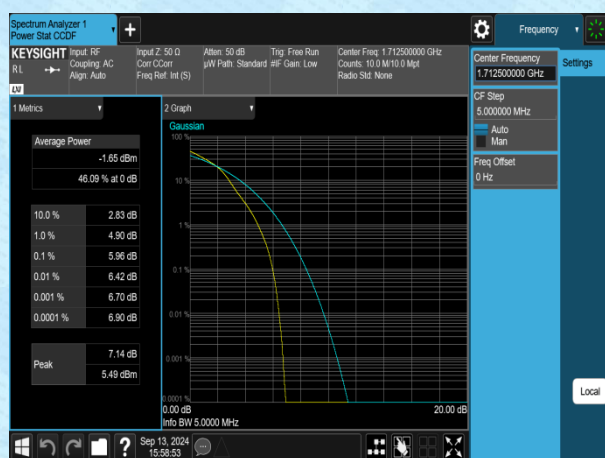
Band4-5MHz-16QAM-19975-1RB#0-PASS
