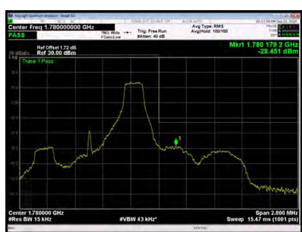
LTE Band 66 QPSK 1.4MHz CH-High, 1 RB
