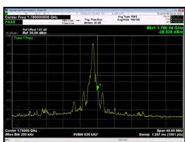
LTE Band 66 64QAM 20MHz CH-High, 1 RB
