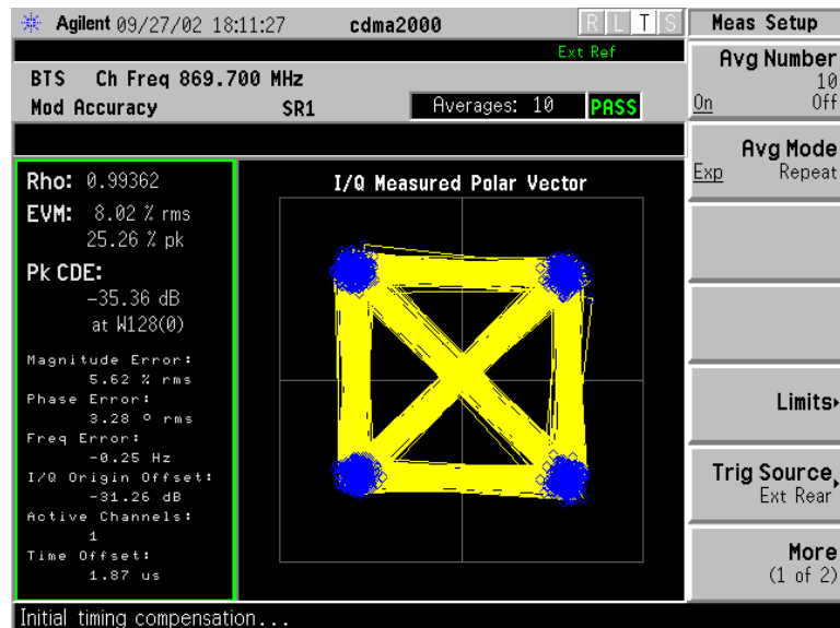
Channel 1013 – 869.7 MHz
