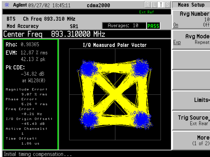
Channel 777 – 893.31 MHz
