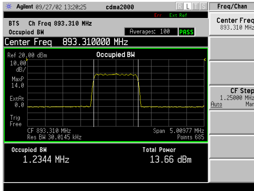
Channel 777 – 893.31 MHz
