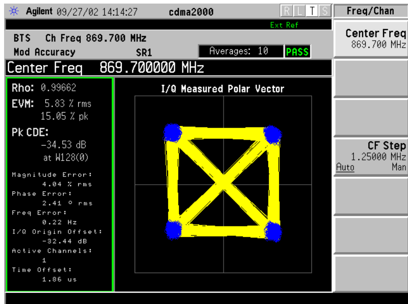
Channel 1013 – 869.7 MHz
