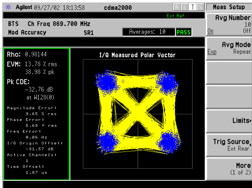
Channel 1013 – 869.7 MHz
