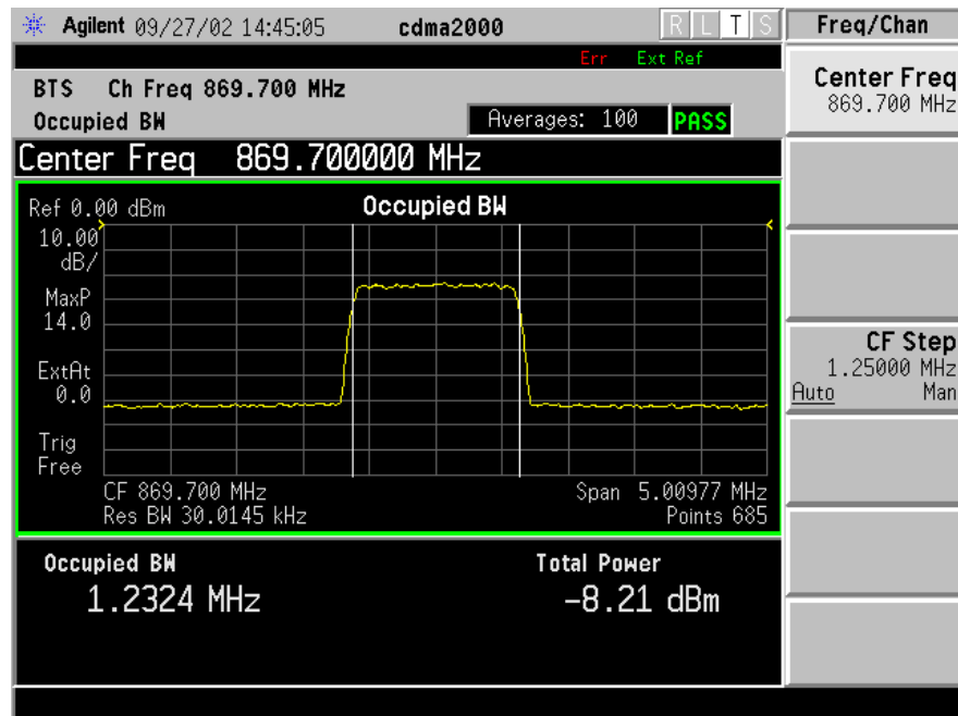
Channel 1013 – 869.7 MHz
