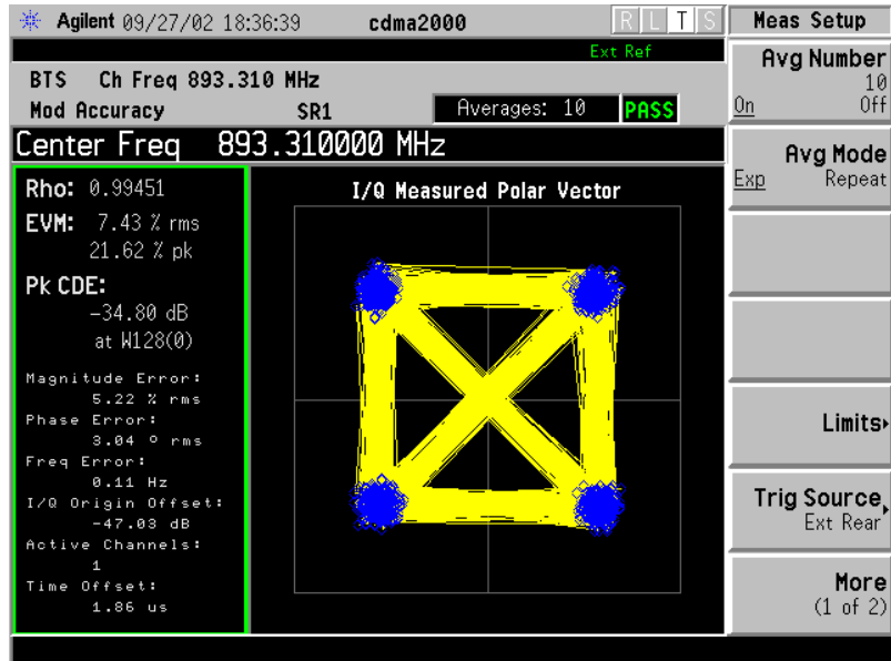
Channel 777 – 893.31 MHz
