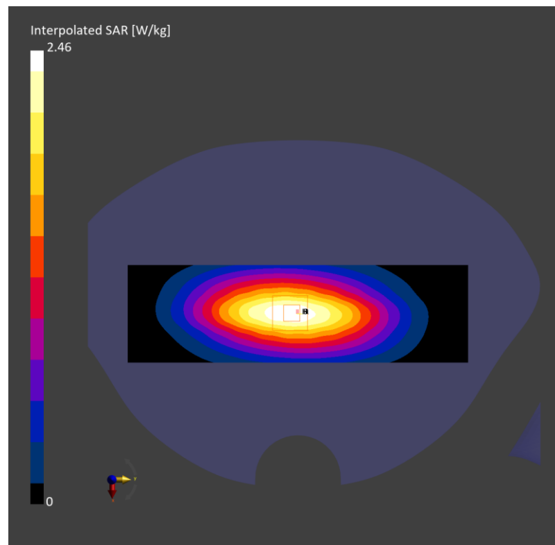
Fig.B.1. Validation 750MHz 250mW
