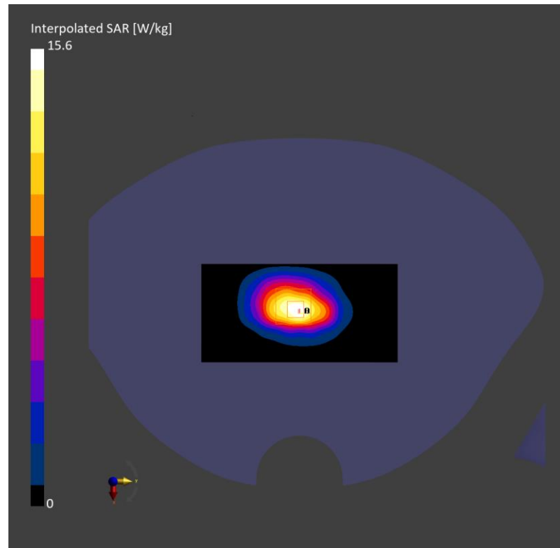
Fig.B.4. Validation 1900MHz 250mW
