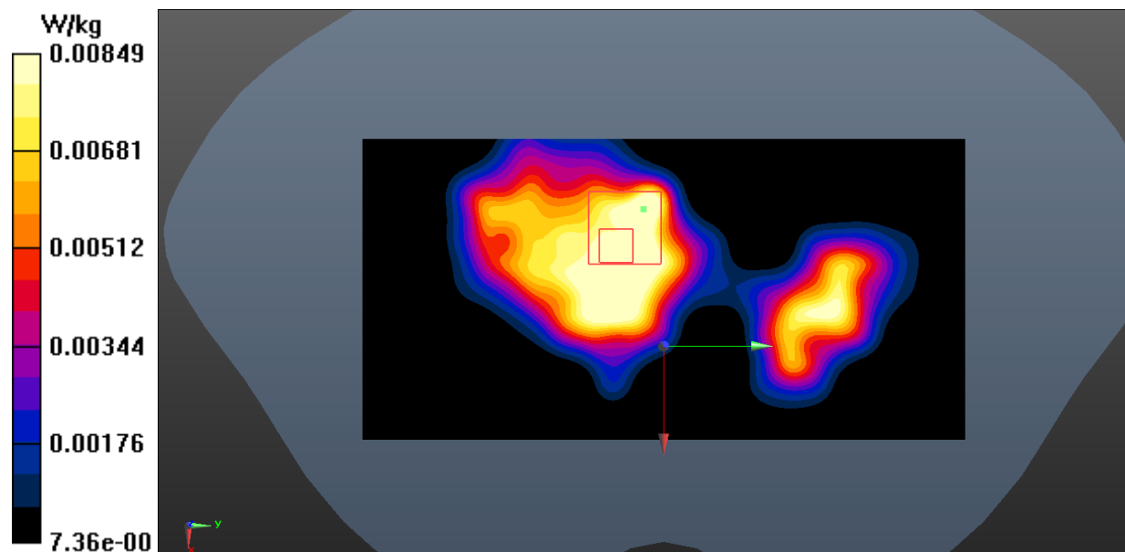
Fig.24 Bluetooth Body
