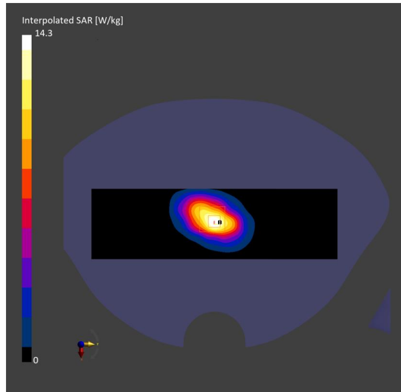
Fig.B.3. Validation 1750MHz 250mW
