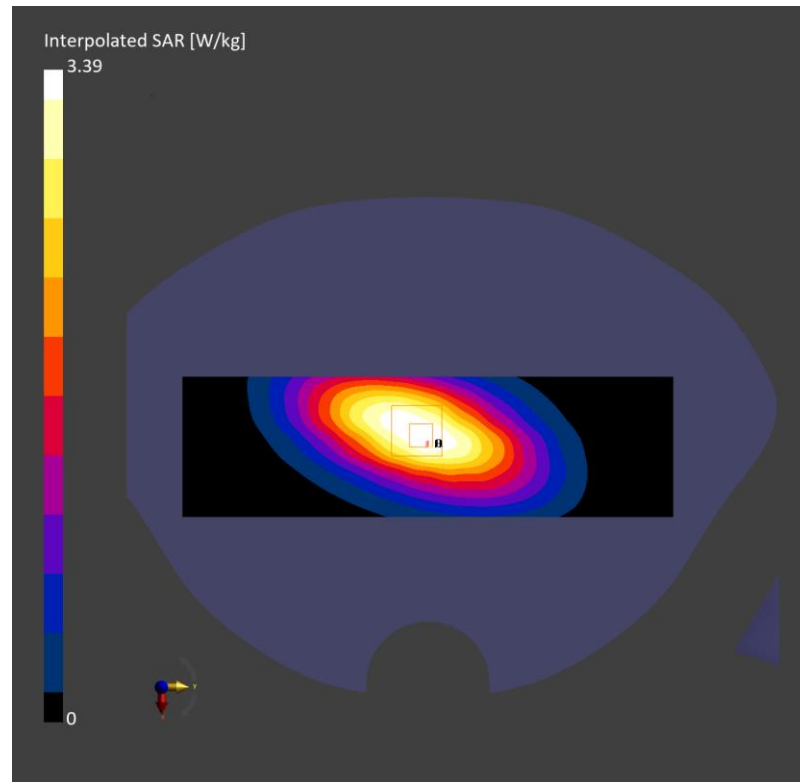
Fig.B.2. Validation 835MHz 250mW
