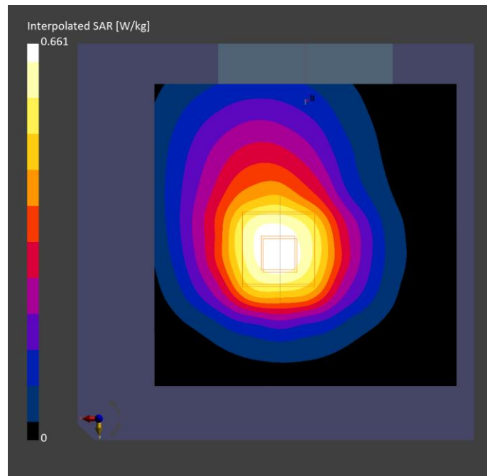
Fig.4 GSM 1900 Body
