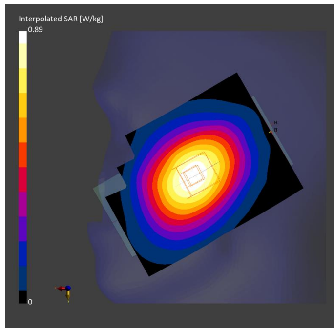
Fig.1 GSM 850 Head
