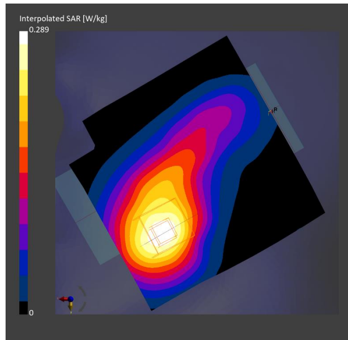
Fig.3 GSM 1900 Head
