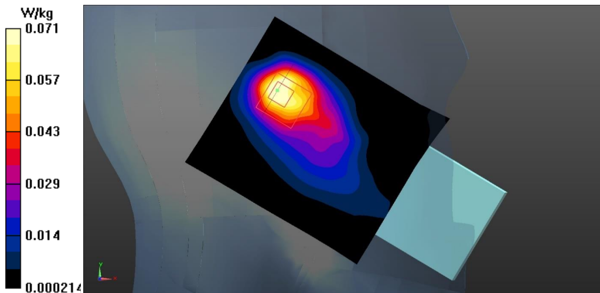
Fig.23 Bluetooth Head
