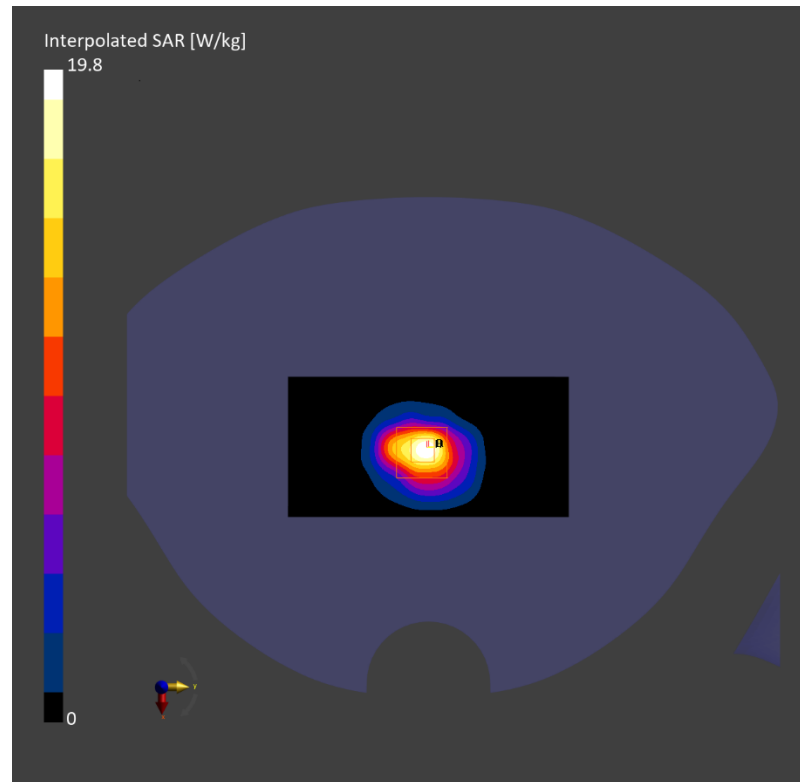
Fig.B.6. Validation 2550MHz 250mW
