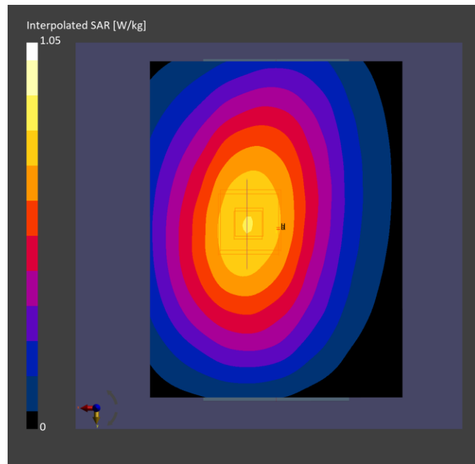
Fig.2 GSM 850 Body
