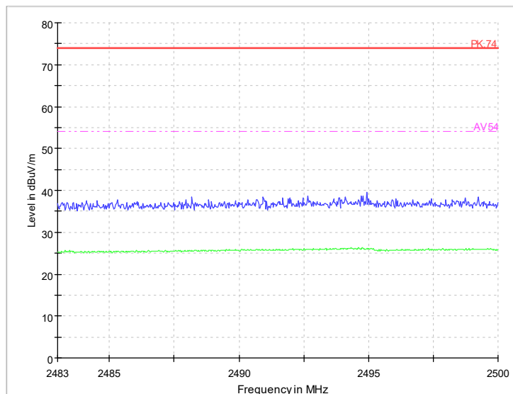
Radiated Emission Band Edge Channel No.:39 Test Mode: GFSK (LE) Polarization: H
