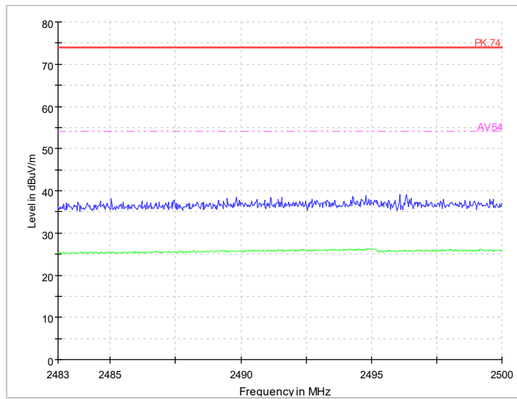
Radiated Emission Band Edge Channel No.:39 Test Mode: GFSK (LE) Polarization: V
