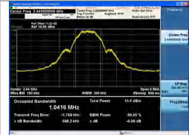
Test Mode:Coded 500K 2440MHz
