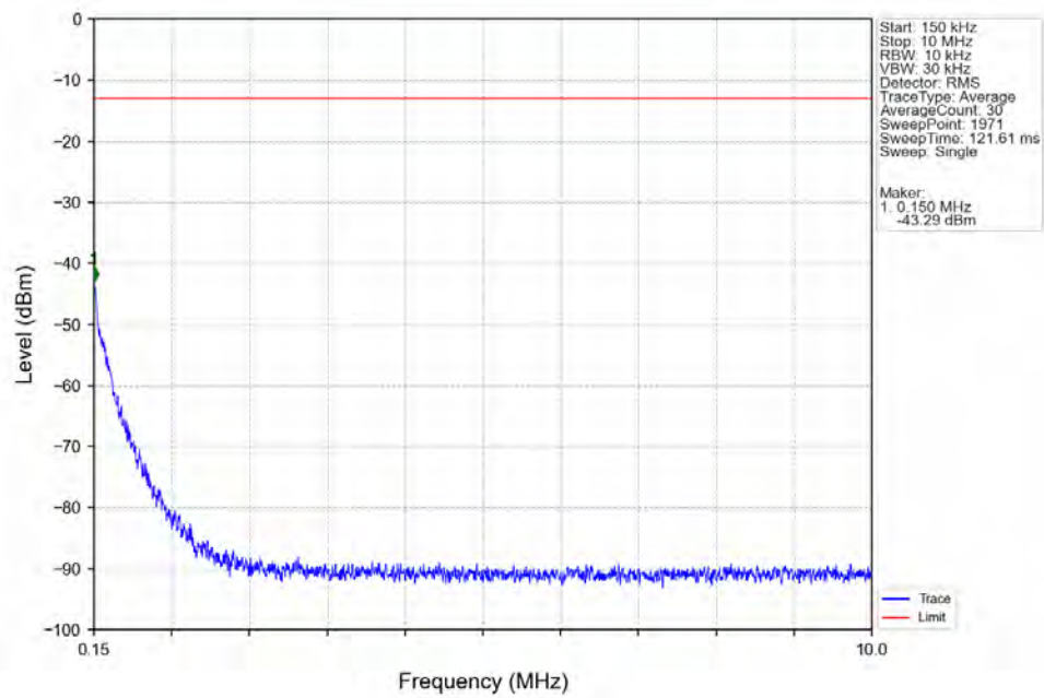
Band5_5MHz_16QAM_HCH_846.5MHz_RB_1_0_NTNV
