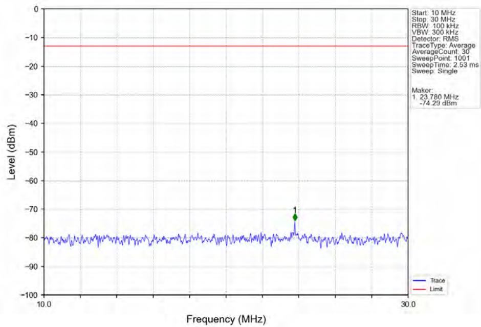
Band5_5MHz_64QAM_LCH_826.5MHz_RB_1_0_NTNV
