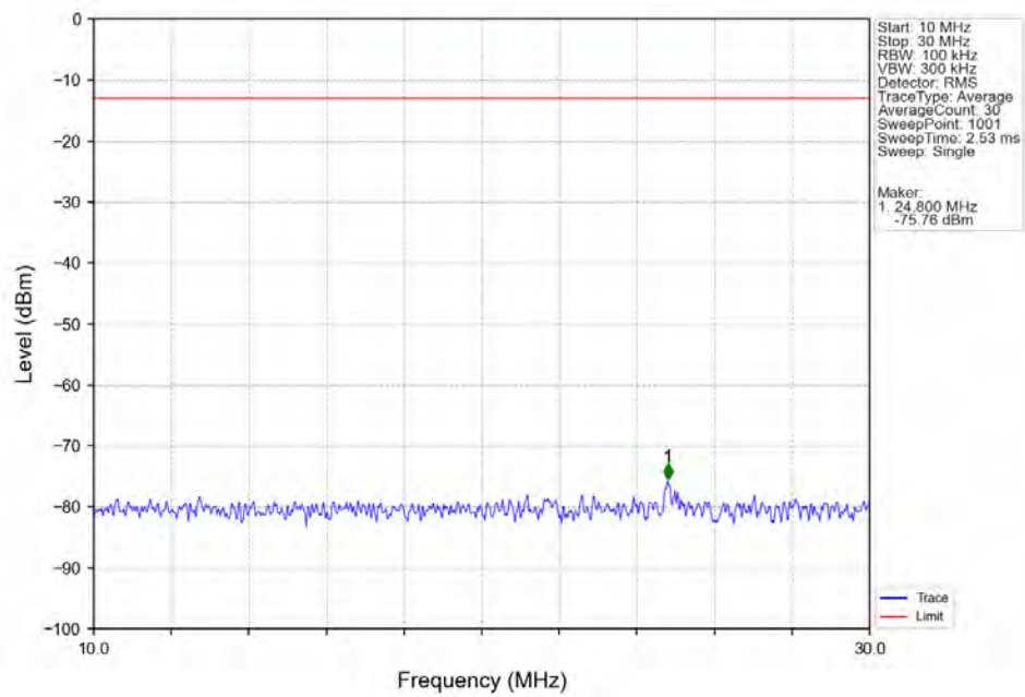
Band5_10MHz_64QAM_LCH_829MHz_RB_1_0_NTNV
