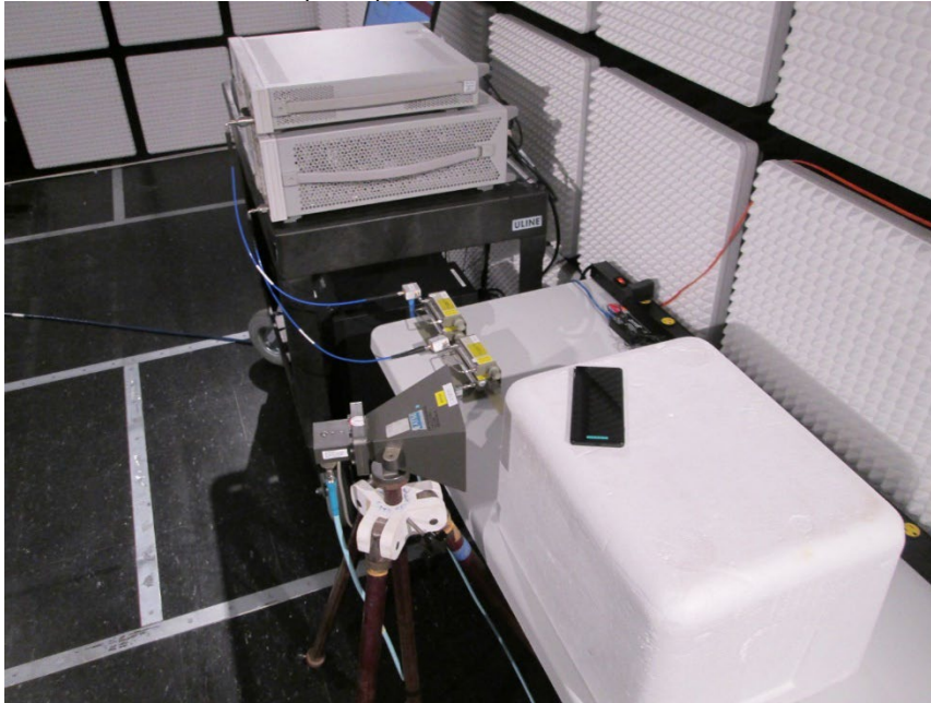
RADIATED PHOTO (DFS)
