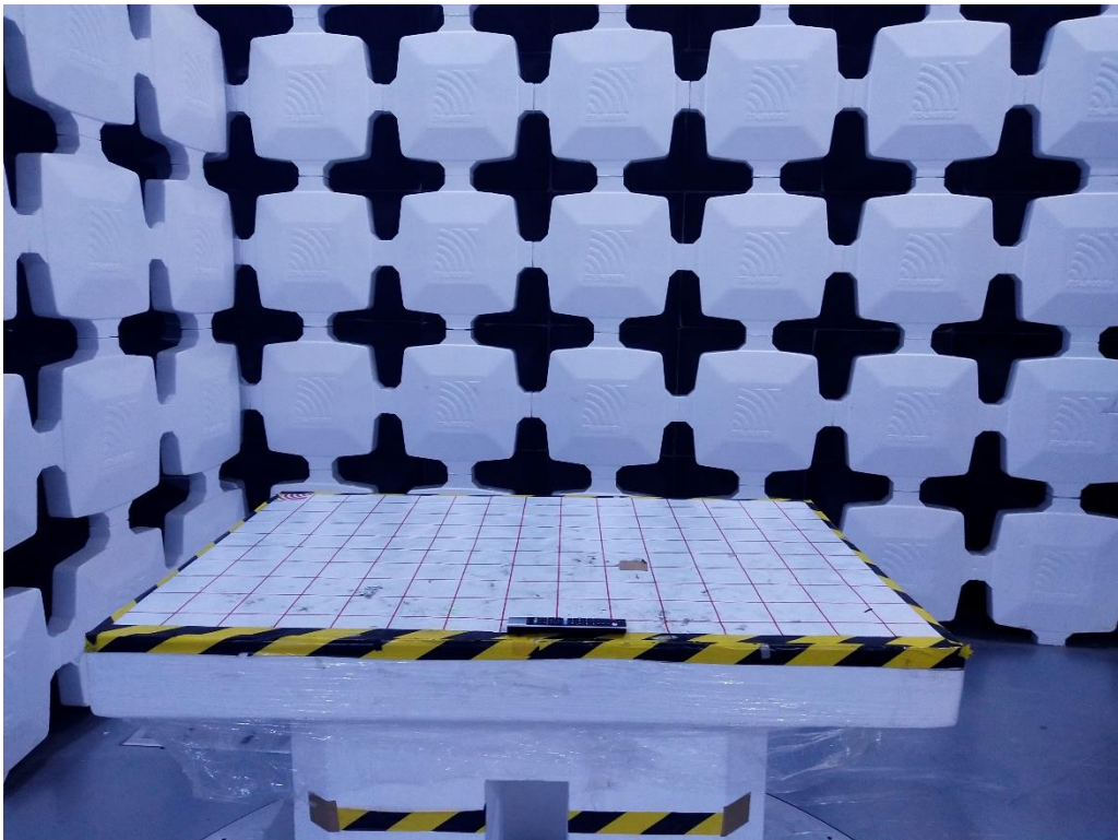
(The EUT placed at the center of turntable)
