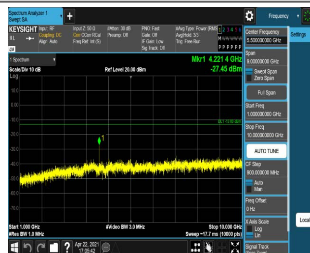
Band5-10MHz-QPSK-20450-1RB#0-Range2:1000~100
