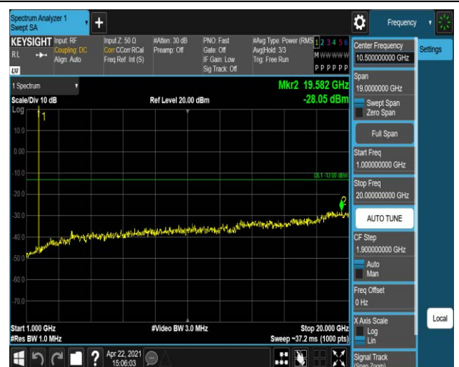
Band4-1.4MHz-QPSK-20393-1RB#0-Range2:1000~20
