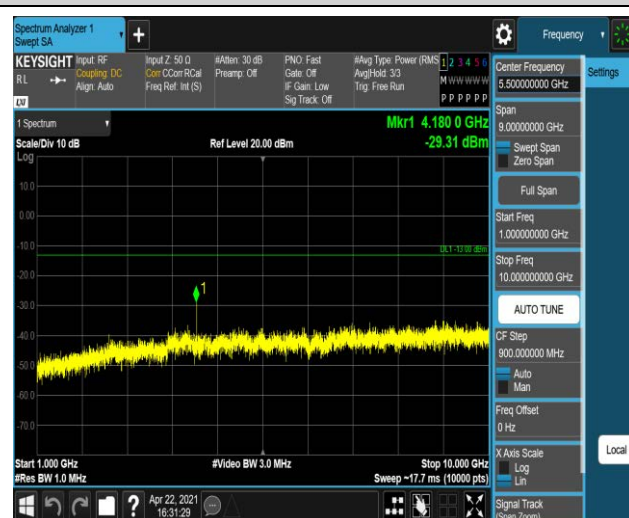
Band5-1.4MHz-QPSK-20643-1RB#0-Range2:1000~10
