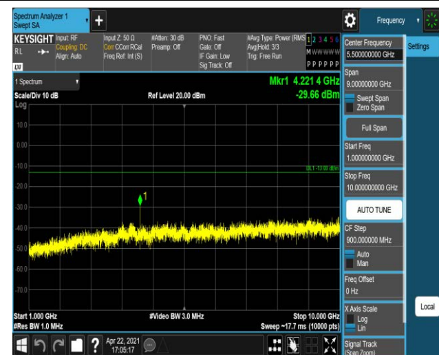
Band5-5MHz-16QAM-20425-1RB#0-Range2:1000~100
