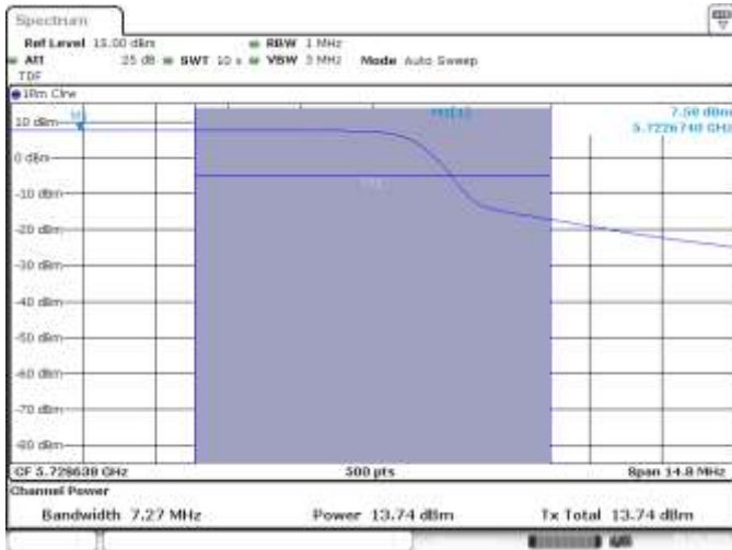
MIMO A, HE0, 802.11ax20, Overlapped CH144
