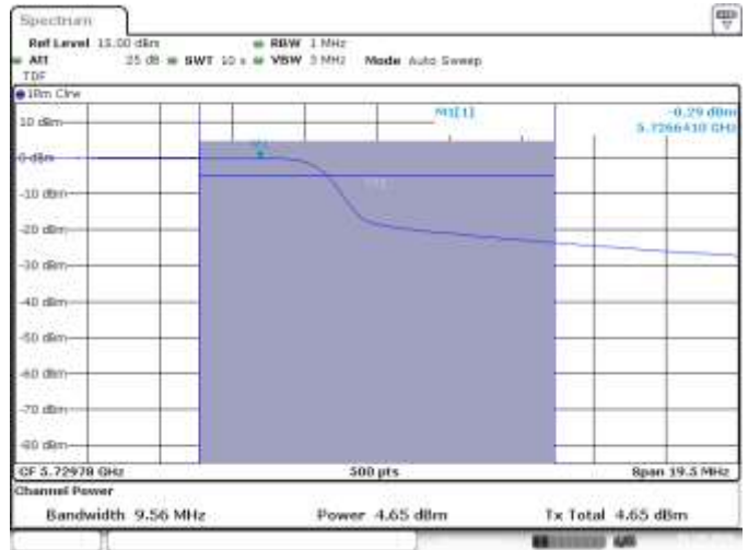
SISO B, VHT0, 802.11ac80, Overlapped CH138
