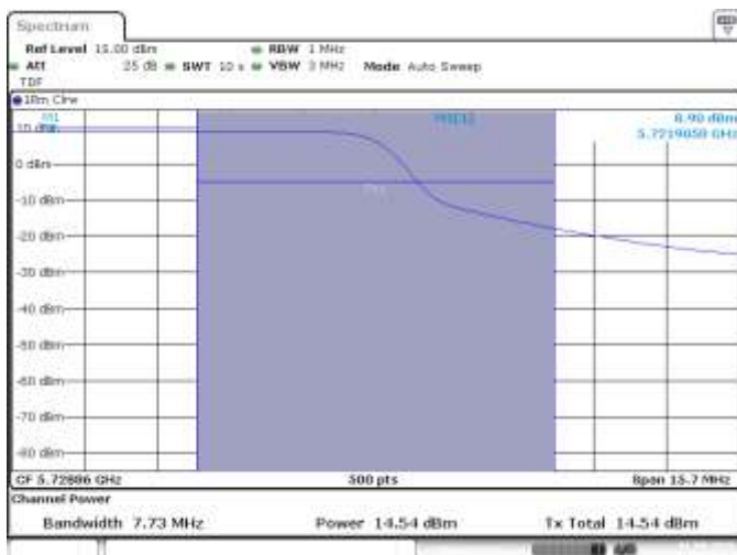
SISO A, CH155, 802.11ax80, HE0
