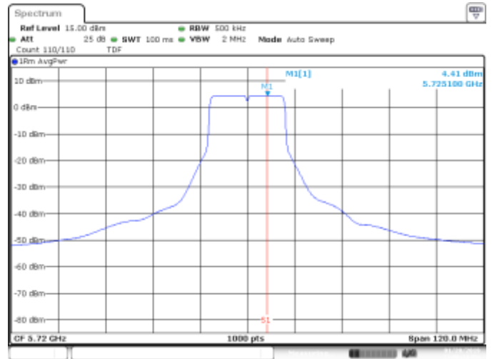
MIMO B, HE0, 802.11ax20, Overlapped CH144
