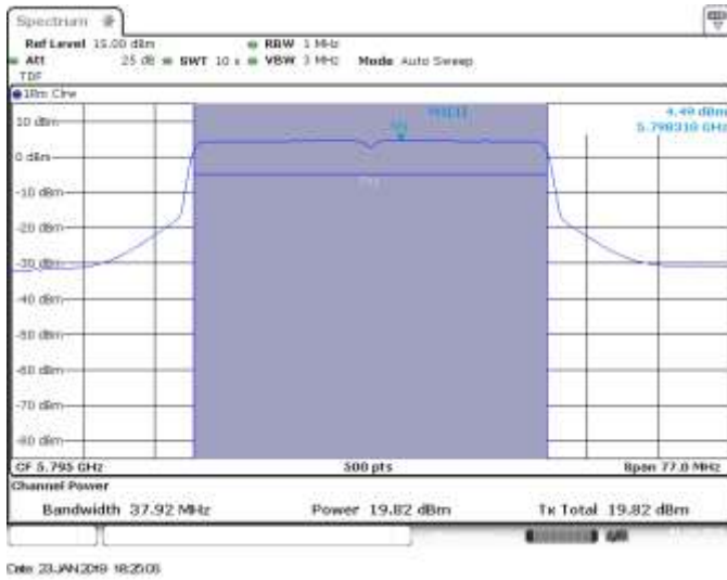
MIMO A, CH159, 802.11ax40, HE0
