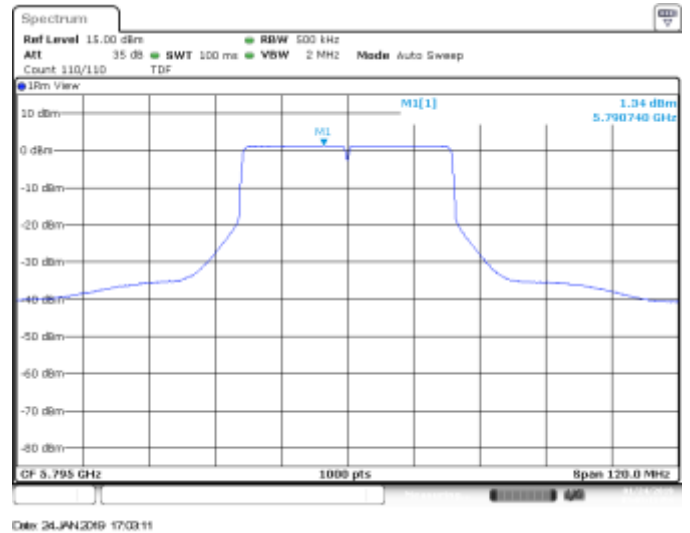
MIMO B, CH159, 802.11ax40, HE0
