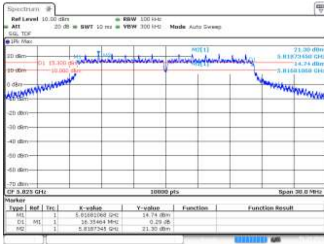
SISO B, CH165, 802.11a, 6Mbps, 6dB
