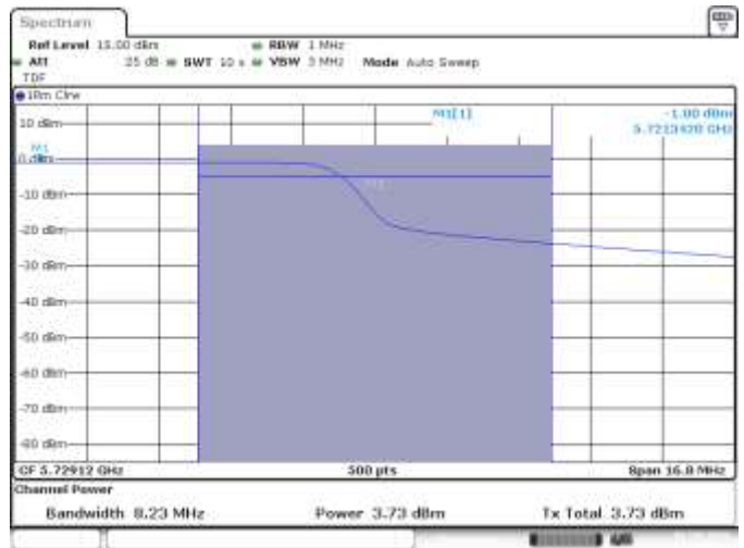
MIMO B, VHT0, 802.11ac80, Overlapped CH138
