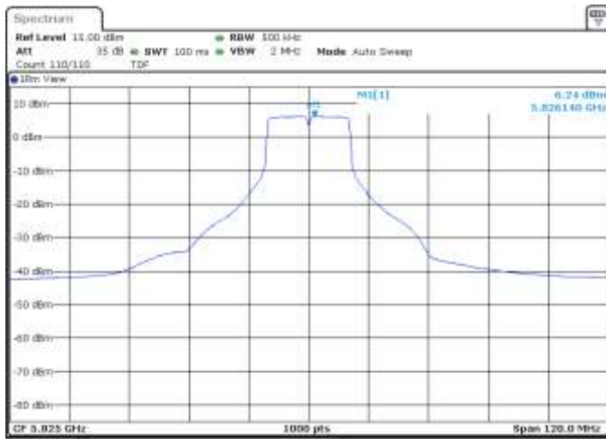
SISO A, CH165, 802.11a, 6Mbps
