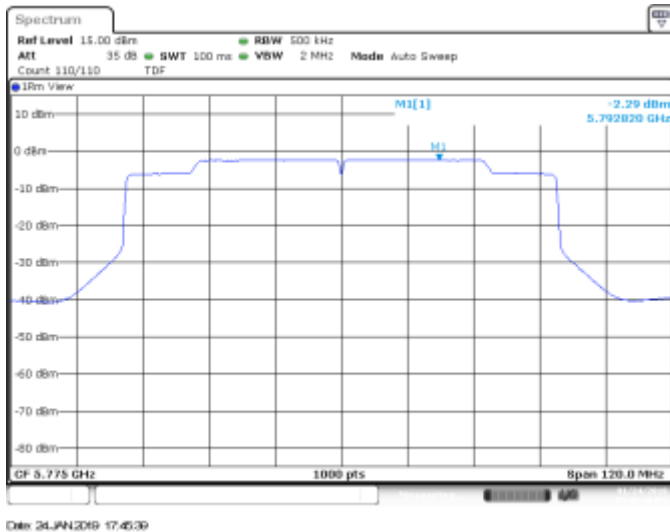
SISO A, CH155, 802.11ax80, HE0
