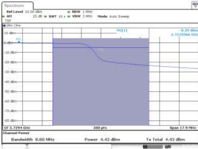
SISO A, VHT0, 802.11ac80, Overlapped CH138
