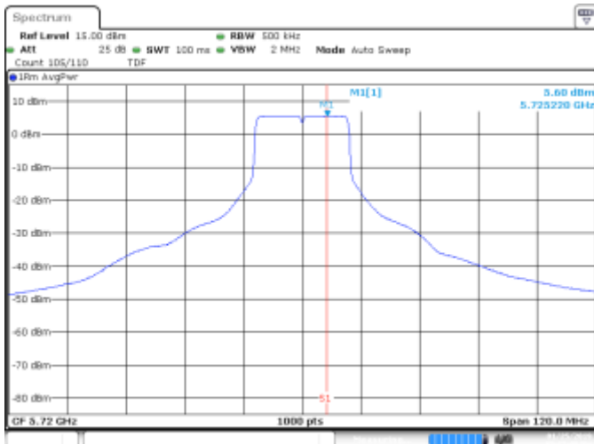
SISO A, HE0, 802.11ax20, Overlapped CH144
