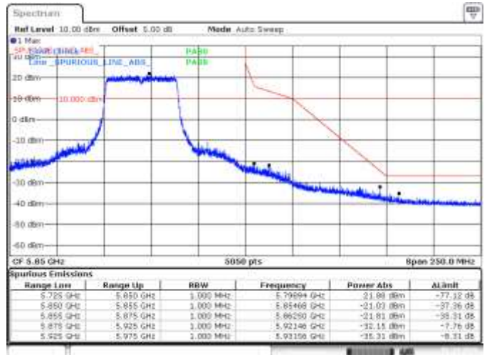
MIMO B, 802.11ax40, HE0, CH159, BE High Peak
