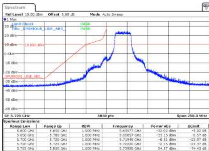
SISO B, 802.11a, 6Mbps, CH149, BE Low Peak
