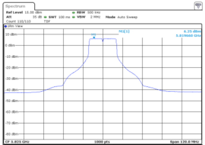
SISO B, CH165, 802.11a, 6Mbps
