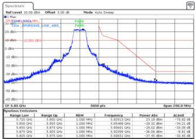
SISO A, 802.11a, 6Mbps, CH165, BE High Peak
