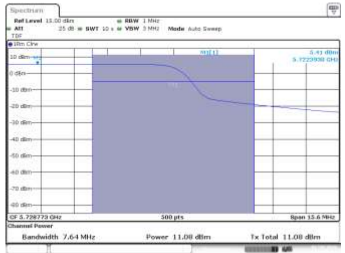
SISO B, HE0, 802.11ax40, Overlapped CH142
