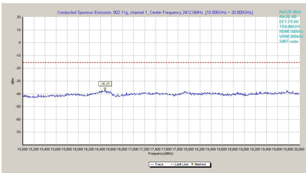
Fig.A.6.1.47 Transmitter Spurious Emission - Conducted (802.11g, Ch1, 15 GHz-20 GHz)
