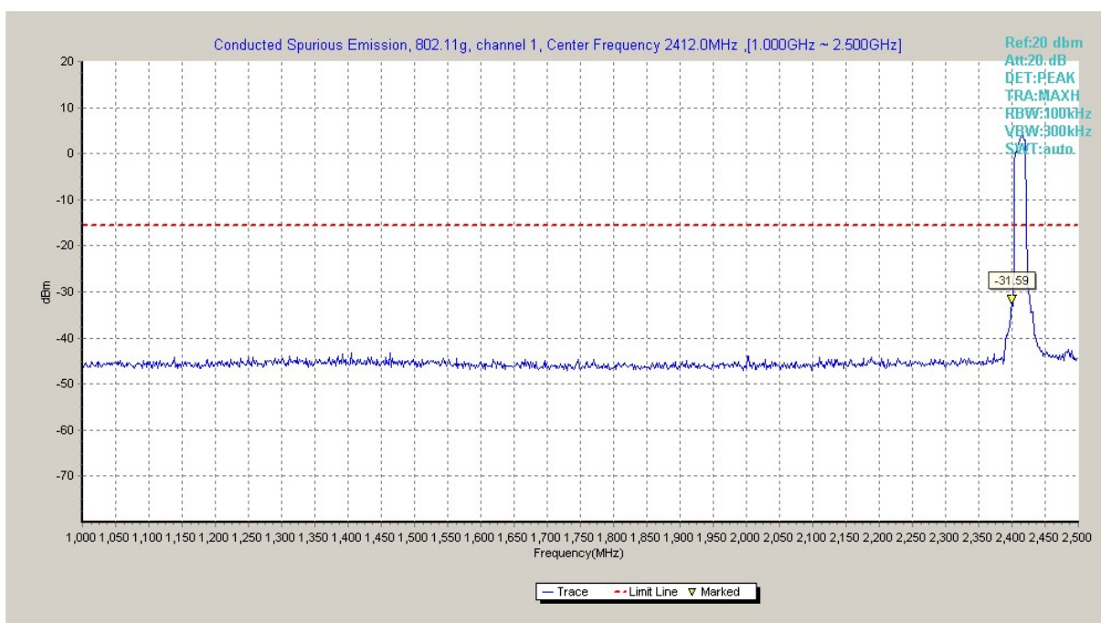
Fig.A.6.1.43 Transmitter Spurious Emission - Conducted (802.11g, Ch1, 1 GHz-2.5 GHz)
