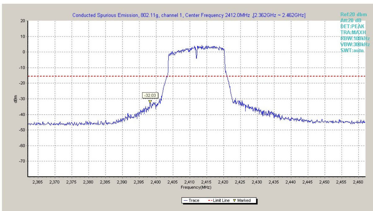
Fig.A.6.1.41 Transmitter Spurious Emission - Conducted (802.11g, Ch1, Center Frequency)
