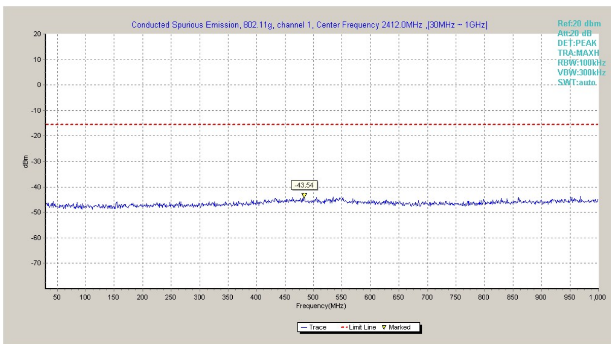
Fig.A.6.1.42 Transmitter Spurious Emission - Conducted (802.11g, Ch1, 30 MHz-1 GHz)
