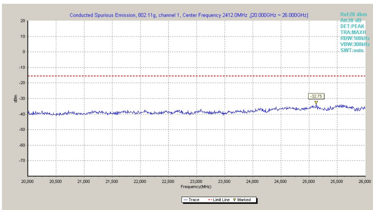
Fig.A.6.1.48 Transmitter Spurious Emission - Conducted (802.11g, Ch1, 20 GHz-26 GHz)
