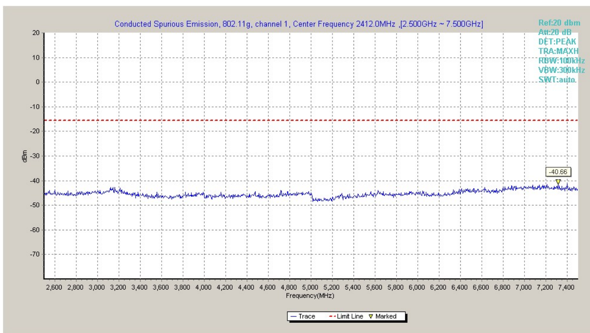
Fig.A.6.1.44 Transmitter Spurious Emission - Conducted (802.11g, Ch1, 2.5 GHz-7.5 GHz)
