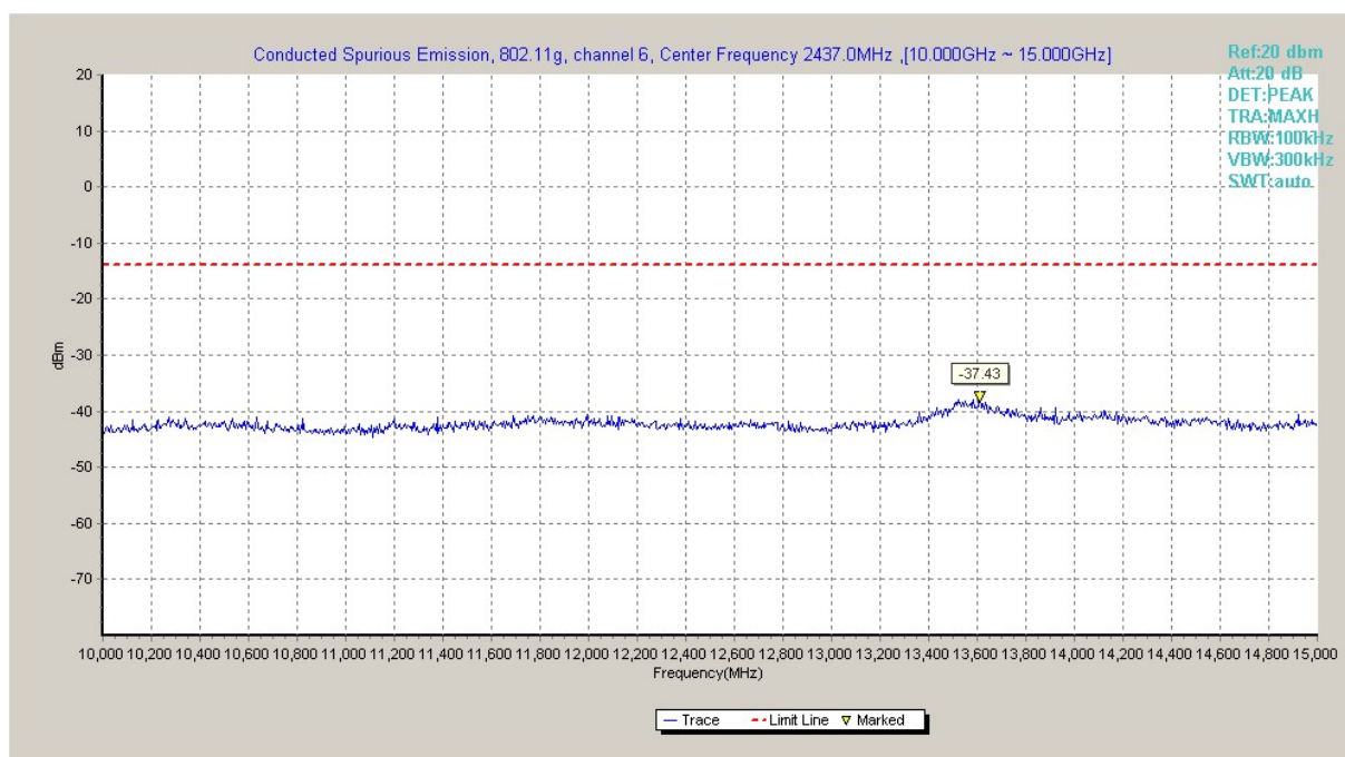
Fig.A.6.1.54 Transmitter Spurious Emission - Conducted (802.11g, Ch6, 10 GHz-15 GHz)
