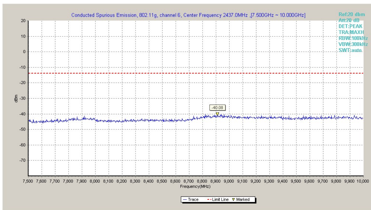
Fig.A.6.1.53 Transmitter Spurious Emission - Conducted (802.11g, Ch6, 7.5 GHz-10 GHz)
