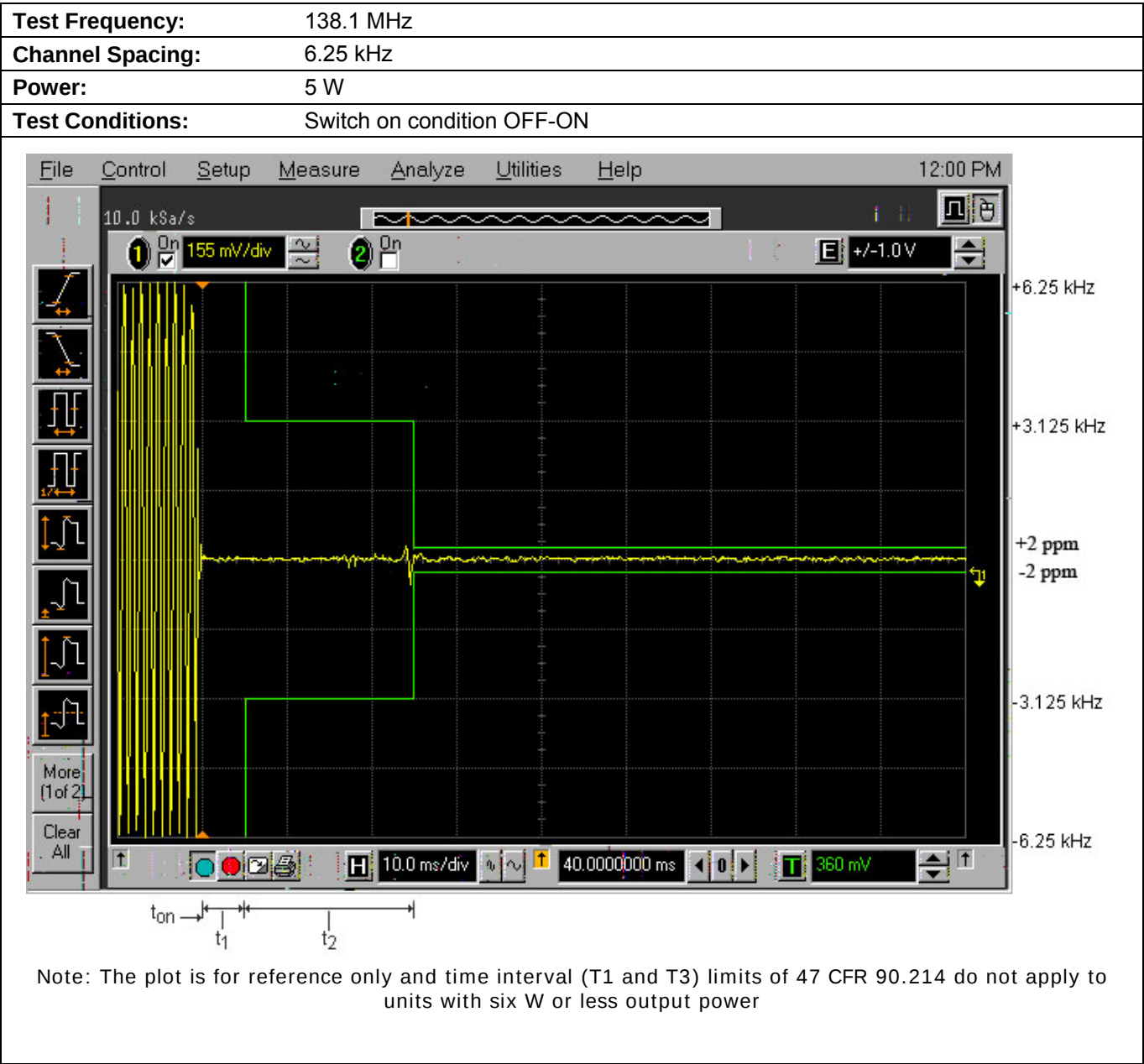
Plot 5.12.4.5. Transient Frequency Behavior for 6.25 kHz Channel Spacing
