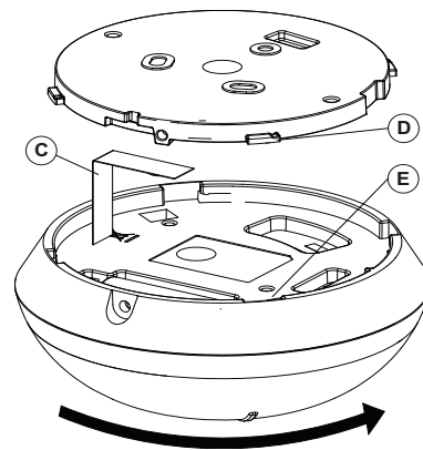
Figure 5. Attaching the detector
