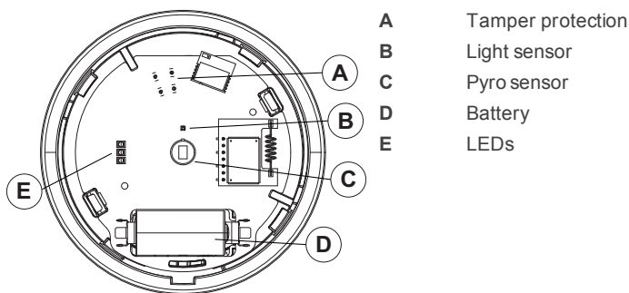
Figure 1. Internal view
