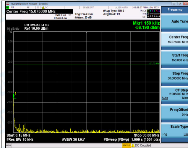
Band12_10MHz_16QAM_23060_1RB#0_0.15~30_0.15~3
