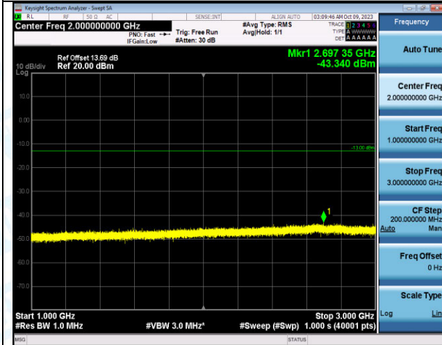
Band12_10MHz_16QAM_23060_1RB#0_1000~3000_1000~3000
