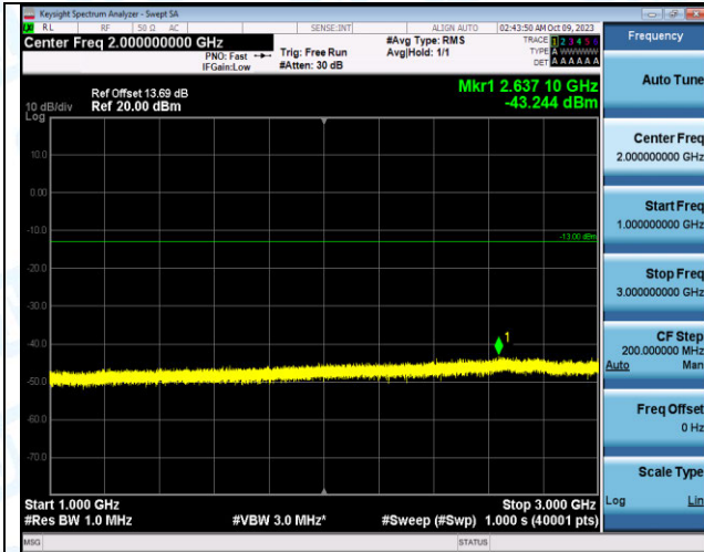
Band12_5MHz_16QAM_23035_25RB#0_1000~3000_100 0~3000
