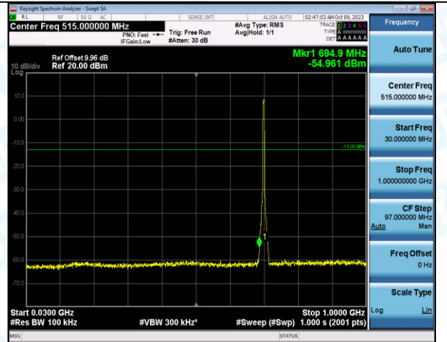
Band12_5MHz_16QAM_23095_25RB#0_30~1000_30~10
