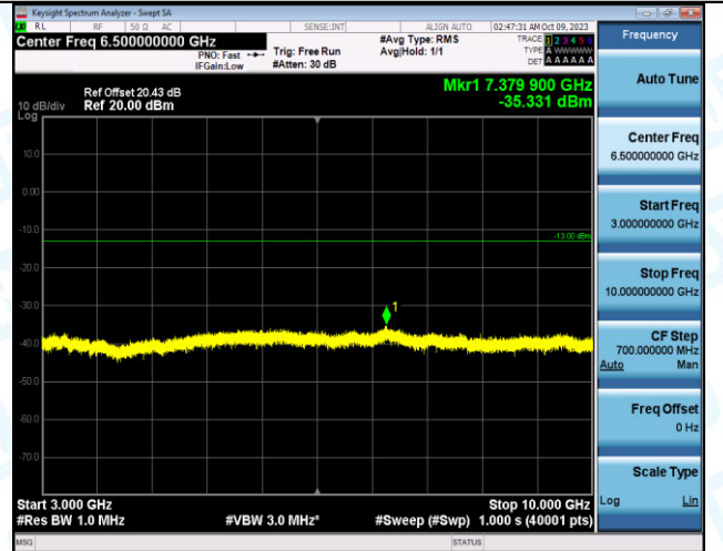
Band12_5MHz_16QAM_23095_25RB#0_3000~10000_3000~10000
