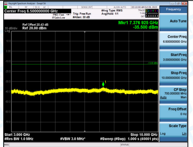
Band12_10MHz_16QAM_23060_1RB#0_3000~10000_3000~10000
