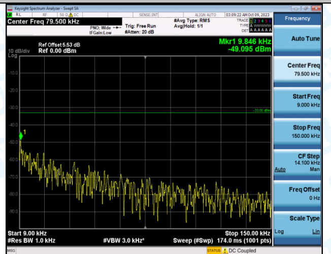
Band12_10MHz_16QAM_23060_1RB#0_0.009~0.15_0.00 9~0.15
