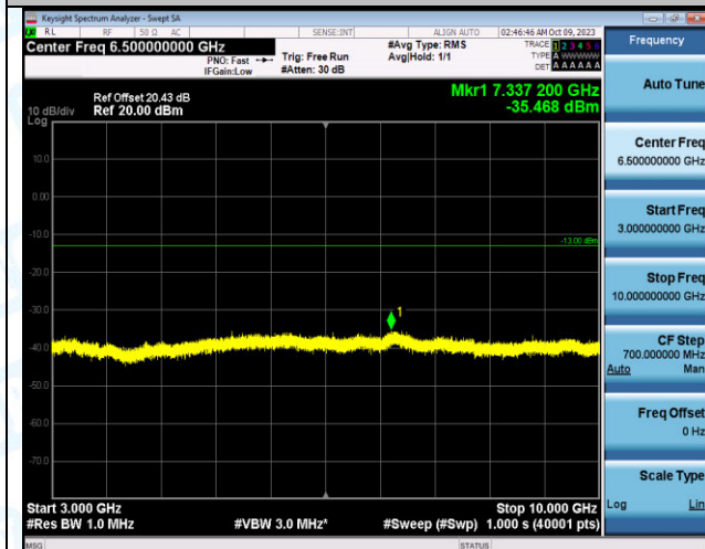
Band12_5MHz_QPSK_23095_25RB#0_3000~10000_300 0~10000
