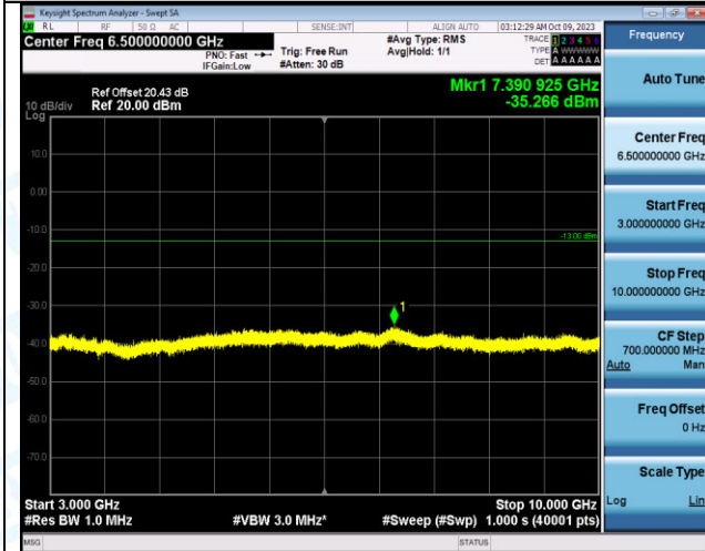
Band12_10MHz_QPSK_23060_1RB#49_3000~10000_3000~10000
