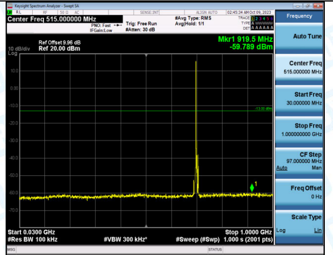
Band12_5MHz_16QAM_23095_1RB#0_30~1000_30~1000 0
