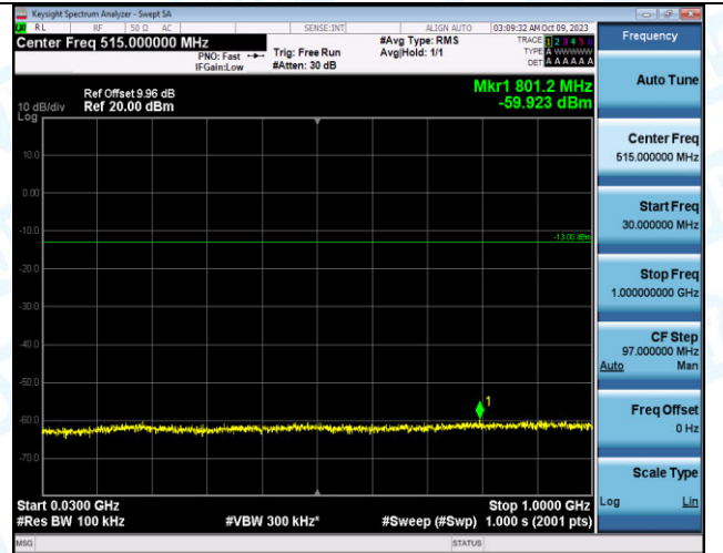
Band12_10MHz_16QAM_23060_1RB#0_30~1000_30~10
