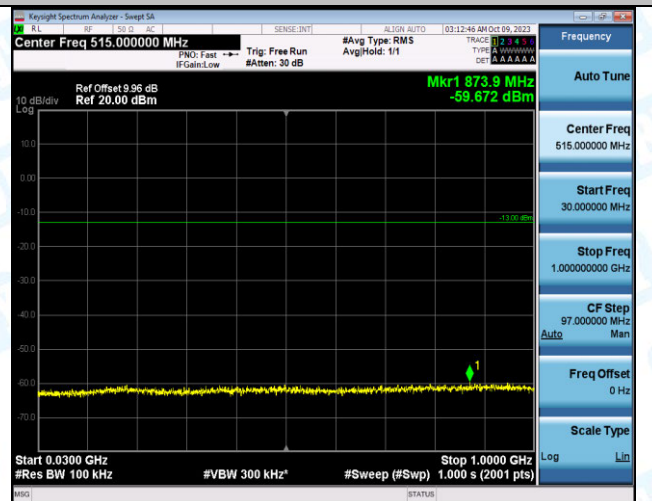
Band12_10MHz_16QAM_23060_1RB#49_30~1000_30~1000
