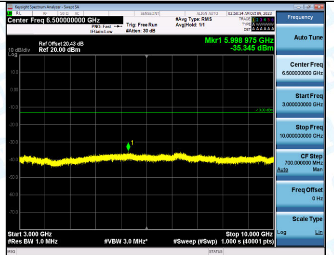
Band12_5MHz_16QAM_23155_25RB#0_3000~10000_30 00~10000
