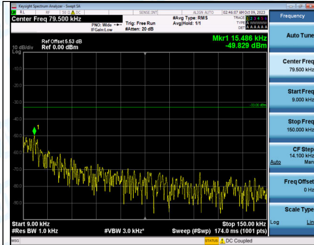
Band12_5MHz_QPSK_23095_25RB#0_0.009~0.15_0.00 9~0.15
