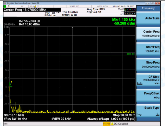
Band12_10MHz_QPSK_23060_1RB#0_0.15~30_0.15~30
