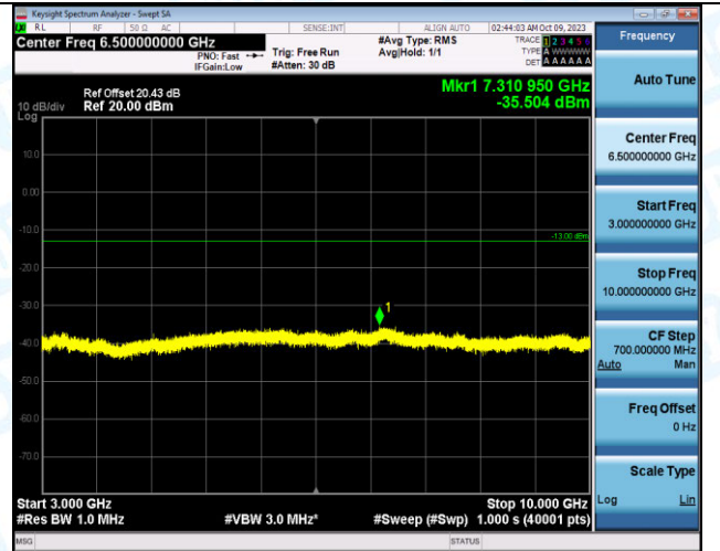
Band12_5MHz_16QAM_23035_25RB#0_3000~10000_30 00~10000
