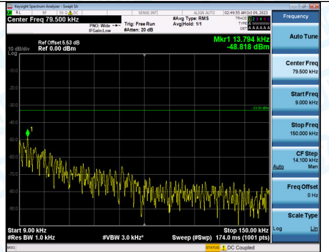
Band12_5MHz_16QAM_23155_25RB#0_0.009~0.15_0.00 9~0.15
