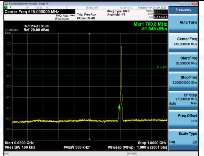
Band12_5MHz_16QAM_23155_25RB#0_30~1000_30~10 00
