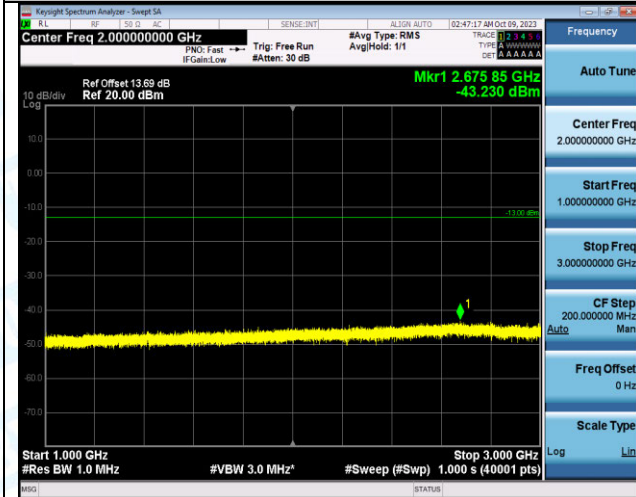
Band12_5MHz_16QAM_23095_25RB#0_1000~3000_1000~3000
