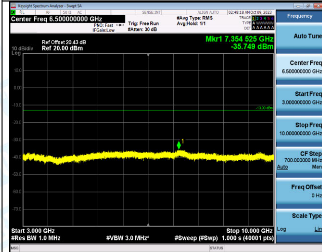
Band12_5MHz_QPSK_23155_1RB#0_3000~10000_3000~10000
