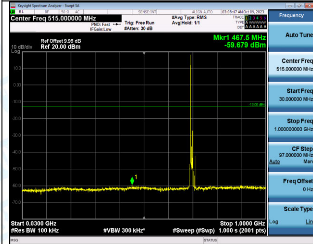
Band12_10MHz_QPSK_23060_1RB#0_30~1000_30~100 0
