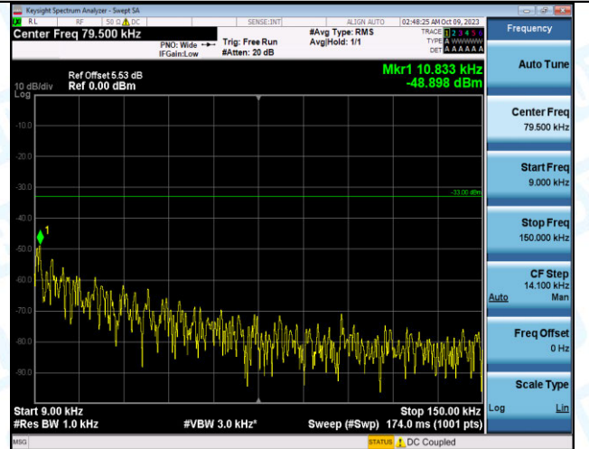
Band12_5MHz_16QAM_23155_1RB#0_0.009~0.15_0.009~0.15
