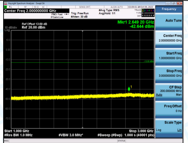
Band12_10MHz_QPSK_23060_1RB#0_1000~3000_1000~3000
