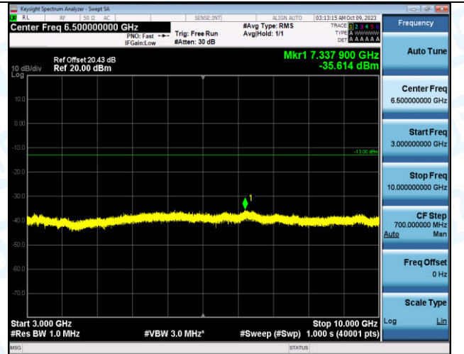
Band12_10MHz_16QAM_23060_1RB#49_3000~10000_3 000~10000
