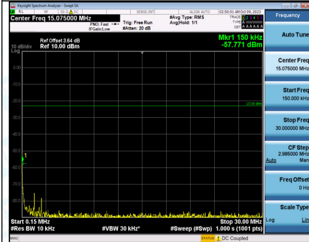
Band12_5MHz_16QAM_23155_25RB#0_0.15~30_0.15~3 0
