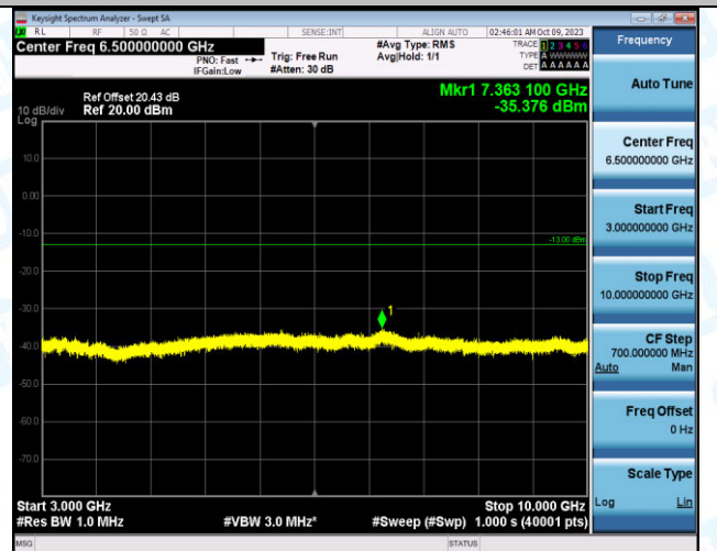
Band12_5MHz_16QAM_23095_1RB#0_3000~10000_300 0~10000
