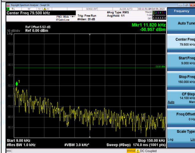
Band12_10MHz_QPSK_23060_1RB#49_0.009~0.15_0.009~0.15
