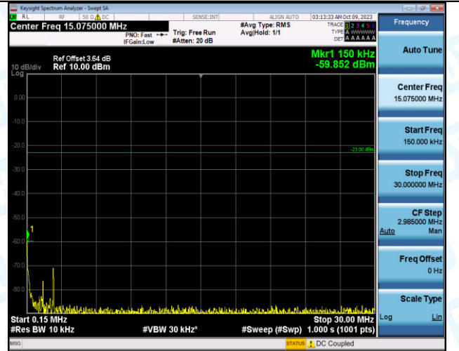
Band12_10MHz_QPSK_23095_1RB#0_0.15~30_0.15~30
