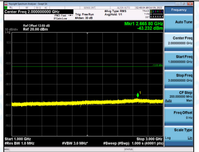
Band12_5MHz_QPSK_23155_1RB#0_1000~3000_1000~3000
