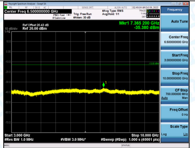
Band12_5MHz_16QAM_23155_1RB#0_3000~10000_300 0~10000
