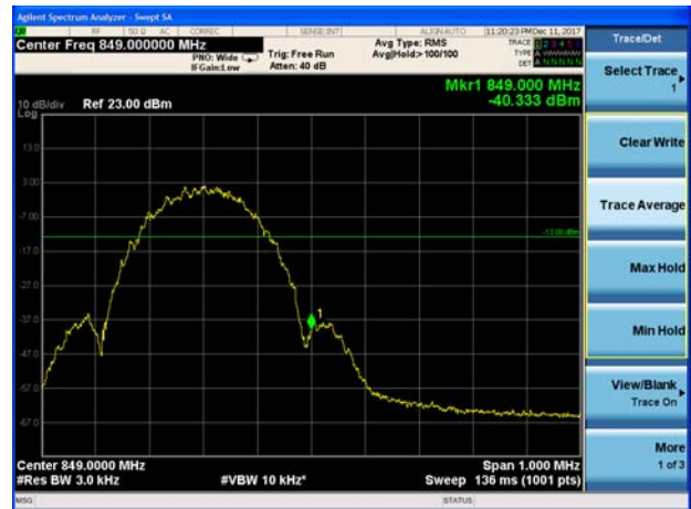
WCDMA Band V CH-High
