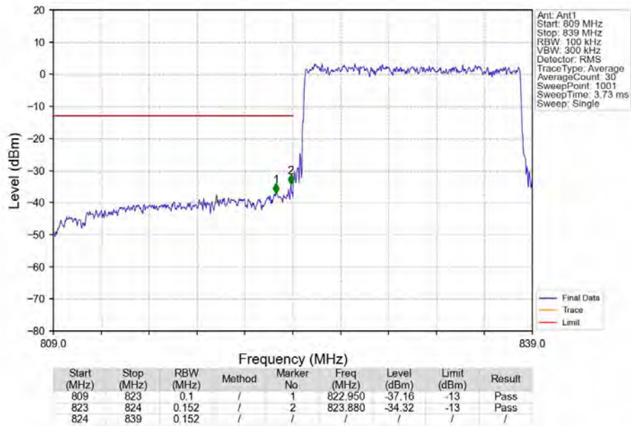
Band26b_15MHz_16QAM_LCH_831.5MHz_RB_75_0_NTNV
