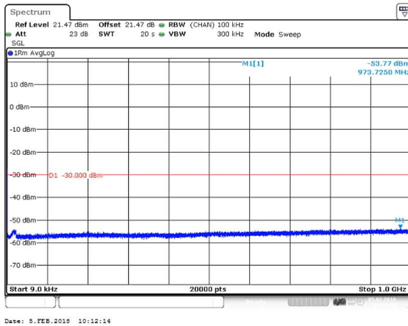
Figure 291 Spurious Emissions (9kHz – 1GHz) – 256QAM (5200.0/ 5220.0/ 5240.0 MHz) (3 X 20MHz Channel BW)
