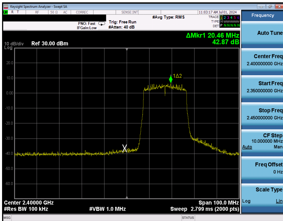
Plot 7-245. Band Edge Plot Antenna WF8 (802.11ax (SU - 2.4GHz) – Ch. 2) – MCS4
