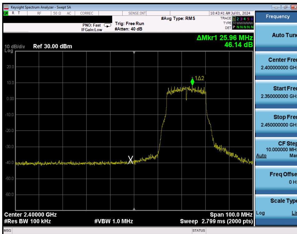
Plot 7-218. Band Edge Plot Antenna WF8 (802.11g – Ch. 3) – 24Mbps
