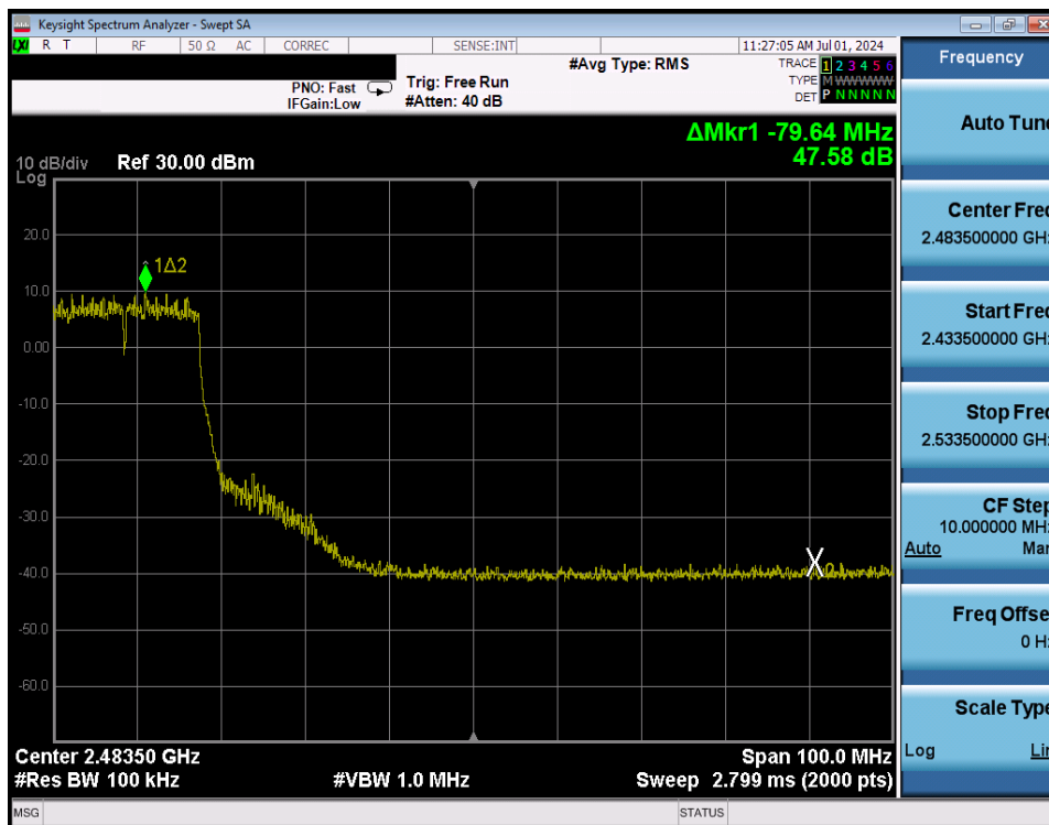
Plot 7-282. Band Edge Plot Antenna WF8 (802.11n (2.4GHz) – Ch. 7) – MCS7
