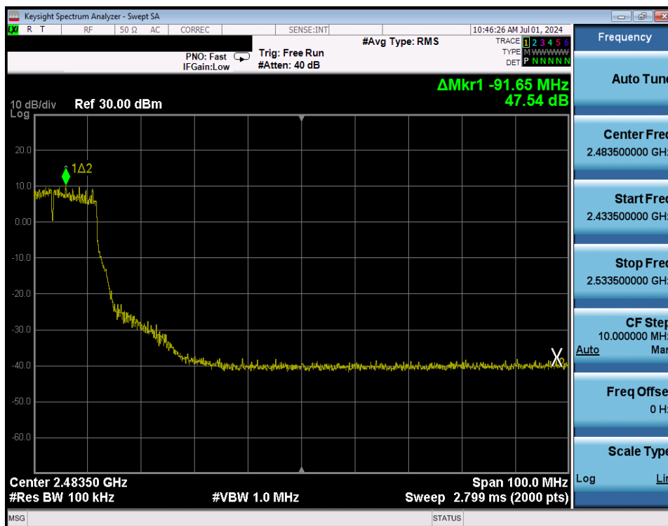
Plot 7-222. Band Edge Plot Antenna WF8 (802.11g – Ch. 6 High) – 24Mbps
