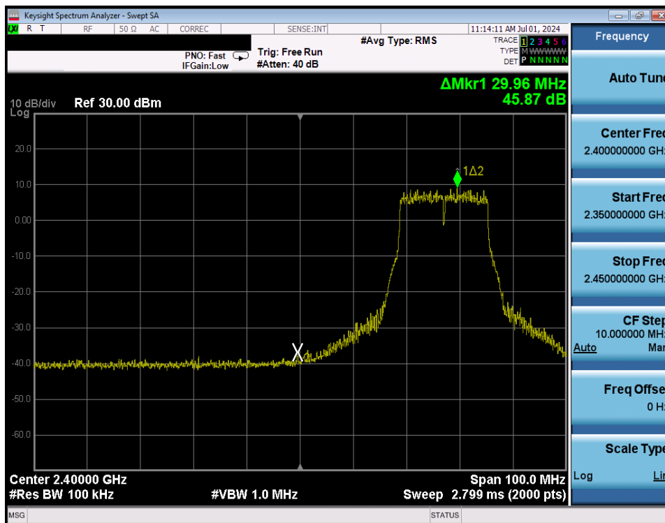
Plot 7-264. Band Edge Plot Antenna WF8 (802.11g – Ch. 4) – 54Mbps
