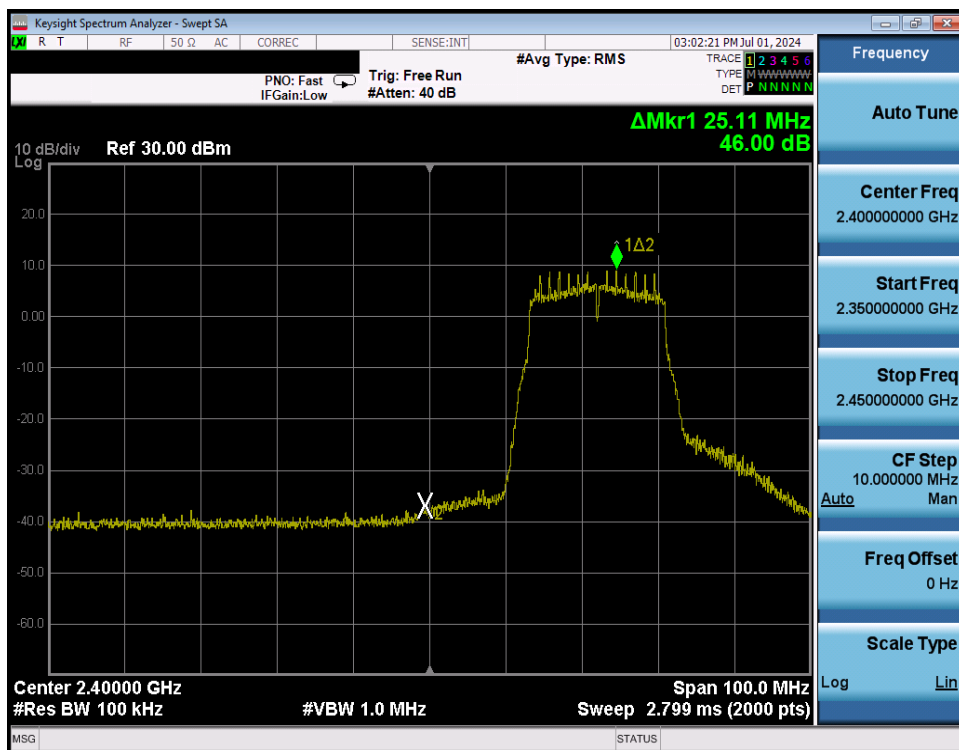
Plot 7-318. Band Edge Plot Antenna WF7 (802.11n (2.4GHz) – Ch. 3) – MCS2
