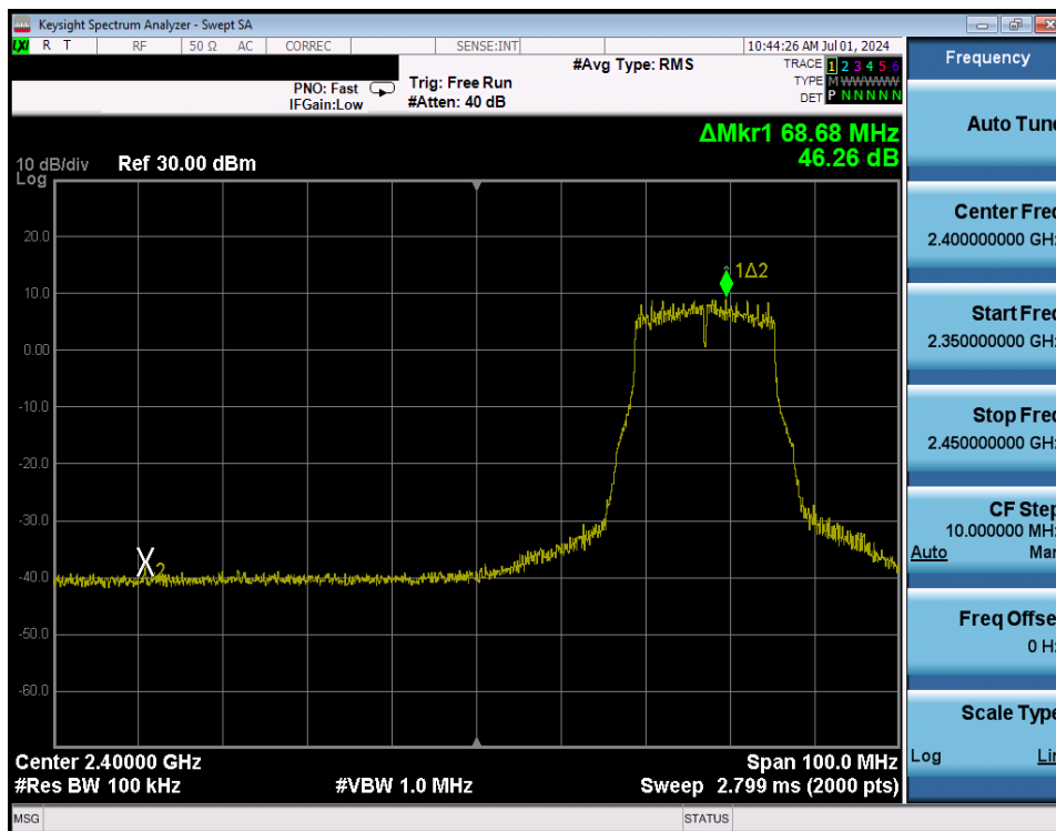
Plot 7-219. Band Edge Plot Antenna WF8 (802.11g – Ch. 4) – 24Mbps
