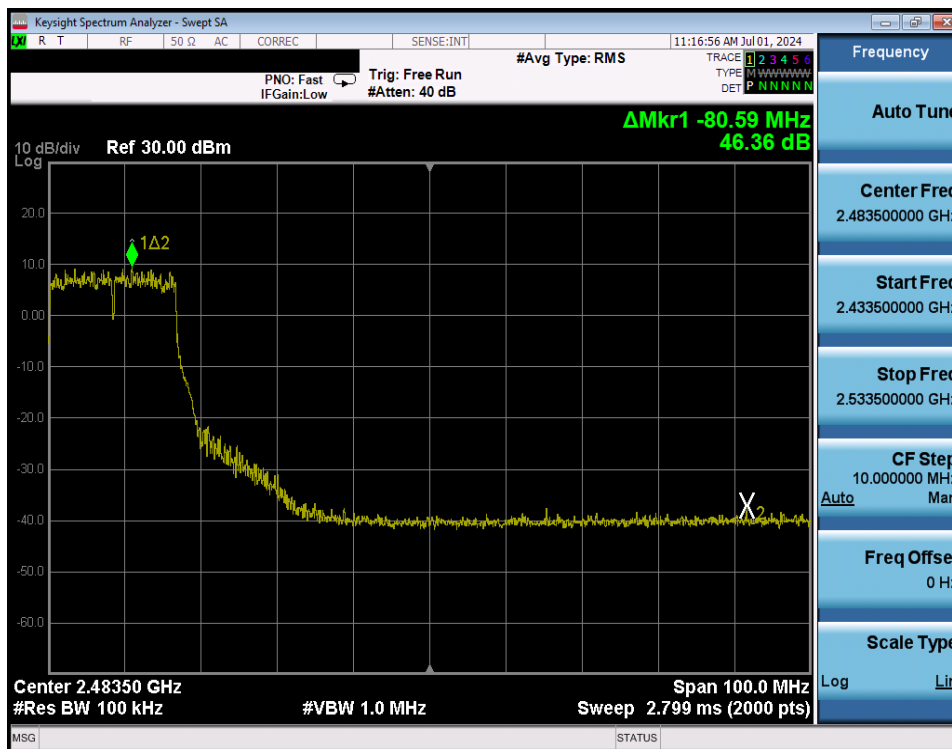
Plot 7-268. Band Edge Plot Antenna WF8 (802.11g – Ch. 7) – 54Mbps
