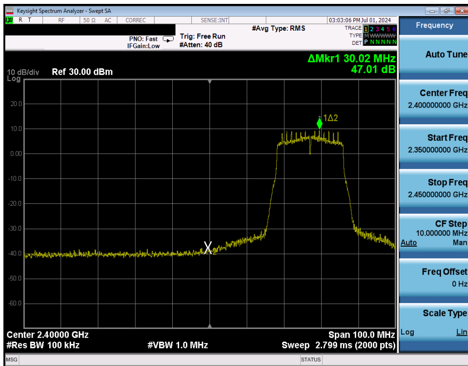
Plot 7-319. Band Edge Plot Antenna WF7 (802.11n (2.4GHz) – Ch. 4) – MCS2
