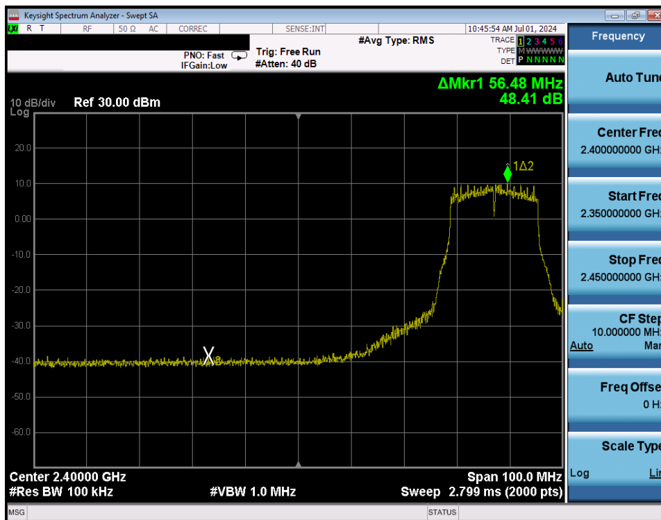
Plot 7-221. Band Edge Plot Antenna WF8 (802.11g – Ch. 6 Low) – 24Mbps
