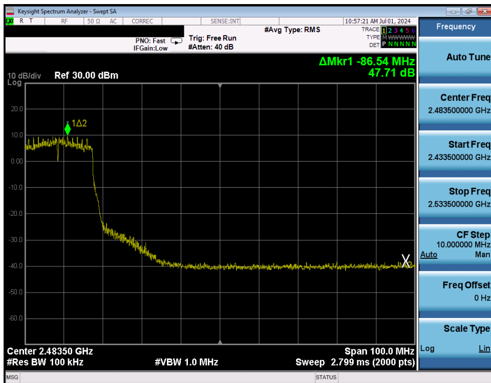
Plot 7-237. Band Edge Plot Antenna WF8 (802.11n (2.4GHz) - Ch. 7) - MCS4
