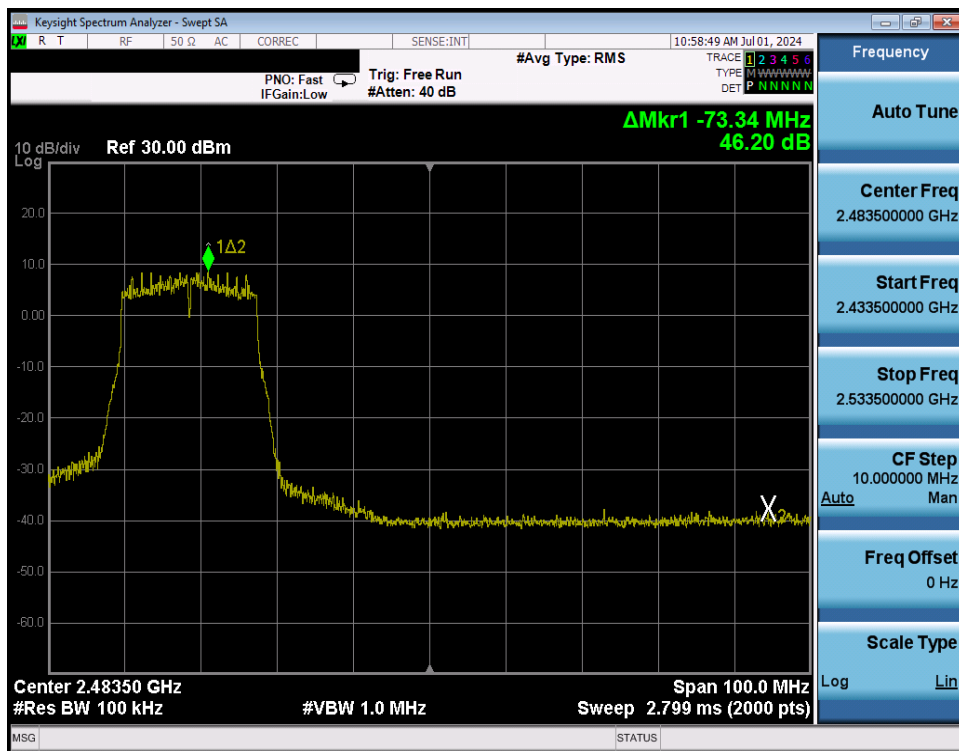
Plot 7-239. Band Edge Plot Antenna WF8 (802.11n (2.4GHz) – Ch. 9) – MCS4
