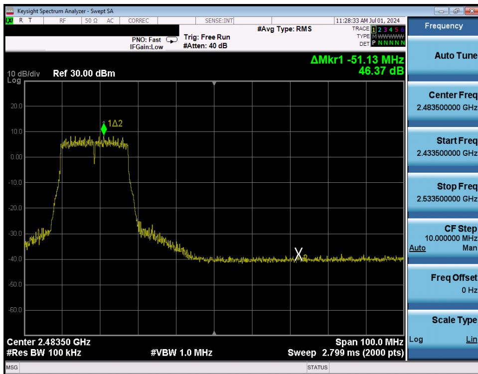
Plot 7-284. Band Edge Plot Antenna WF8 (802.11n (2.4GHz) – Ch. 9) – MCS7
