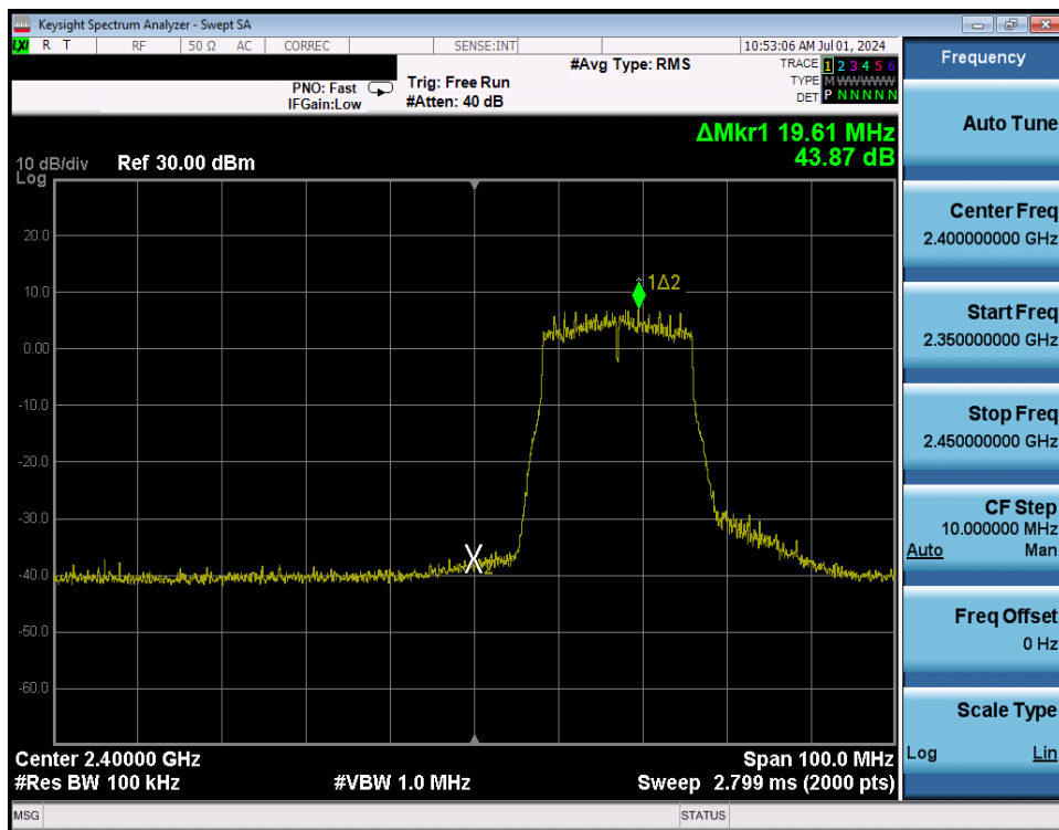
Plot 7-231. Band Edge Plot Antenna WF8 (802.11n (2.4GHz) – Ch. 2) – MCS4
