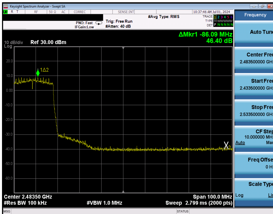
Plot 7-210. Band Edge Plot Antenna WF8 (802.11ax (SU - 2.4GHz) – Ch. 7) – MCS2
