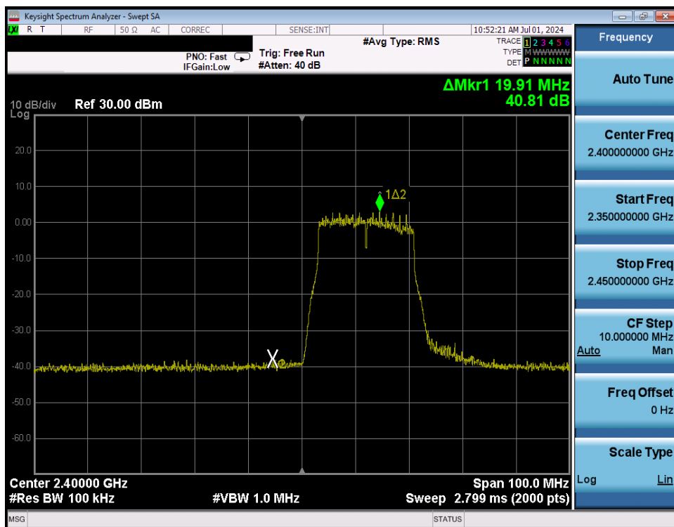
Plot 7-230. Band Edge Plot Antenna WF8 (802.11n (2.4GHz) – Ch. 1) – MCS4
