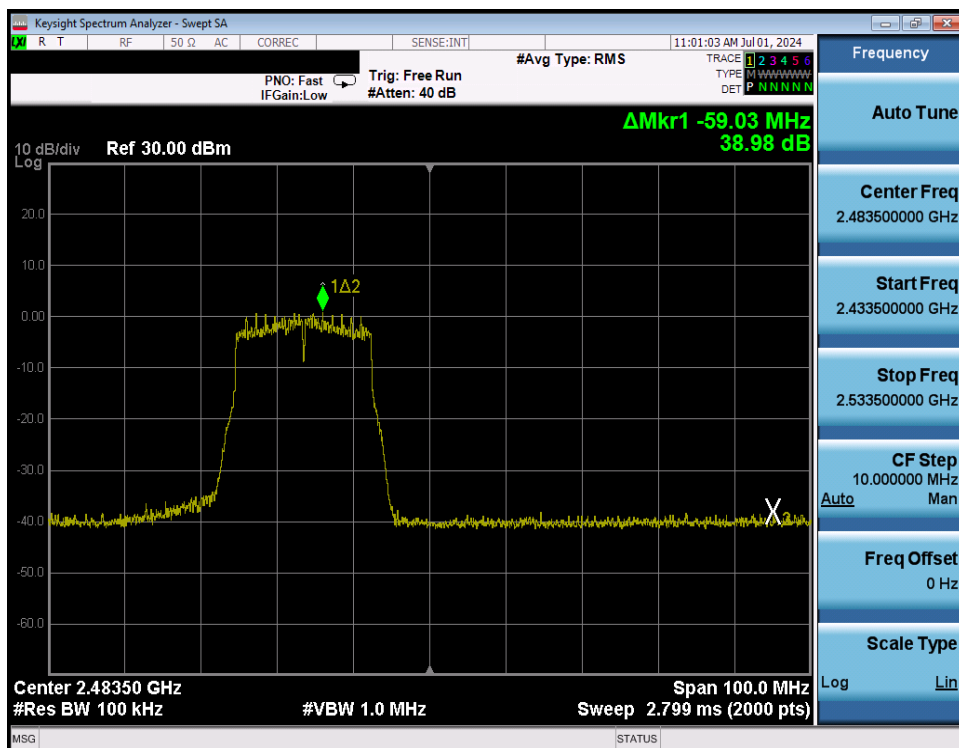
Plot 7-242. Band Edge Plot Antenna WF8 (802.11n (2.4GHz) – Ch. 12) – MCS4
