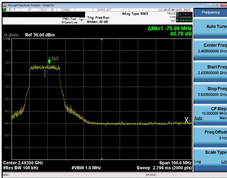
Plot 7-270. Band Edge Plot Antenna WF8 (802.11g - Ch. 9) - 54Mbps
