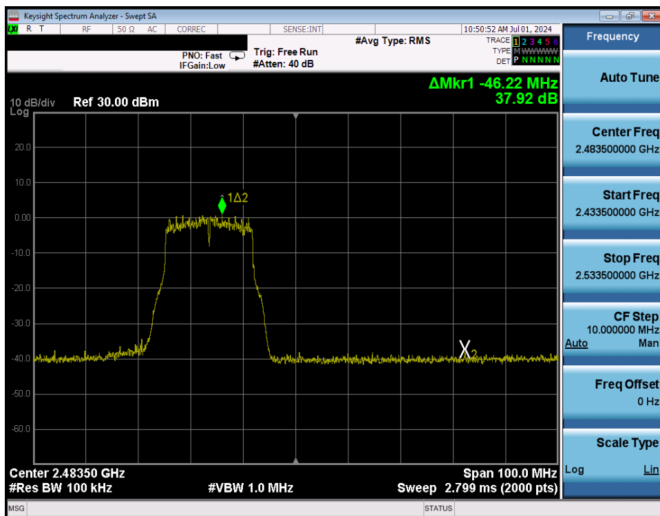
Plot 7-228. Band Edge Plot Antenna WF8 (802.11g – Ch. 12) – 24Mbps
