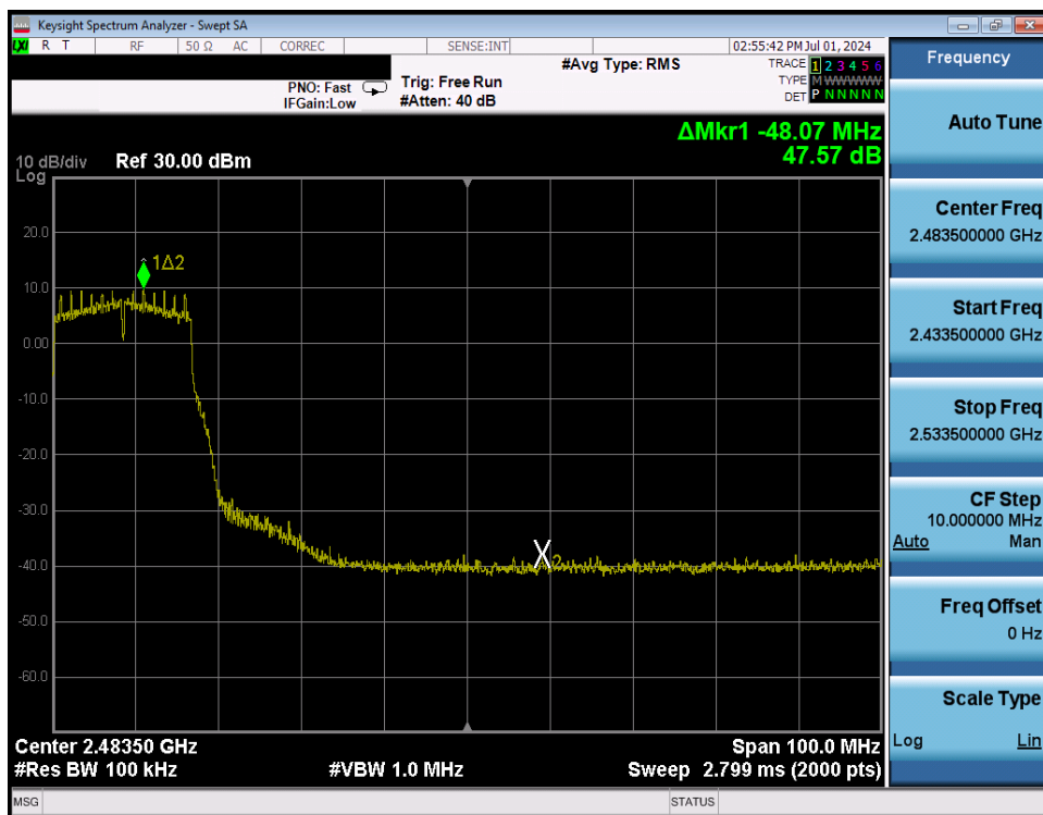
Plot 7-309. Band Edge Plot Antenna WF7 (802.11g – Ch. 7) – 12Mbps
