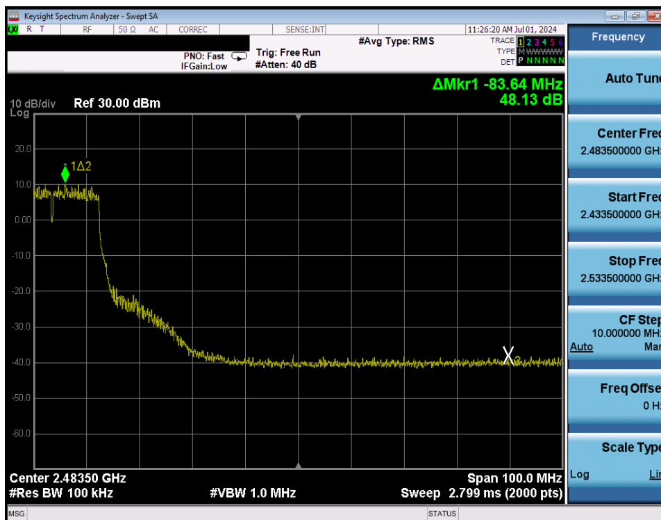
Plot 7-281. Band Edge Plot Antenna WF8 (802.11n (2.4GHz) – Ch. 6 High) – MCS7
