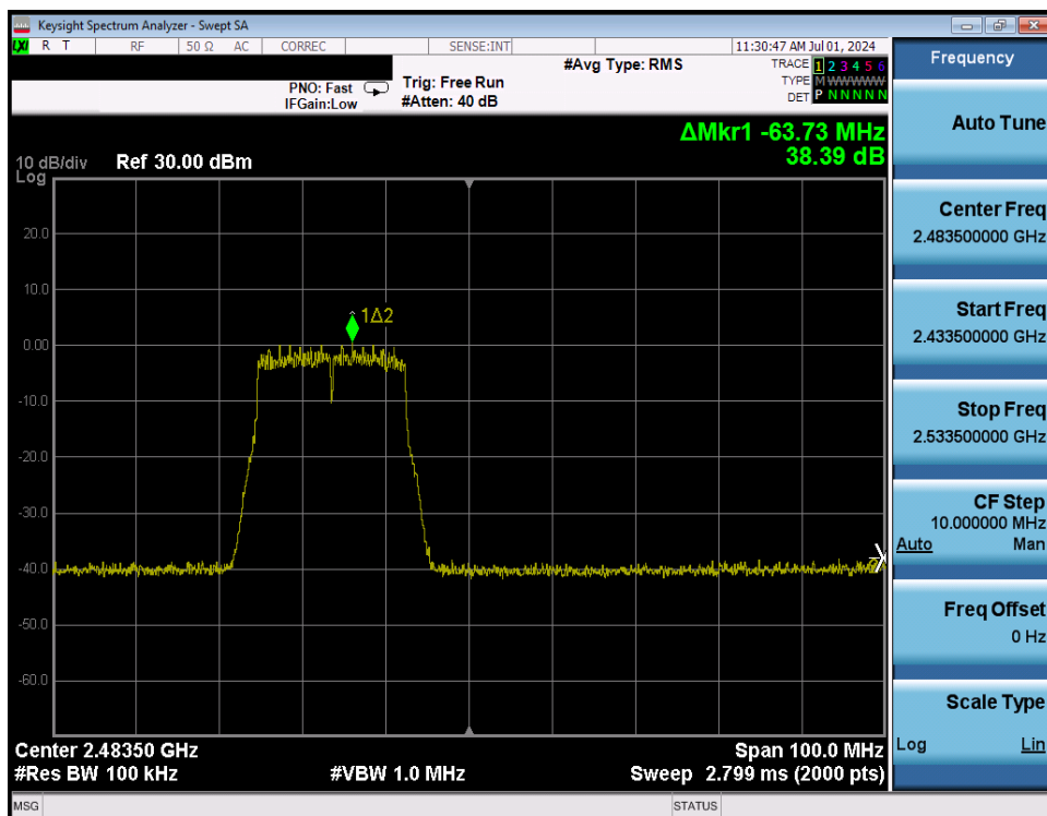
Plot 7-287. Band Edge Plot Antenna WF8 (802.11n (2.4GHz) – Ch. 12) – MCS7
