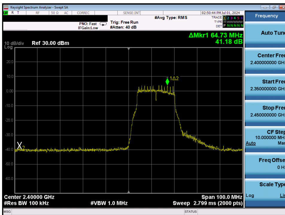
Plot 7-302. Band Edge Plot Antenna WF7 (802.11g – Ch. 1) – 12Mbps
