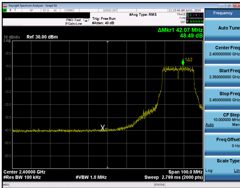
Plot 7-266. Band Edge Plot Antenna WF8 (802.11g – Ch. 6 Low) – 54Mbps
