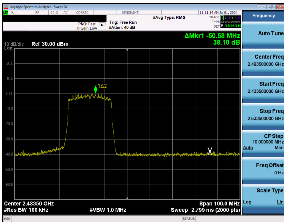
Plot 7-256. Band Edge Plot Antenna WF8 (802.11ax (SU - 2.4GHz) – Ch. 12) – MCS4
