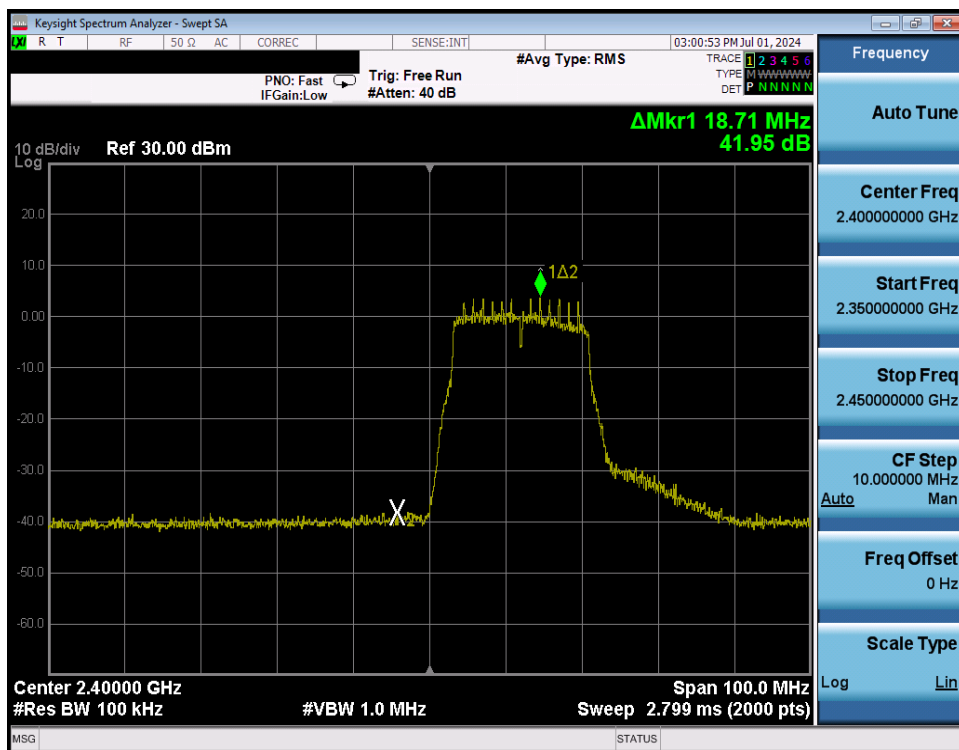
Plot 7-316. Band Edge Plot Antenna WF7 (802.11n (2.4GHz) – Ch. 1) – MCS2
