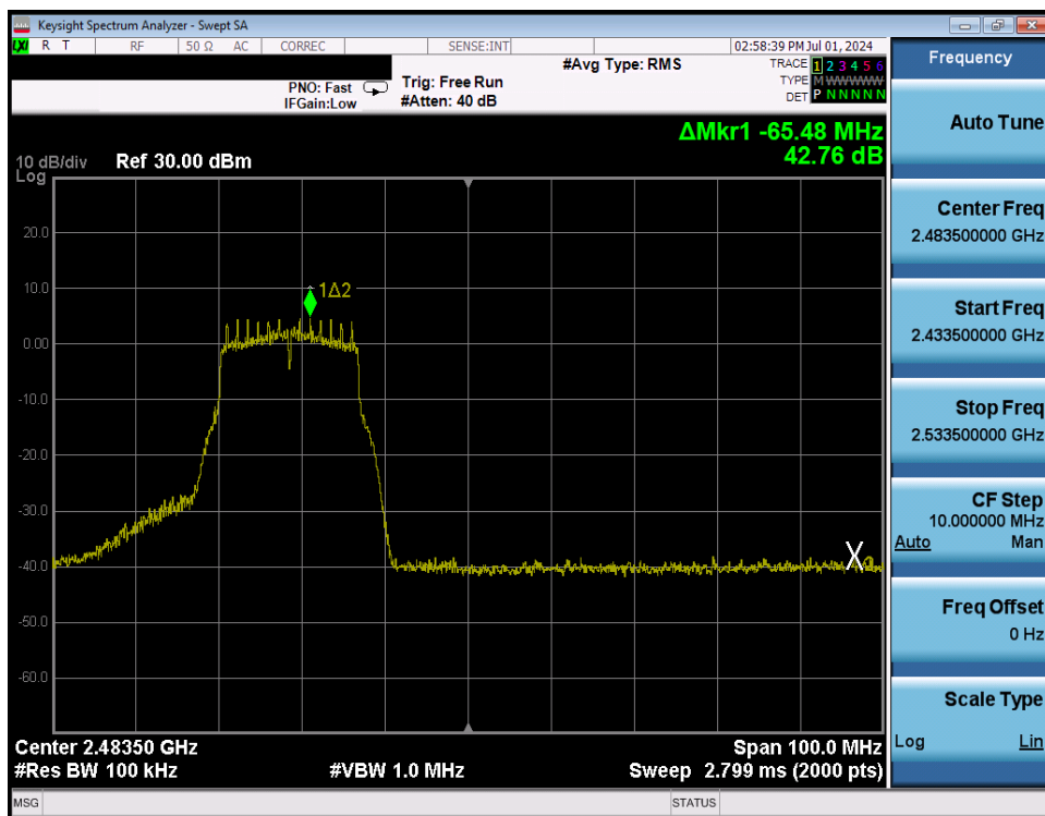
Plot 7-313. Band Edge Plot Antenna WF7 (802.11g – Ch. 11) – 12Mbps
