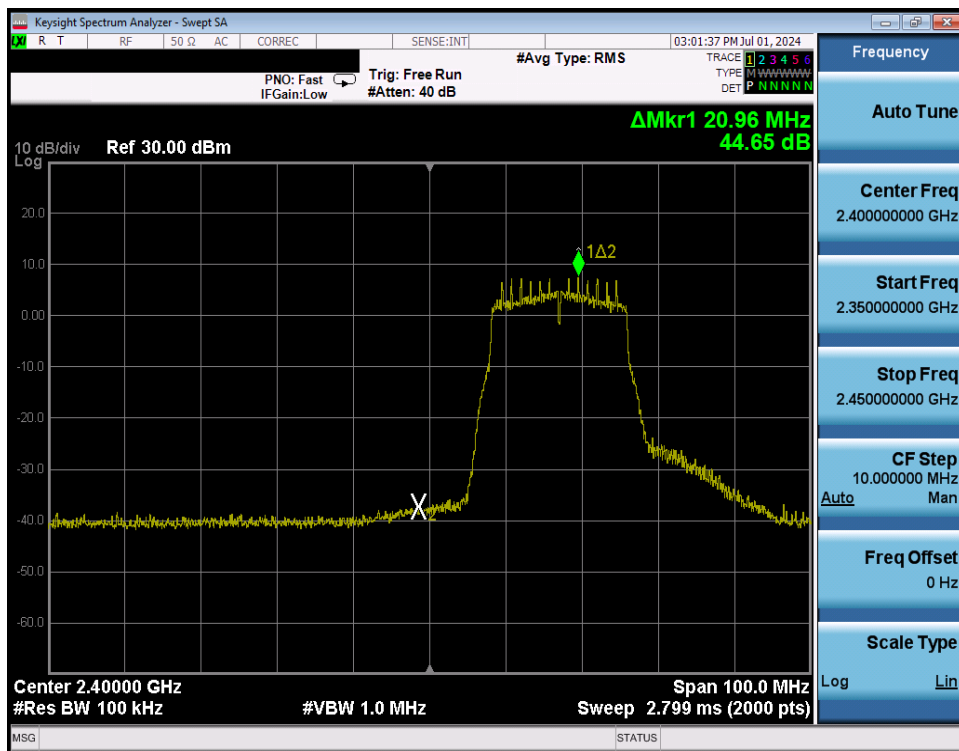
Plot 7-317. Band Edge Plot Antenna WF7 (802.11n (2.4GHz) – Ch. 2) – MCS2
