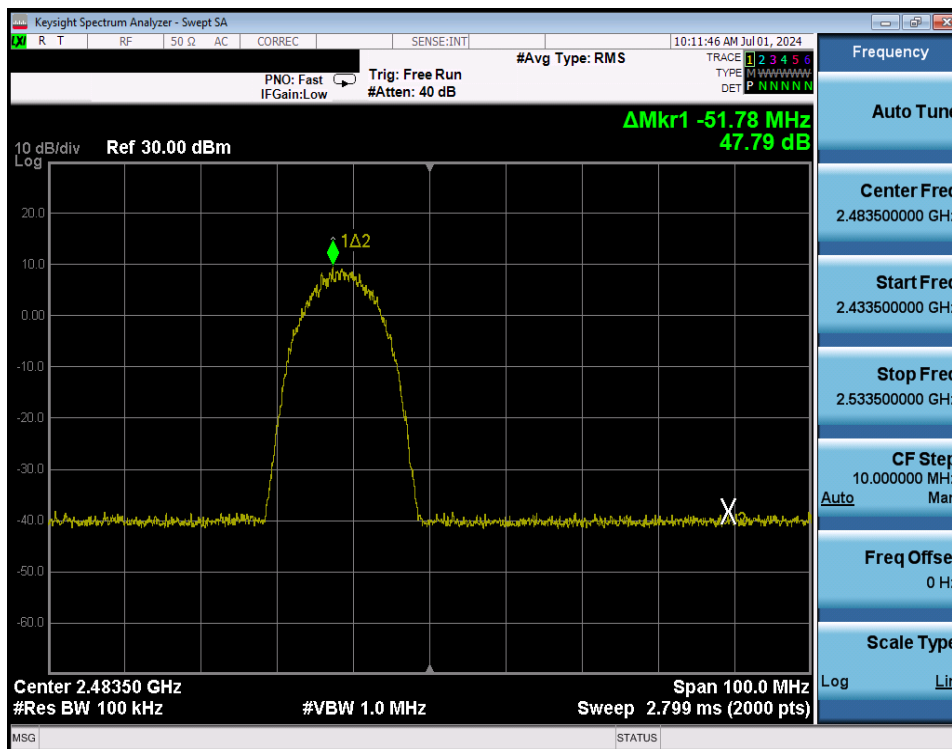
Plot 7-260. Band Edge Plot Antenna WF8 (802.11b – Ch. 13) – 11Mbps
