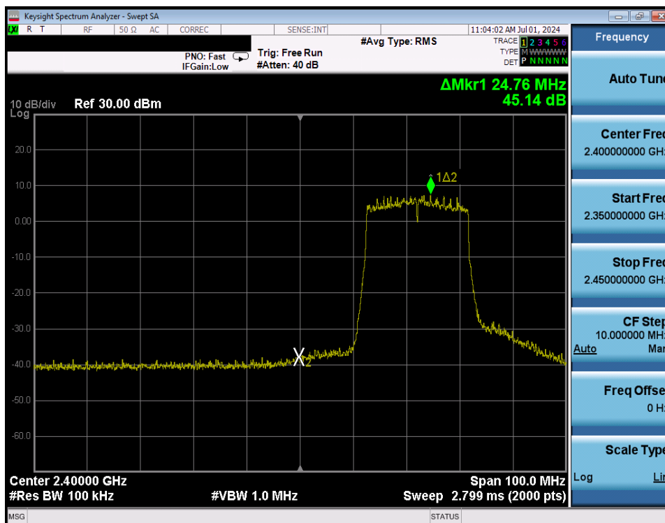
Plot 7-246. Band Edge Plot Antenna WF8 (802.11ax (SU - 2.4GHz) – Ch. 3) – MCS4
