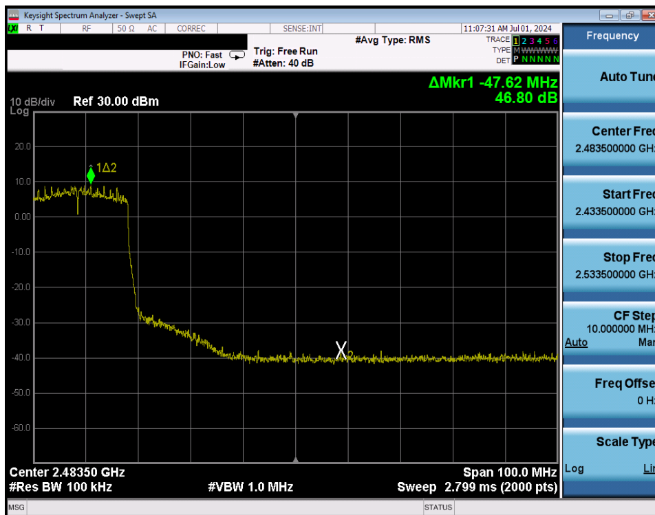
Plot 7-251. Band Edge Plot Antenna WF8 (802.11ax (SU - 2.4GHz) – Ch. 7) – MCS4
