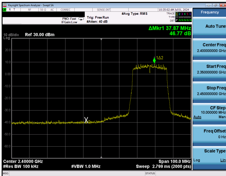
Plot 7-206. Band Edge Plot Antenna WF8 (802.11ax (SU - 2.4GHz) – Ch. 4) – MCS2
