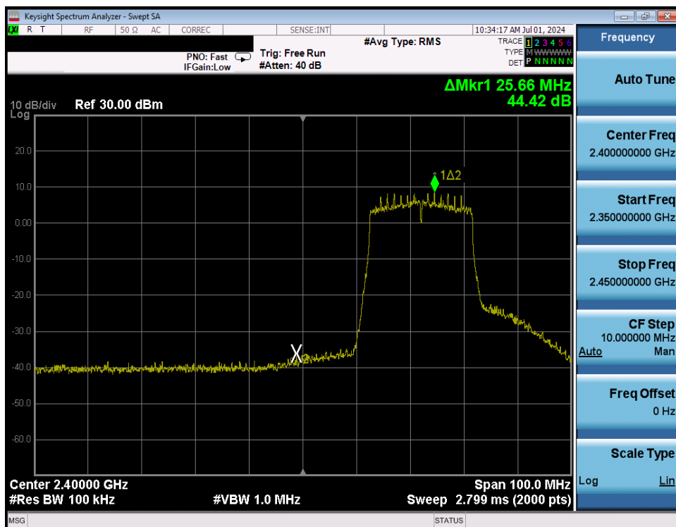
Plot 7-205. Band Edge Plot Antenna WF8 (802.11ax (SU - 2.4GHz) – Ch. 3) – MCS2
