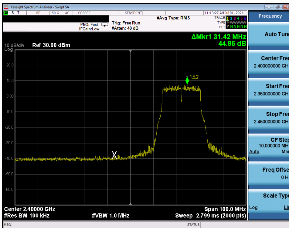
Plot 7-263. Band Edge Plot Antenna WF8 (802.11g – Ch. 3) – 54Mbps
