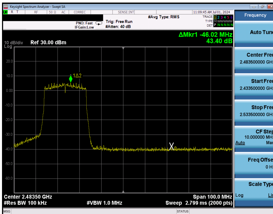
Plot 7-254. Band Edge Plot Antenna WF8 (802.11ax (SU - 2.4GHz) – Ch. 10) – MCS4
