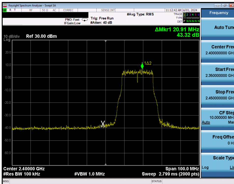
Plot 7-262. Band Edge Plot Antenna WF8 (802.11g – Ch. 2) – 54Mbps
