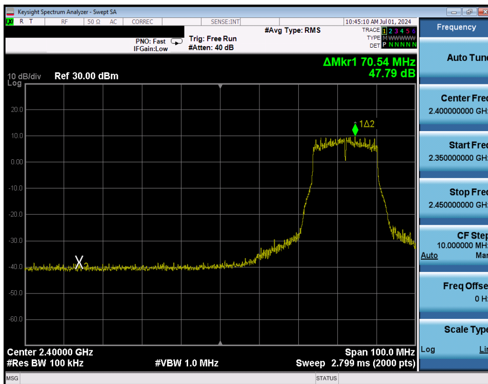
Plot 7-220. Band Edge Plot Antenna WF8 (802.11g – Ch. 5) – 24Mbps
