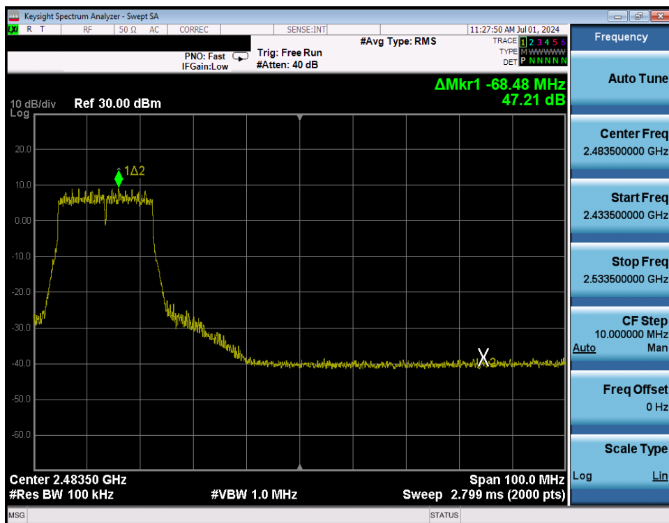
Plot 7-283. Band Edge Plot Antenna WF8 (802.11n (2.4GHz) – Ch. 8) – MCS7
