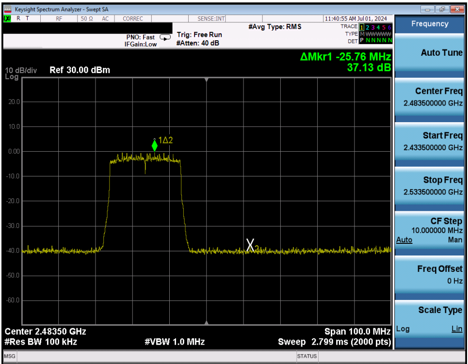
Plot 7-301. Band Edge Plot Antenna WF8 (802.11ax (SU - 2.4GHz) – Ch. 12) – MCS9
