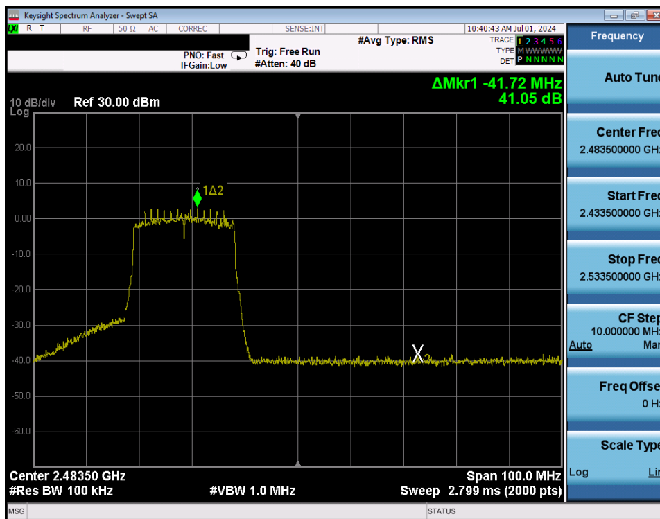
Plot 7-214. Band Edge Plot Antenna WF8 (802.11ax (SU - 2.4GHz) – Ch. 11) – MCS2
