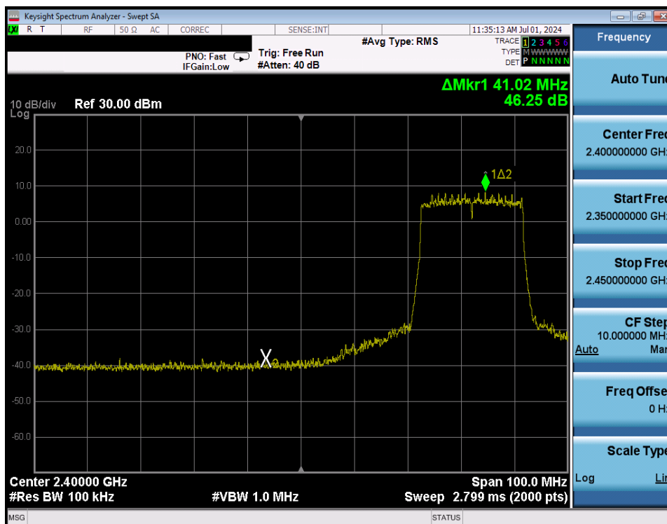
Plot 7-293. Band Edge Plot Antenna WF8 (802.11ax (SU - 2.4GHz) – Ch. 5) – MCS9
