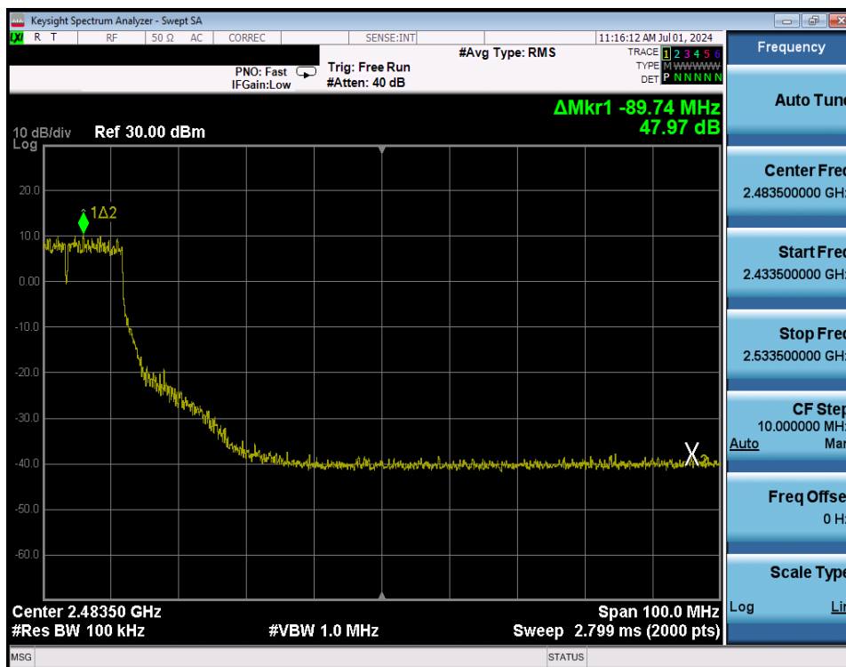
Plot 7-267. Band Edge Plot Antenna WF8 (802.11g – Ch. 6 High) – 54Mbps
