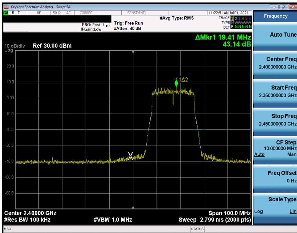
Plot 7-276. Band Edge Plot Antenna WF8 (802.11n (2.4GHz) – Ch. 2) – MCS7
