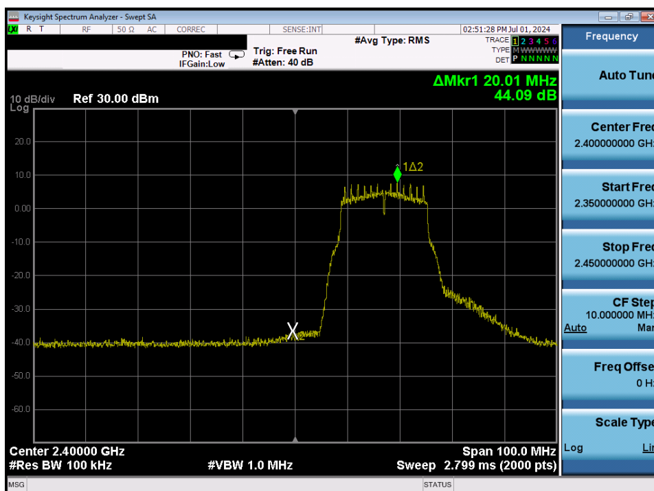
Plot 7-303. Band Edge Plot Antenna WF7 (802.11g – Ch. 2) – 12Mbps
