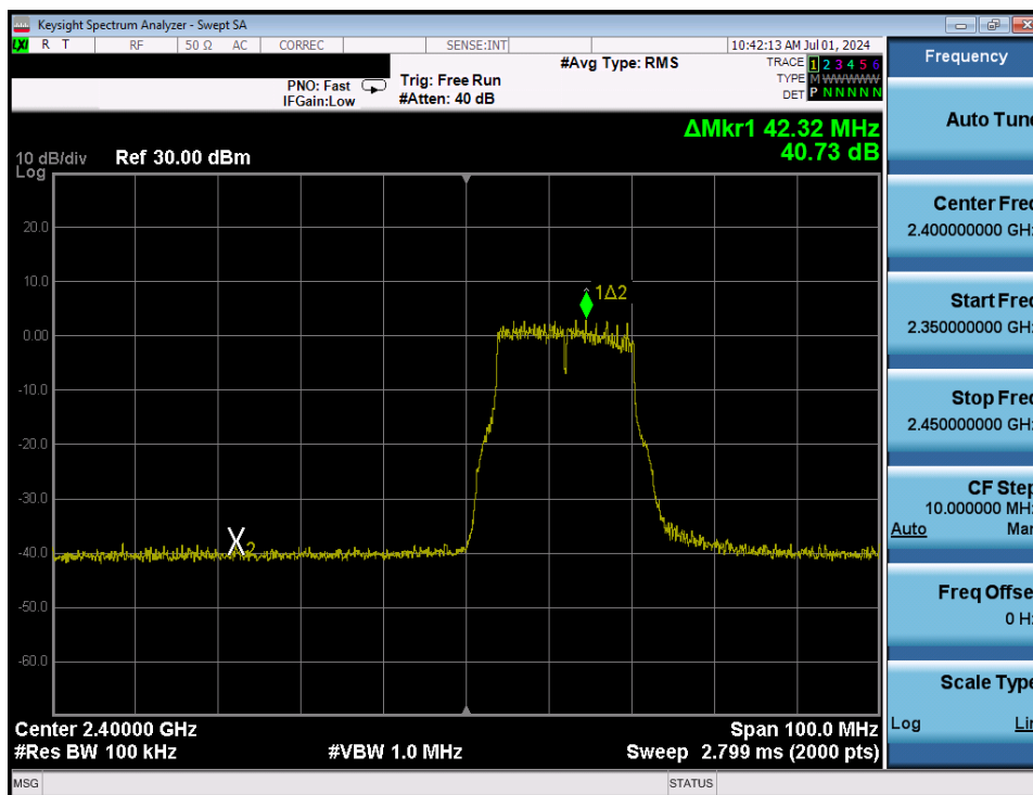
Plot 7-216. Band Edge Plot Antenna WF8 (802.11g – Ch. 1) – 24Mbps
