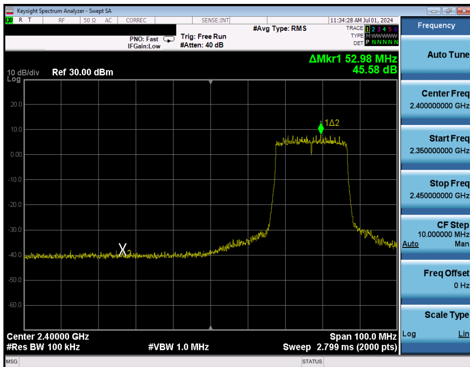
Plot 7-292. Band Edge Plot Antenna WF8 (802.11ax (SU - 2.4GHz) – Ch. 4) – MCS9
