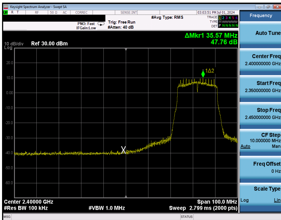
Plot 7-320. Band Edge Plot Antenna WF7 (802.11n (2.4GHz) – Ch. 5) – MCS2
