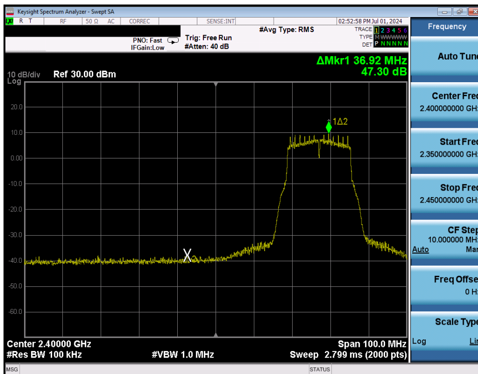
Plot 7-305. Band Edge Plot Antenna WF7 (802.11g – Ch. 4) – 12Mbps
