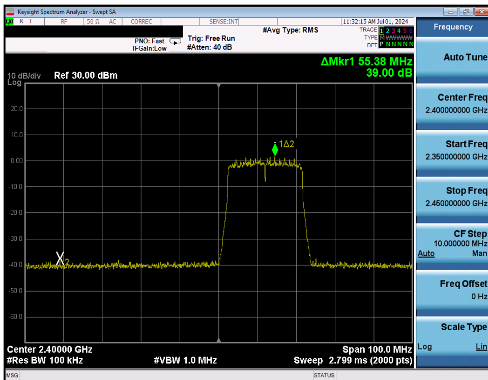
Plot 7-289. Band Edge Plot Antenna WF8 (802.11ax (SU - 2.4GHz) – Ch. 1) – MCS9
