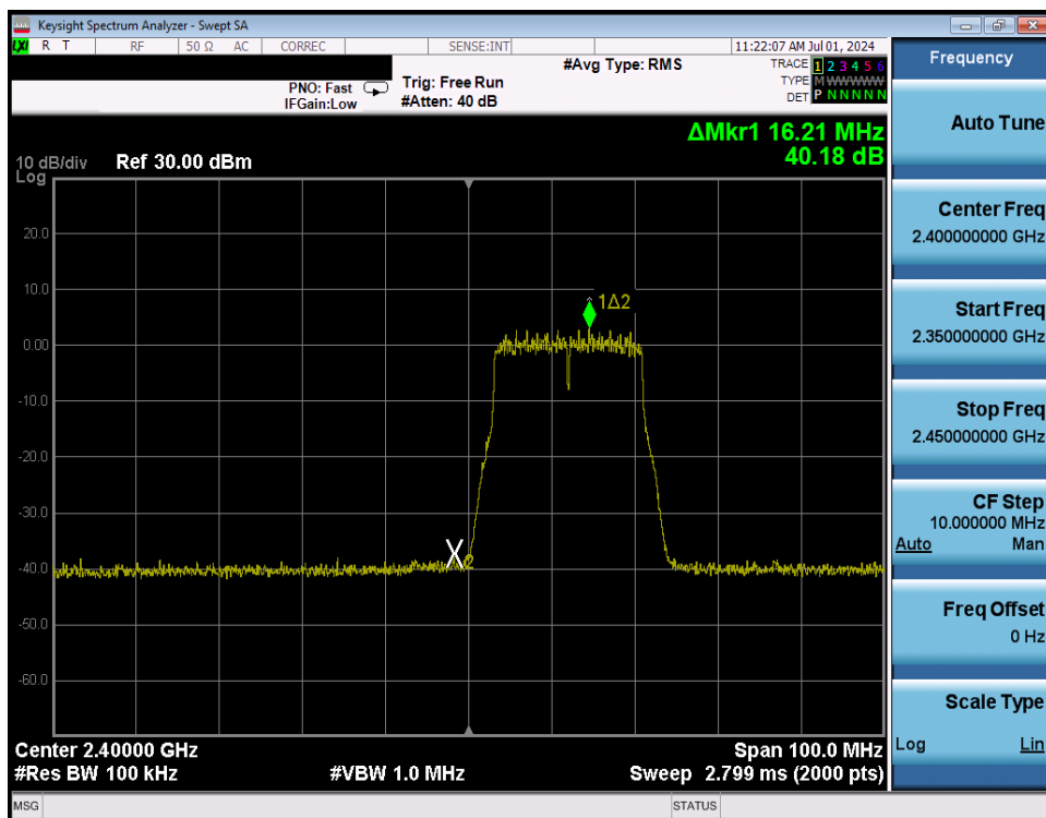
Plot 7-275. Band Edge Plot Antenna WF8 (802.11n (2.4GHz) – Ch. 1) – MCS7
