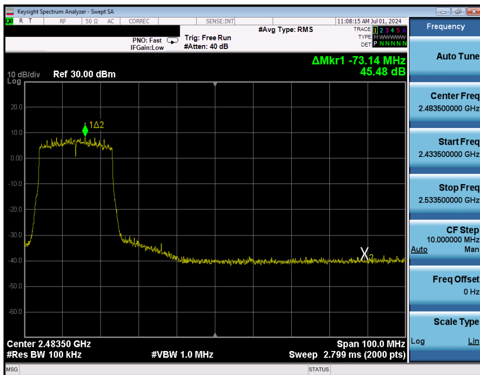
Plot 7-252. Band Edge Plot Antenna WF8 (802.11ax (SU - 2.4GHz) – Ch. 8) – MCS4
