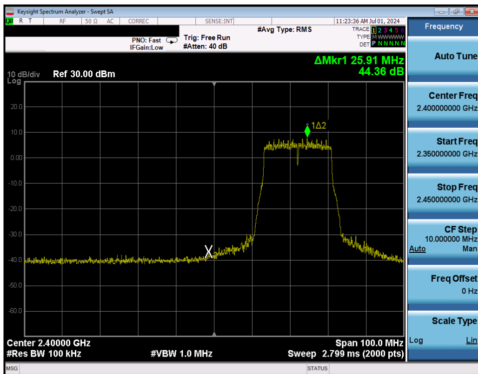
Plot 7-277. Band Edge Plot Antenna WF8 (802.11n (2.4GHz) – Ch. 3) – MCS7
