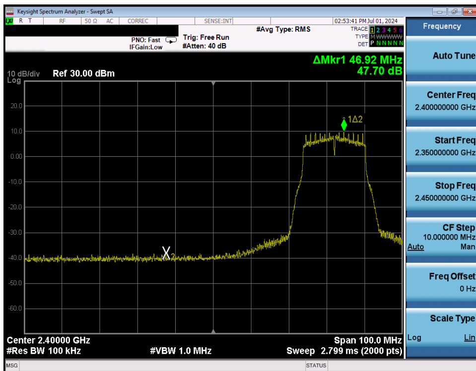
Plot 7-306. Band Edge Plot Antenna WF7 (802.11g – Ch. 5) – 12Mbps
