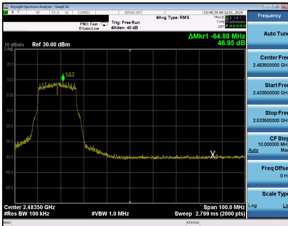
Plot 7-225. Band Edge Plot Antenna WF8 (802.11g – Ch. 9) – 24Mbps
