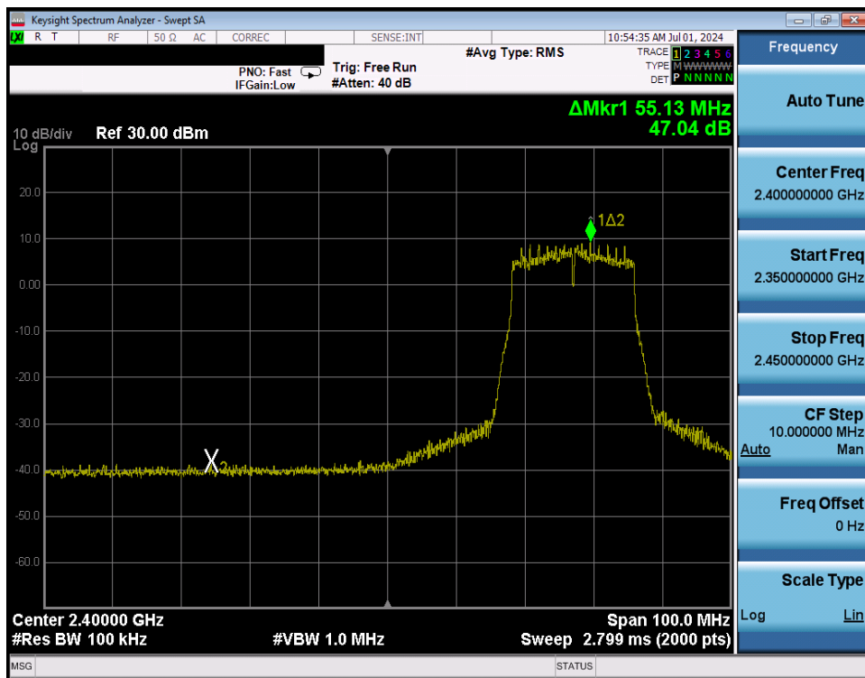
Plot 7-233. Band Edge Plot Antenna WF8 (802.11n (2.4GHz) – Ch. 4) – MCS4
