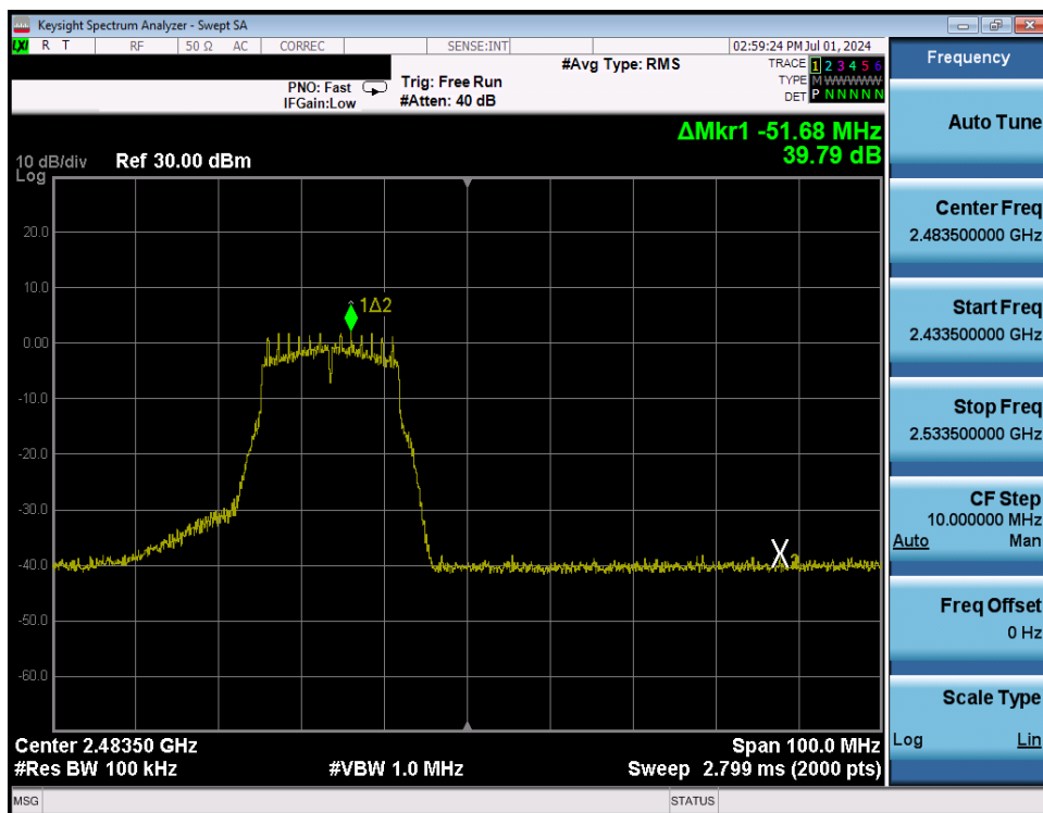
Plot 7-314. Band Edge Plot Antenna WF7 (802.11g – Ch. 12) – 12Mbps
