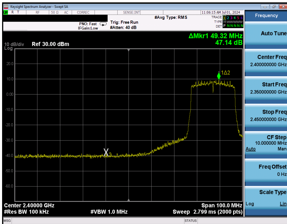
Plot 7-249. Band Edge Plot Antenna WF8 (802.11ax (SU - 2.4GHz) – Ch. 6 Low) – MCS4
