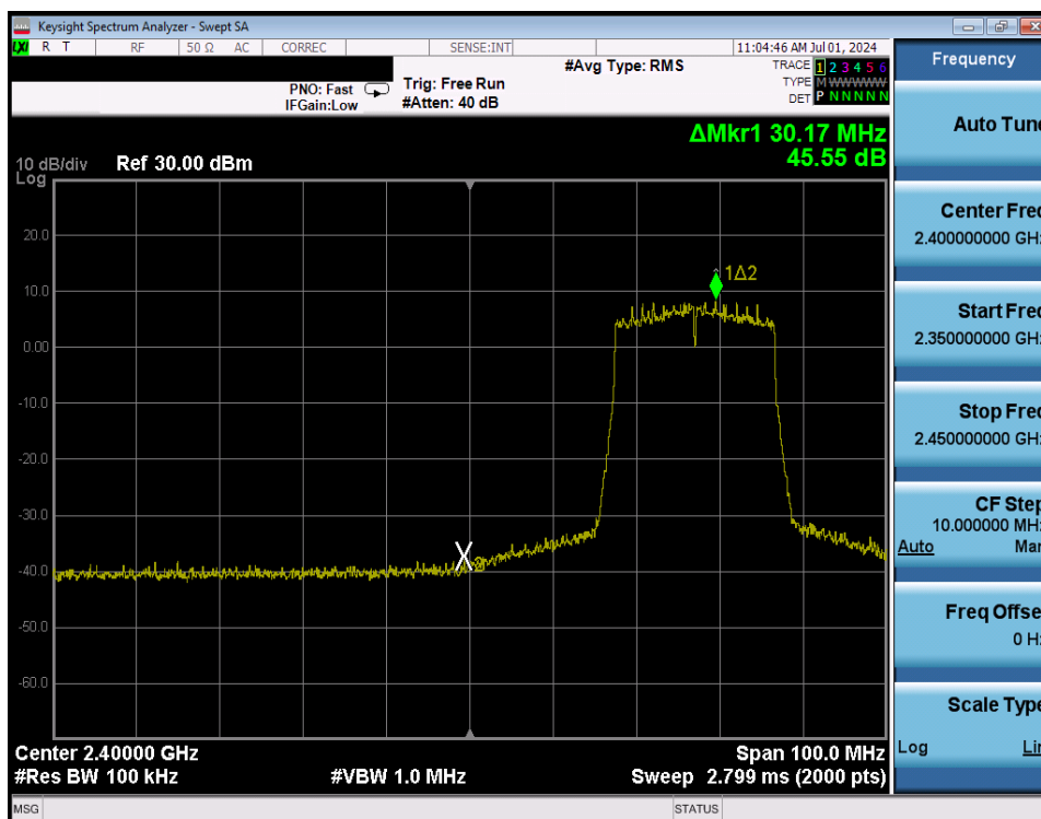
Plot 7-247. Band Edge Plot Antenna WF8 (802.11ax (SU - 2.4GHz) – Ch. 4) – MCS4
