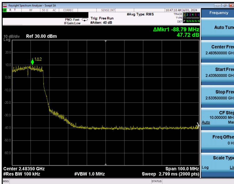
Plot 7-223. Band Edge Plot Antenna WF8 (802.11g – Ch. 7) – 24Mbps
