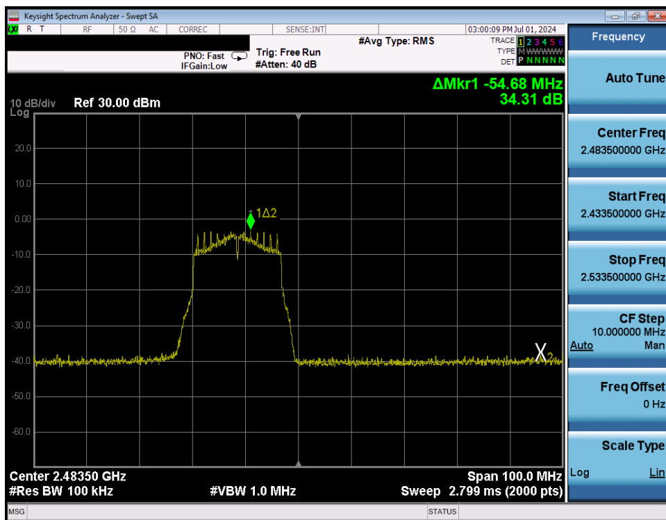
Plot 7-315. Band Edge Plot Antenna WF7 (802.11g – Ch. 13) – 12Mbps
