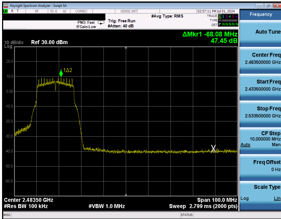
Plot 7-311. Band Edge Plot Antenna WF7 (802.11g – Ch. 9) – 12Mbps
