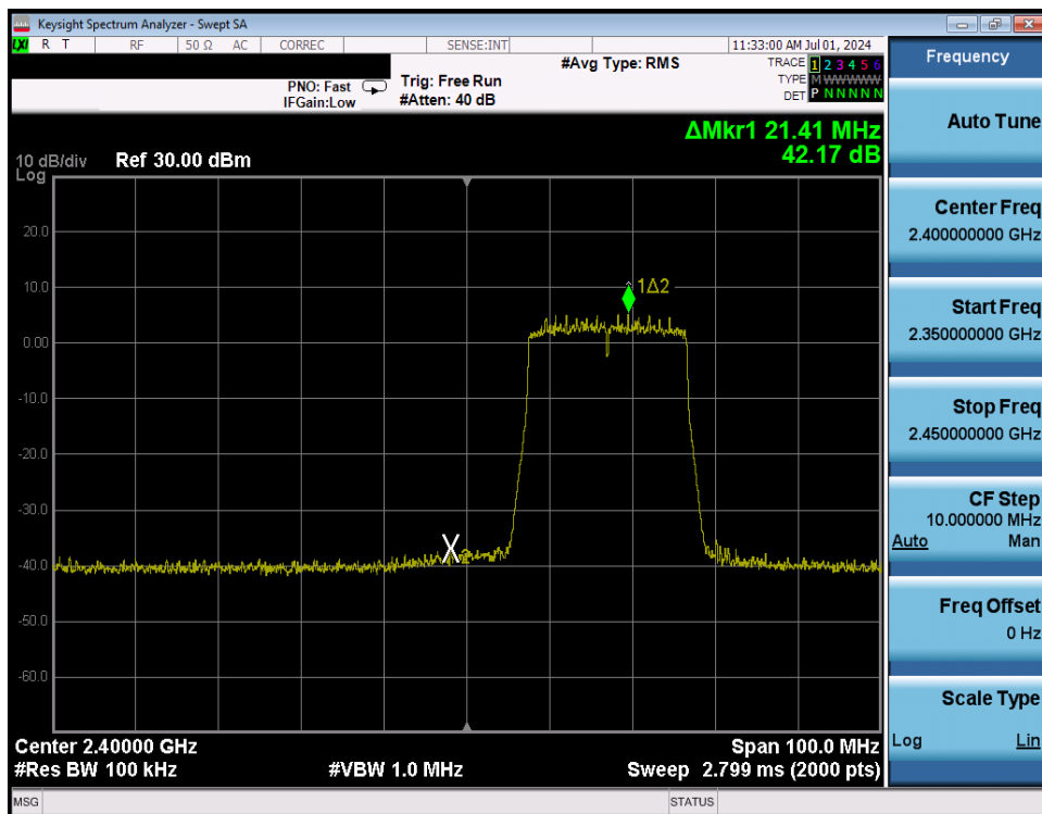
Plot 7-290. Band Edge Plot Antenna WF8 (802.11ax (SU - 2.4GHz) – Ch. 2) – MCS9
