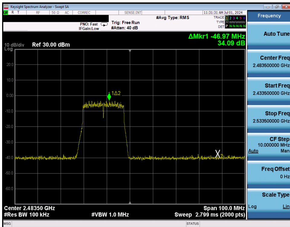
Plot 7-288. Band Edge Plot Antenna WF8 (802.11n (2.4GHz) – Ch. 13) – MCS7
