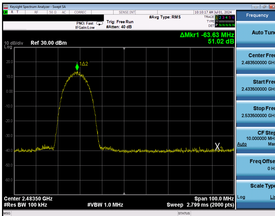
Plot 7-258. Band Edge Plot Antenna WF8 (802.11b – Ch. 11) – 11Mbps
