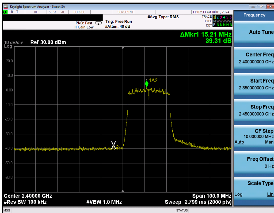
Plot 7-244. Band Edge Plot Antenna WF8 (802.11ax (SU - 2.4GHz) – Ch. 1) – MCS4
