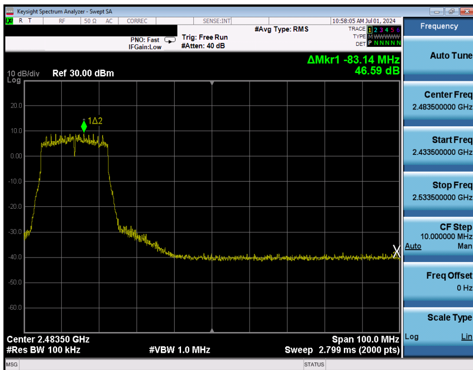
Plot 7-238. Band Edge Plot Antenna WF8 (802.11n (2.4GHz) – Ch. 8) – MCS4
