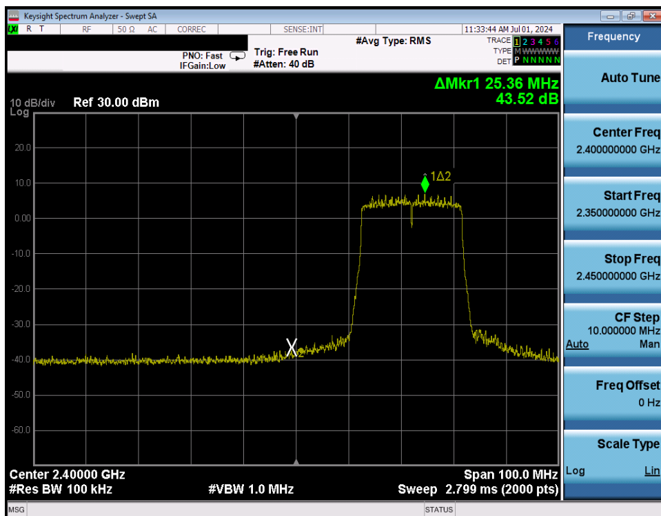
Plot 7-291. Band Edge Plot Antenna WF8 (802.11ax (SU - 2.4GHz) – Ch. 3) – MCS9
