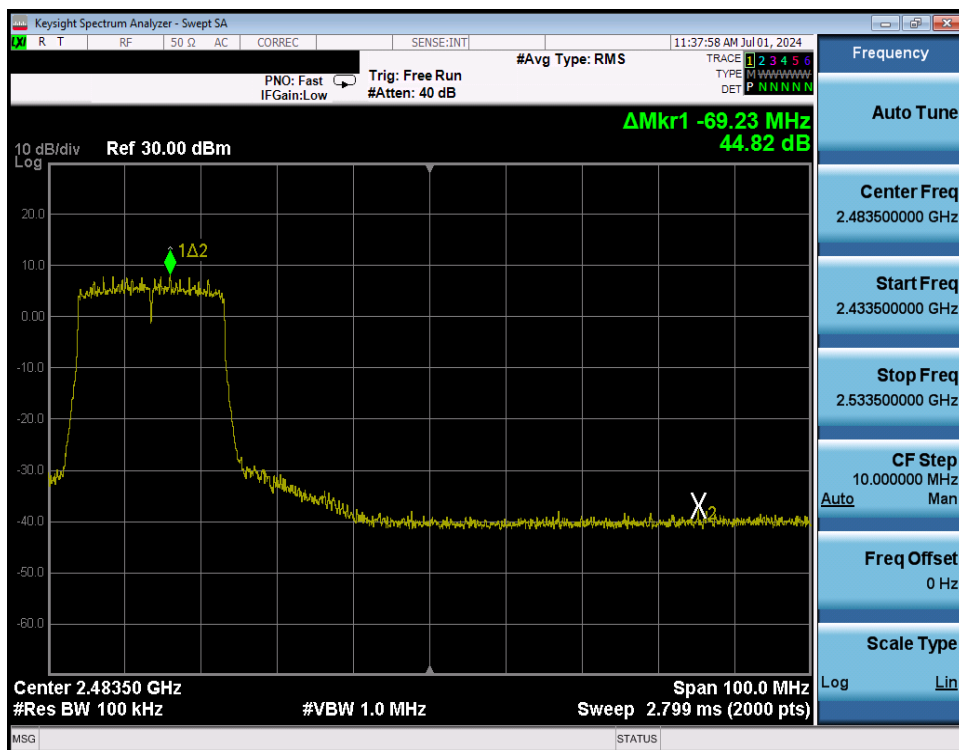
Plot 7-297. Band Edge Plot Antenna WF8 (802.11ax (SU - 2.4GHz) – Ch. 8) – MCS9
