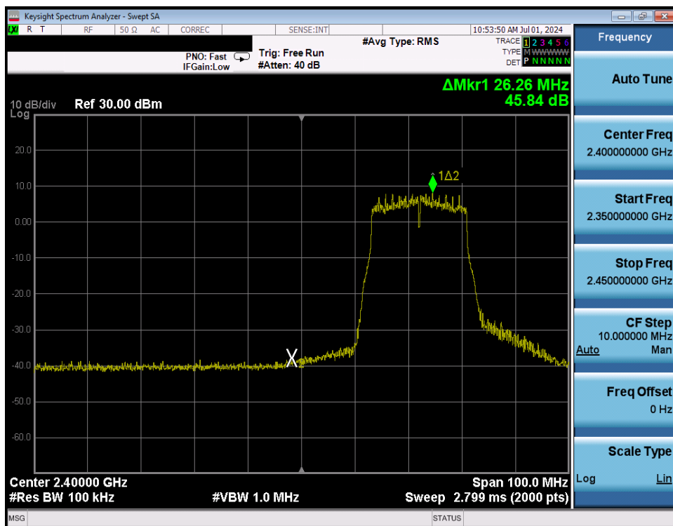
Plot 7-232. Band Edge Plot Antenna WF8 (802.11n (2.4GHz) – Ch. 3) – MCS4
