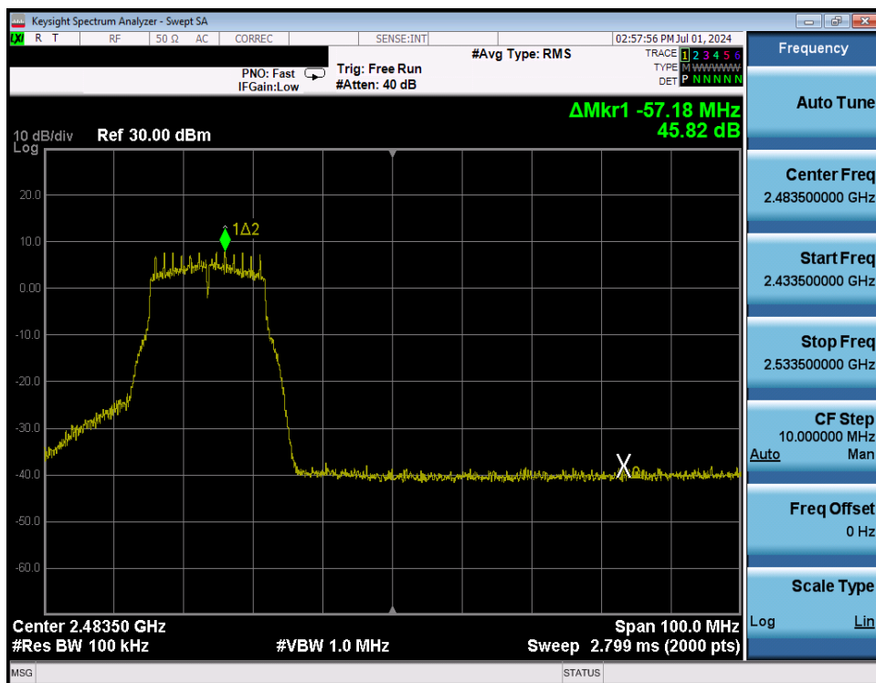
Plot 7-312. Band Edge Plot Antenna WF7 (802.11g – Ch. 10) – 12Mbps
