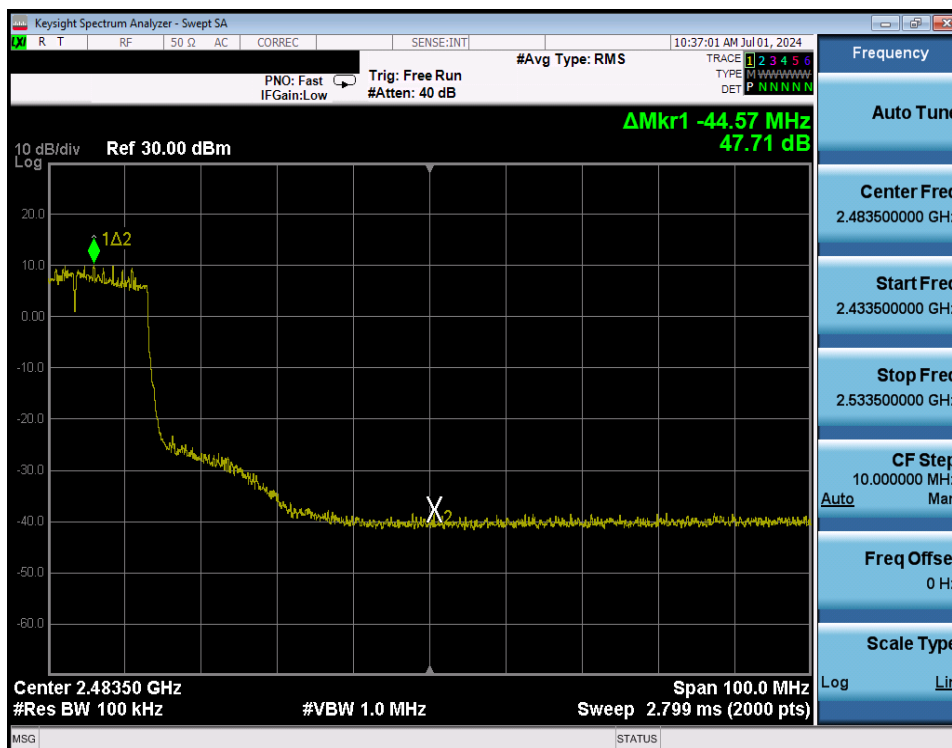
Plot 7-209. Band Edge Plot Antenna WF8 (802.11ax (SU - 2.4GHz) – Ch. 6 High) – MCS2
