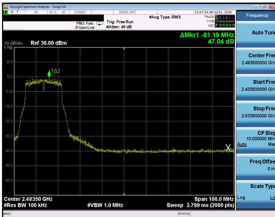
Plot 7-224. Band Edge Plot Antenna WF8 (802.11g – Ch. 8) – 24Mbps
