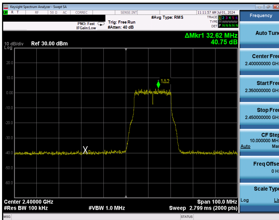
Plot 7-261. Band Edge Plot Antenna WF8 (802.11g – Ch. 1) – 54Mbps
