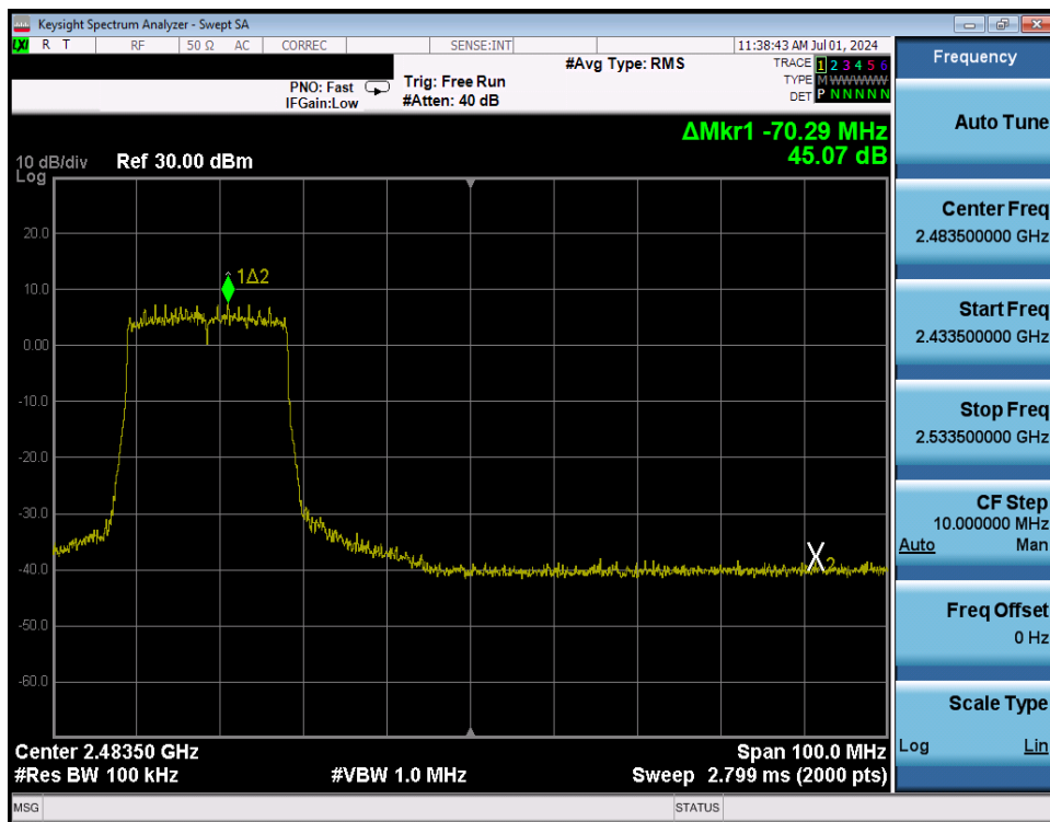
Plot 7-298. Band Edge Plot Antenna WF8 (802.11ax (SU - 2.4GHz) – Ch. 9) – MCS9
