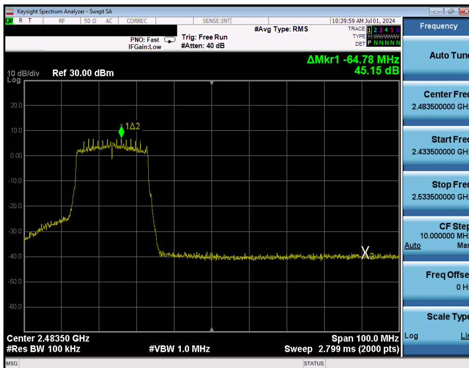
Plot 7-213. Band Edge Plot Antenna WF8 (802.11ax (SU - 2.4GHz) – Ch. 10) – MCS2
