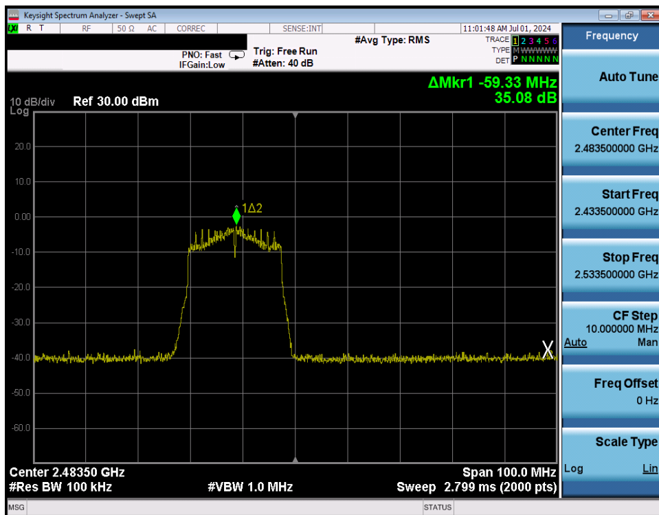
Plot 7-243. Band Edge Plot Antenna WF8 (802.11n (2.4GHz) – Ch. 13) – MCS4
