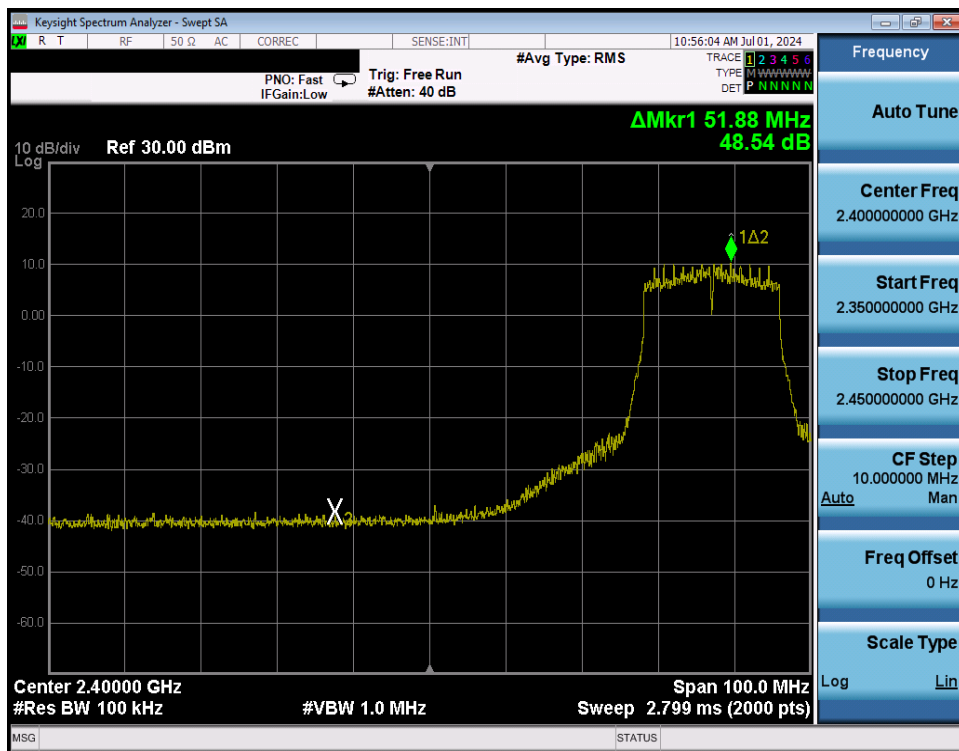
Plot 7-235. Band Edge Plot Antenna WF8 (802.11n (2.4GHz) – Ch. 6 Low) – MCS4
