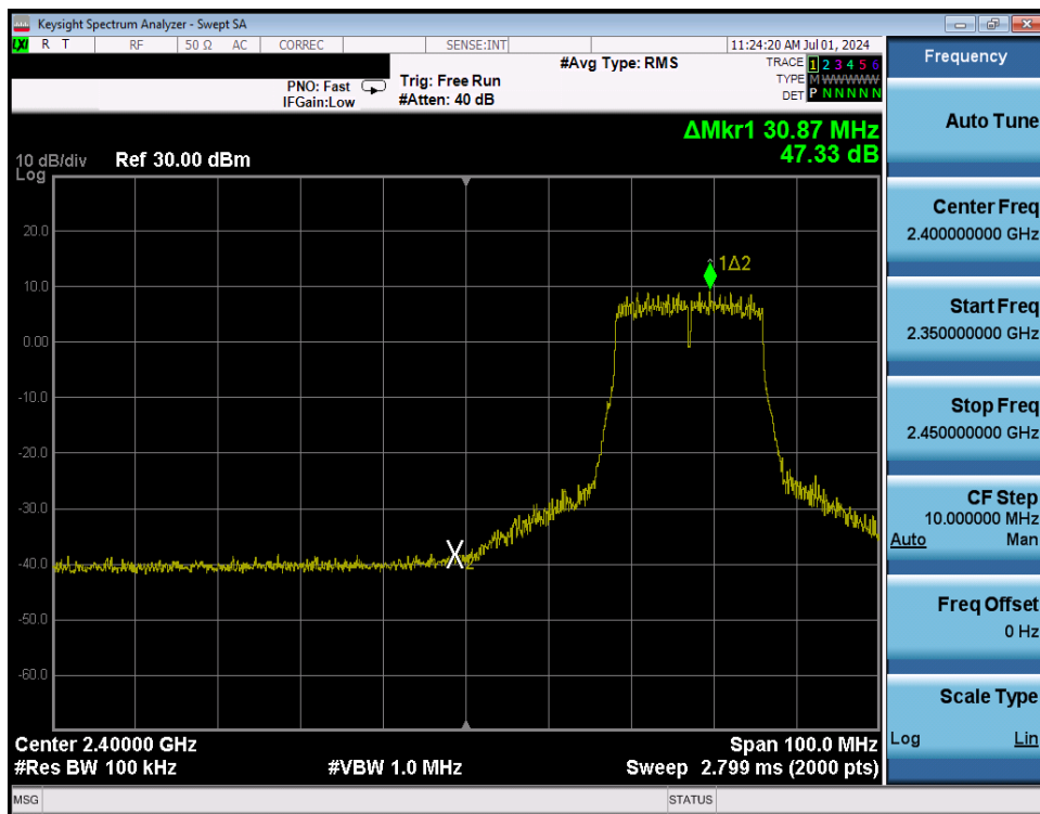
Plot 7-278. Band Edge Plot Antenna WF8 (802.11n (2.4GHz) – Ch. 4) – MCS7
