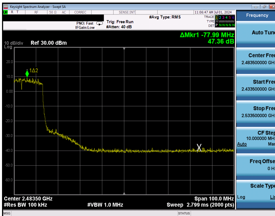
Plot 7-250. Band Edge Plot Antenna WF8 (802.11ax (SU - 2.4GHz) – Ch. 6 High) – MCS4
