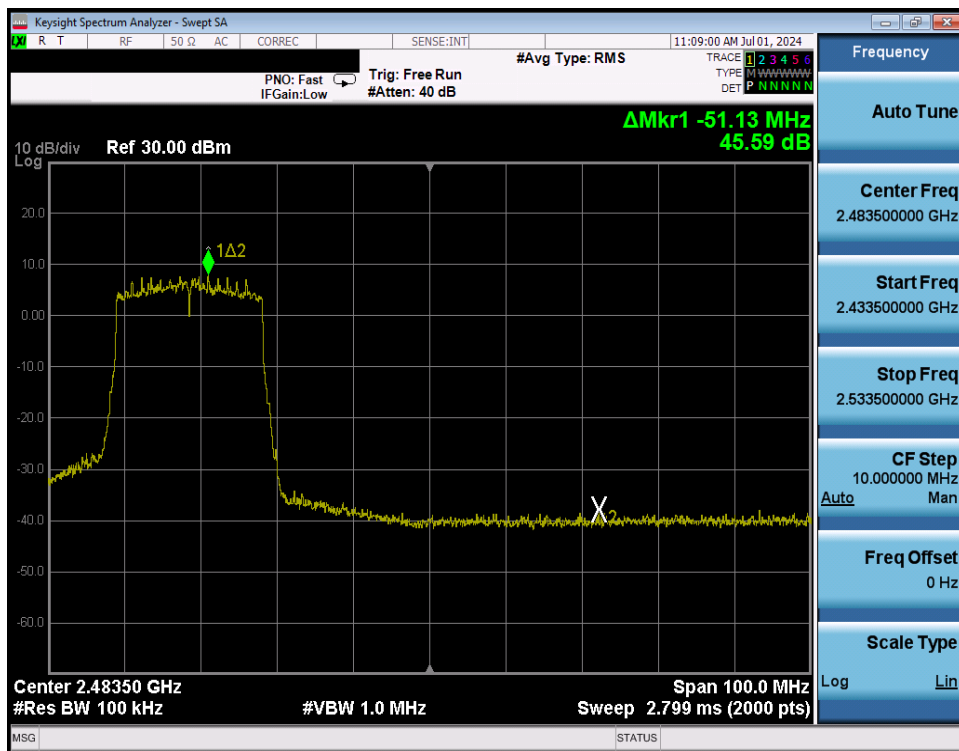
Plot 7-253. Band Edge Plot Antenna WF8 (802.11ax (SU - 2.4GHz) – Ch. 9) – MCS4
