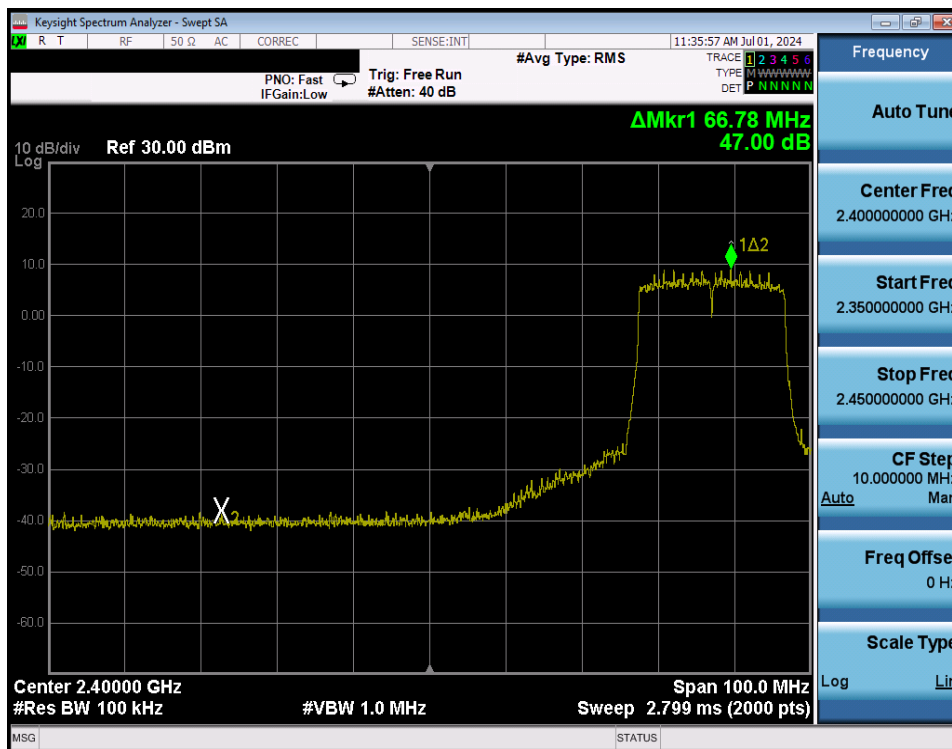
Plot 7-294. Band Edge Plot Antenna WF8 (802.11ax (SU - 2.4GHz) – Ch. 6 Low) – MCS9
