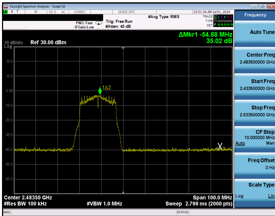
Plot 7-229. Band Edge Plot Antenna WF8 (802.11g – Ch. 13) – 24Mbps
