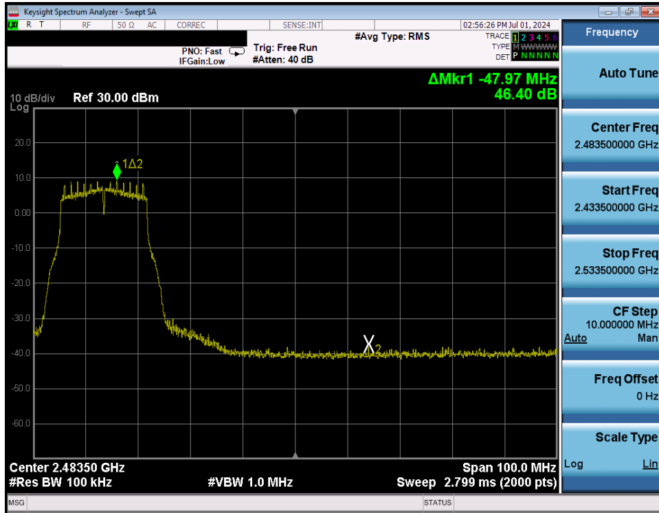
Plot 7-310. Band Edge Plot Antenna WF7 (802.11g – Ch. 8) – 12Mbps
