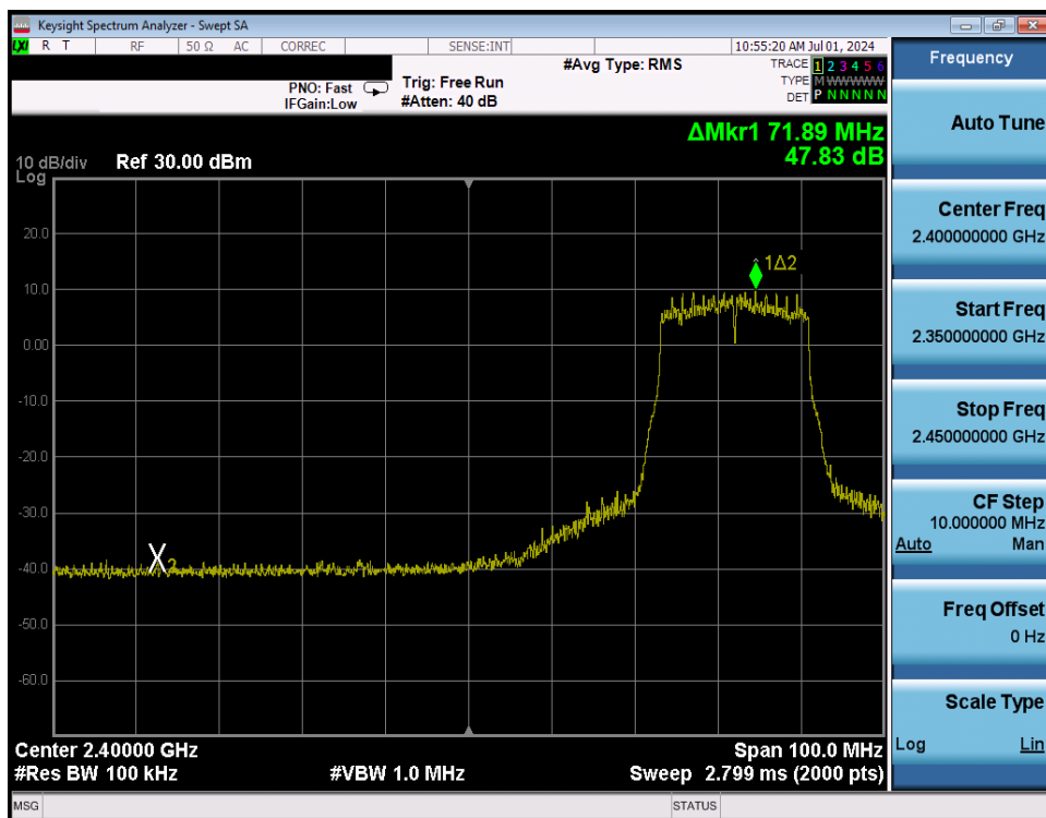
Plot 7-234. Band Edge Plot Antenna WF8 (802.11n (2.4GHz) – Ch. 5) – MCS4
