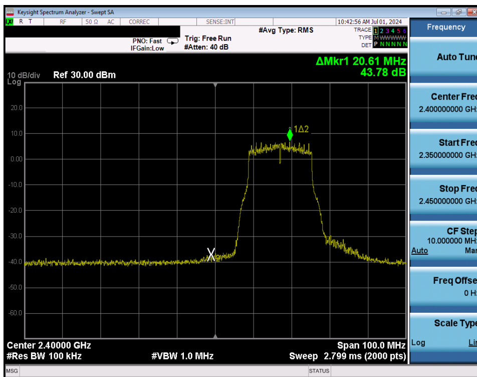
Plot 7-217. Band Edge Plot Antenna WF8 (802.11g – Ch. 2) – 24Mbps
