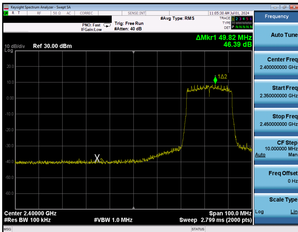
Plot 7-248. Band Edge Plot Antenna WF8 (802.11ax (SU - 2.4GHz) – Ch. 5) – MCS4
