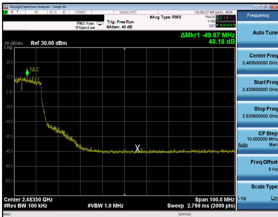
Plot 7-236. Band Edge Plot Antenna WF8 (802.11n (2.4GHz) - Ch. 6 High) - MCS4
