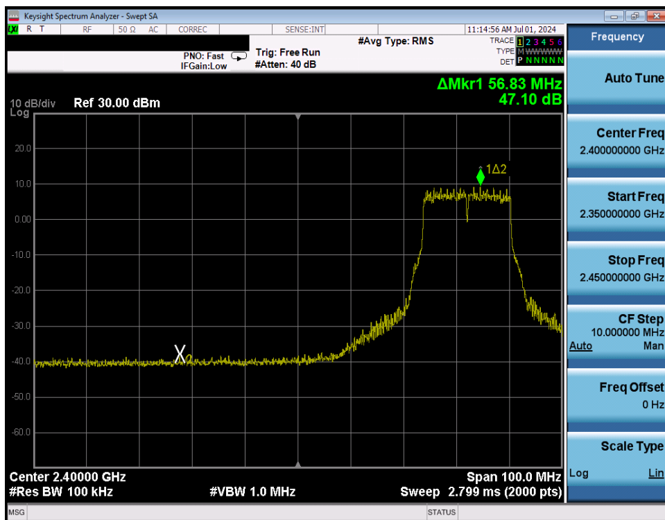
Plot 7-265. Band Edge Plot Antenna WF8 (802.11g – Ch. 5) – 54Mbps
