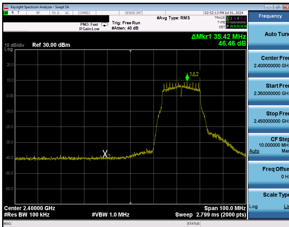
Plot 7-304. Band Edge Plot Antenna WF7 (802.11g – Ch. 3) – 12Mbps
