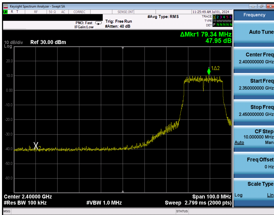
Plot 7-280. Band Edge Plot Antenna WF8 (802.11n (2.4GHz) – Ch. 6 Low) – MCS7
