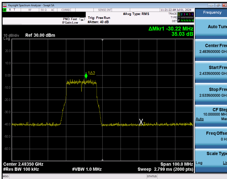
Plot 7-274. Band Edge Plot Antenna WF8 (802.11g – Ch. 13) – 54Mbps
