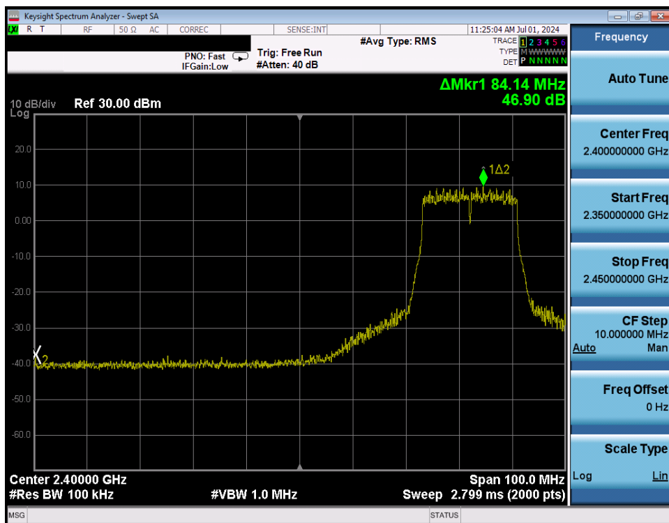
Plot 7-279. Band Edge Plot Antenna WF8 (802.11n (2.4GHz) – Ch. 5) – MCS7
