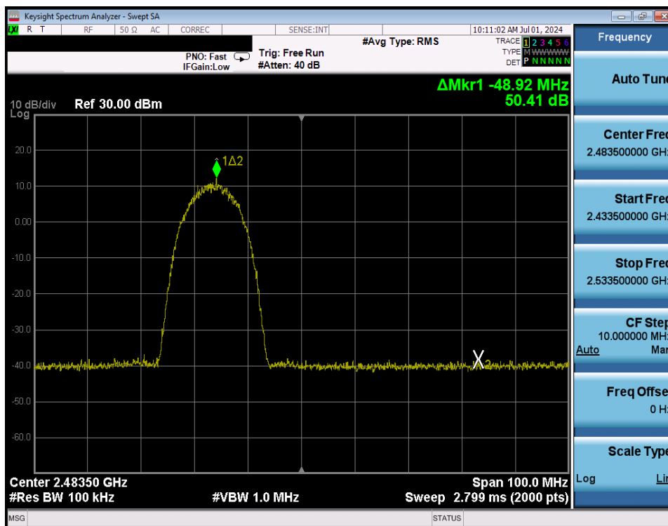
Plot 7-259. Band Edge Plot Antenna WF8 (802.11b – Ch. 12) – 11Mbps
