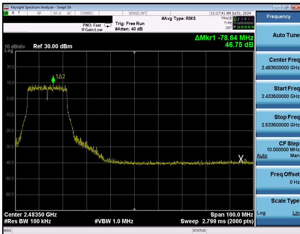
Plot 7-269. Band Edge Plot Antenna WF8 (802.11g - Ch. 8) - 54Mbps
