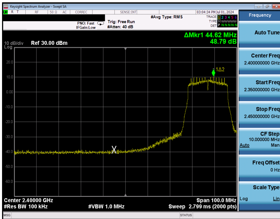
Plot 7-321. Band Edge Plot Antenna WF7 (802.11n (2.4GHz) – Ch. 6 Low) – MCS2
