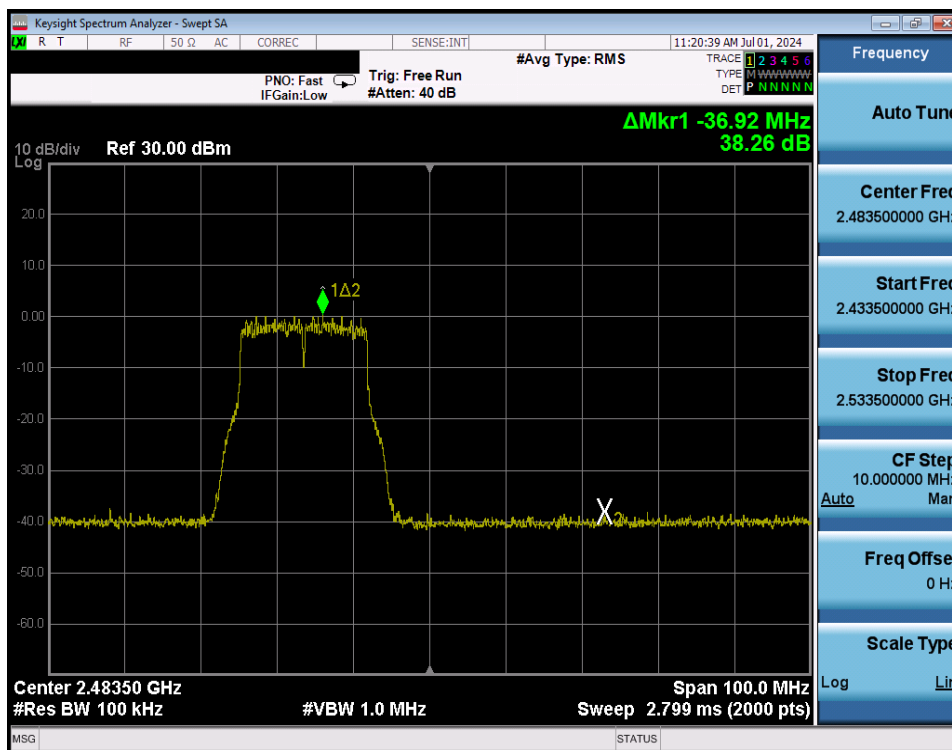
Plot 7-273. Band Edge Plot Antenna WF8 (802.11g – Ch. 12) – 54Mbps
