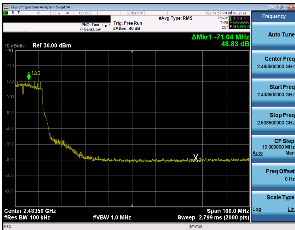
Plot 7-308. Band Edge Plot Antenna WF7 (802.11g – Ch. 6 High) – 12Mbps
