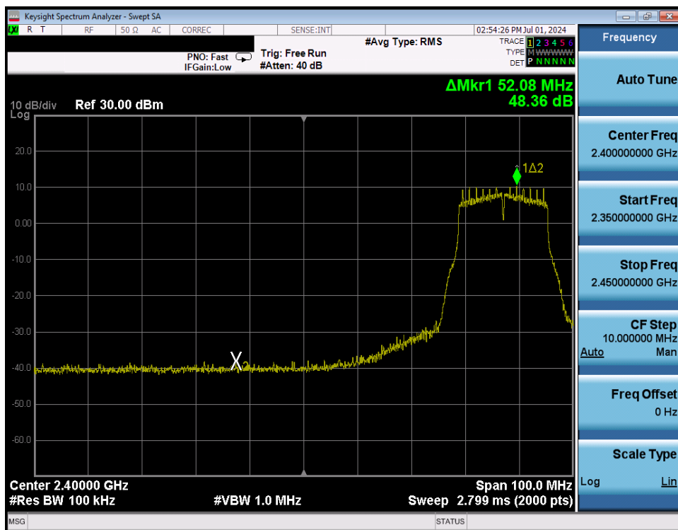
Plot 7-307. Band Edge Plot Antenna WF7 (802.11g – Ch. 6 Low) – 12Mbps
