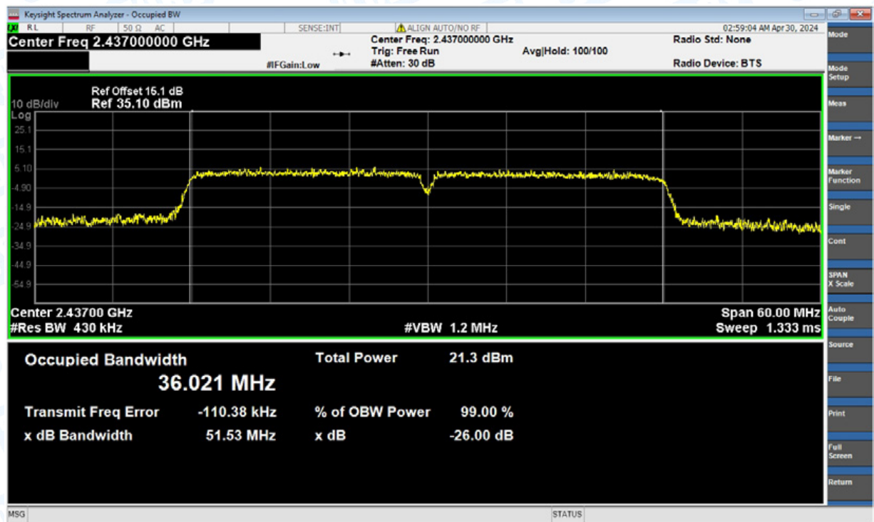
OBW NVNT n(HT40) 2437MHz Ant2
